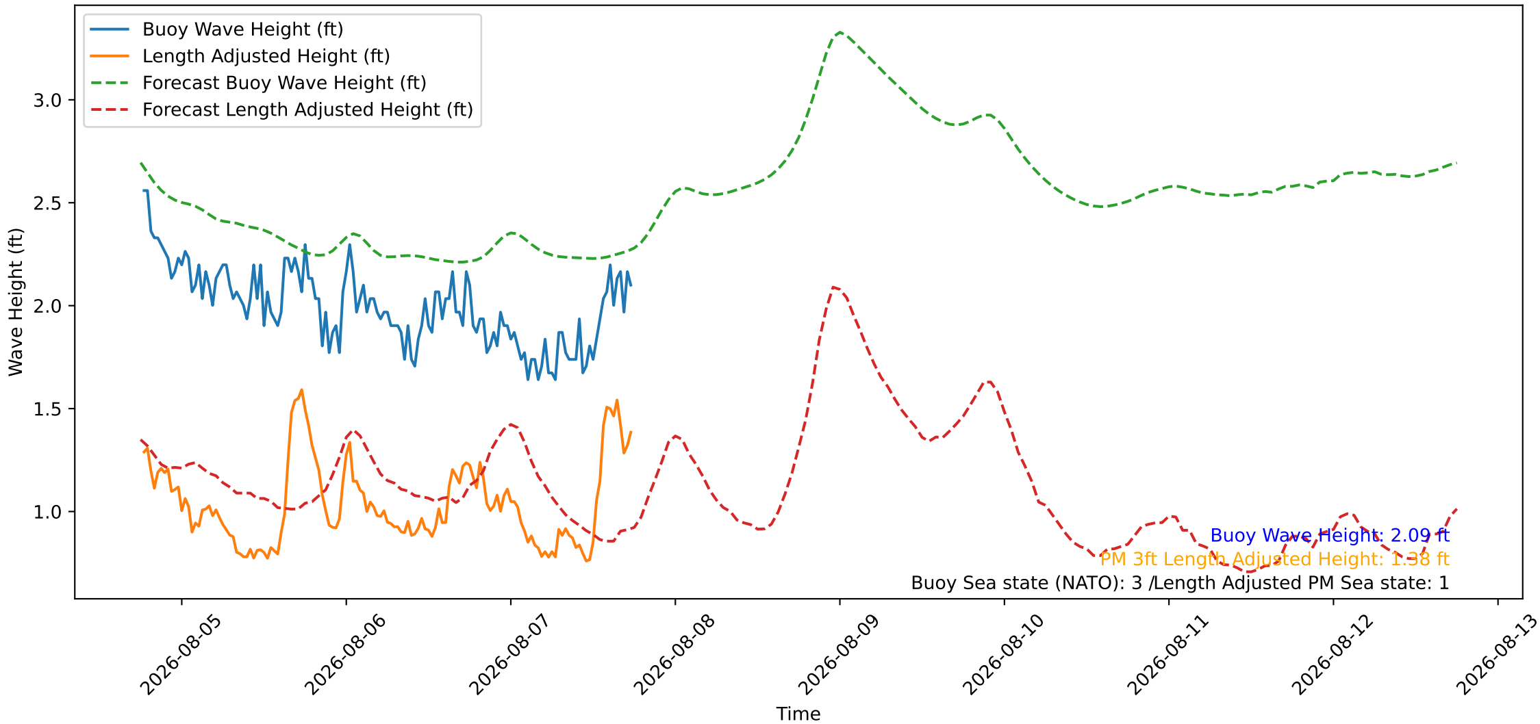
Wave Heights over Time for Oceanside Harbor at 2026-08-07 18:20:26
