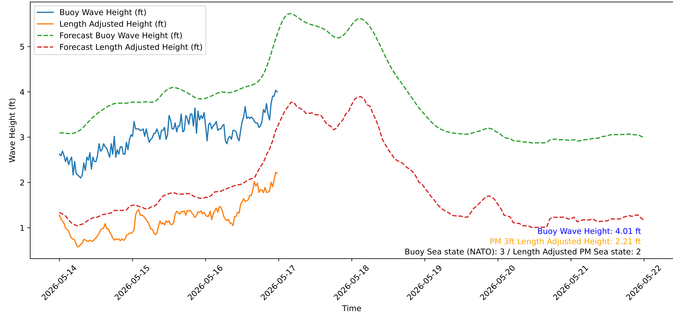
Wave Heights over Time for Green Beach at 2026-05-17 00:11:12
