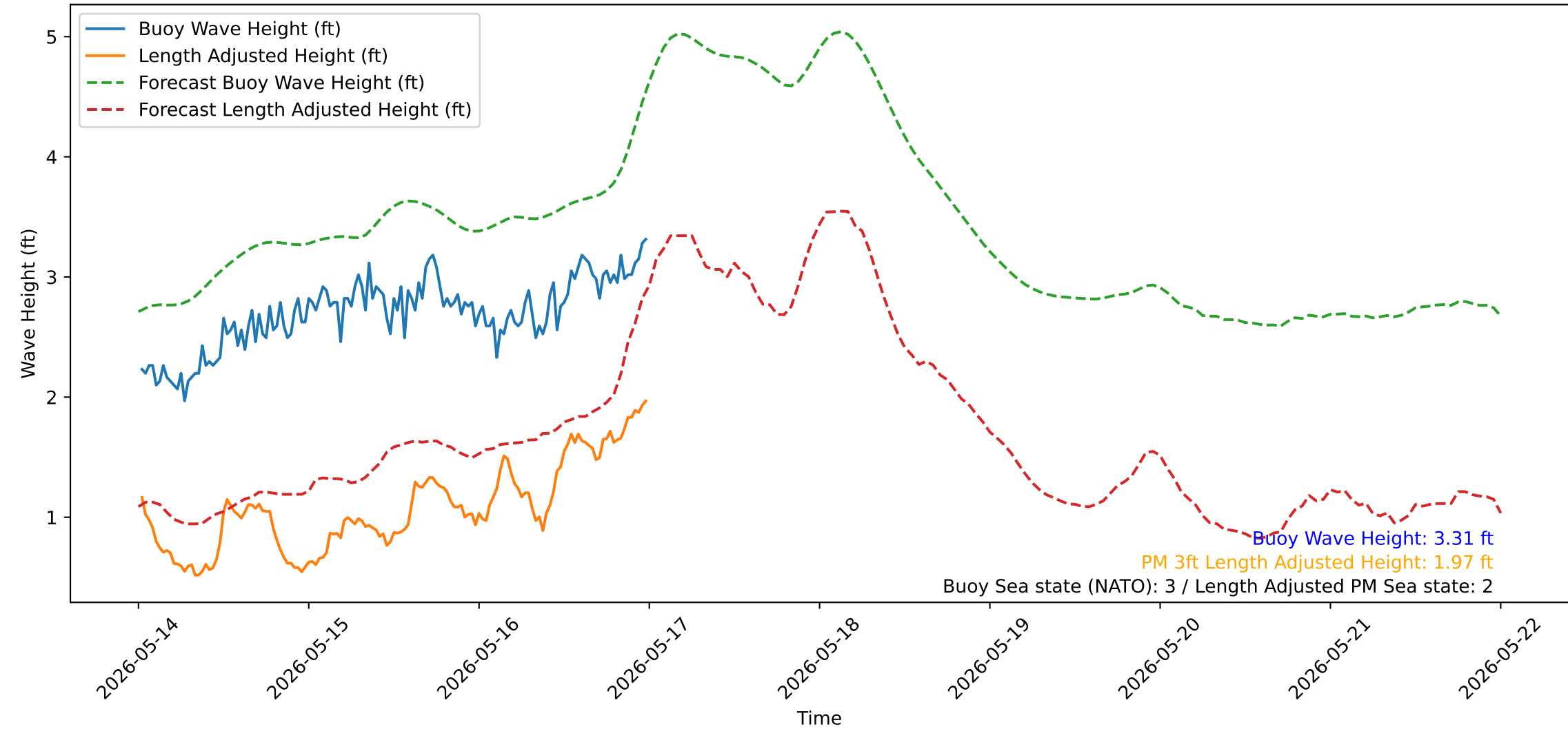
Wave Heights over Time for Red Beach at 2026-05-17 00:10:50
