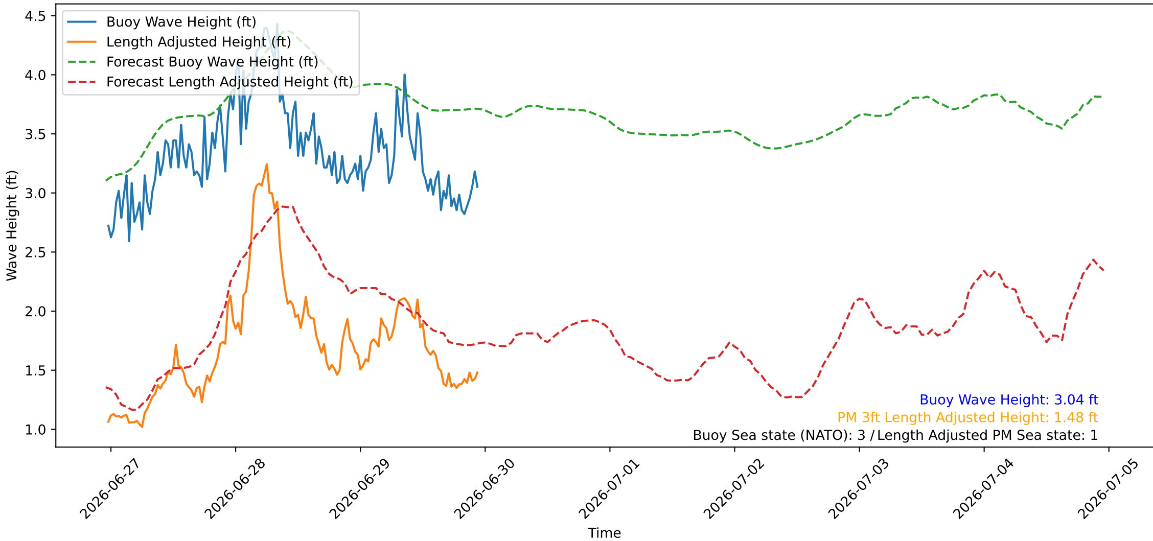
Wave Heights over Time for Oceanside Harbor at 2026-06-29 23:20:25
