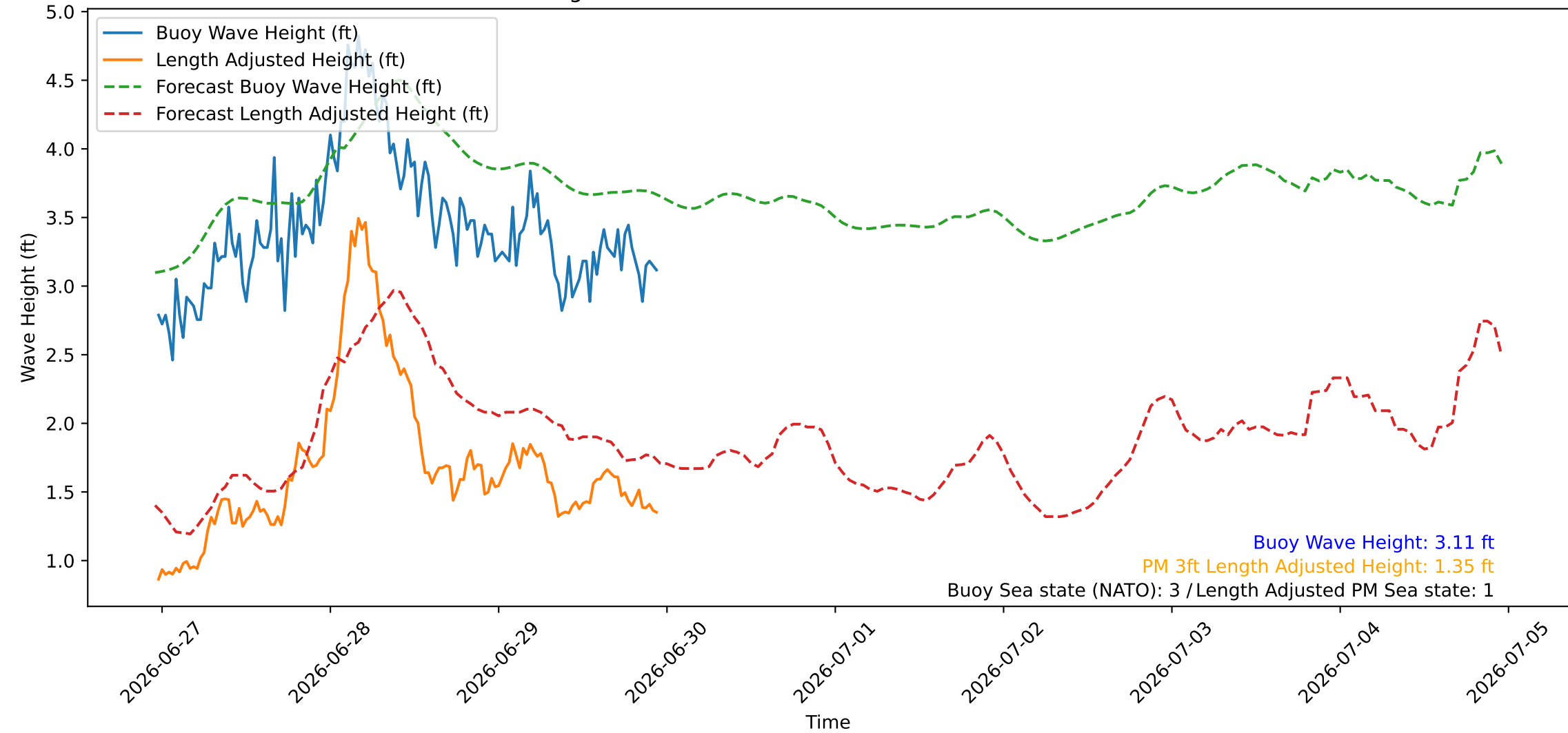
Wave Heights over Time for Green Beach at 2026-06-29 23:21:08
