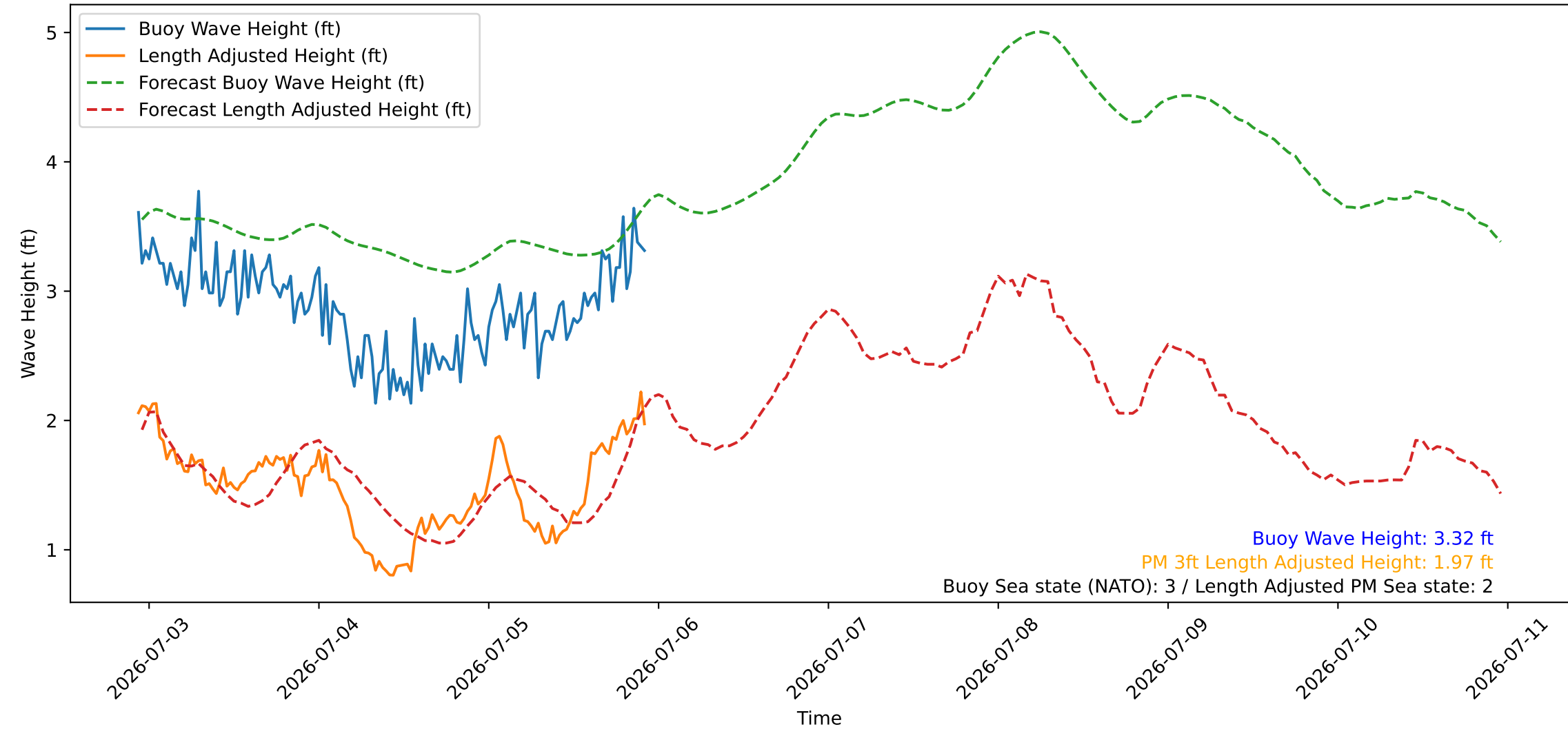
Wave Heights over Time for Oceanside Harbor at 2026-07-05 22:40:26
