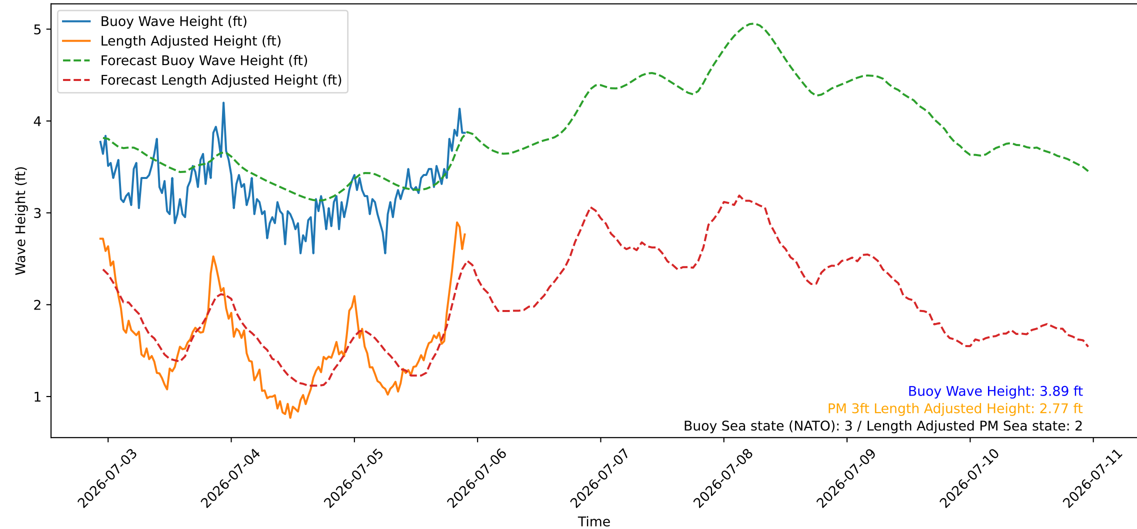
Wave Heights over Time for Green Beach at 2026-07-05 22:41:08
