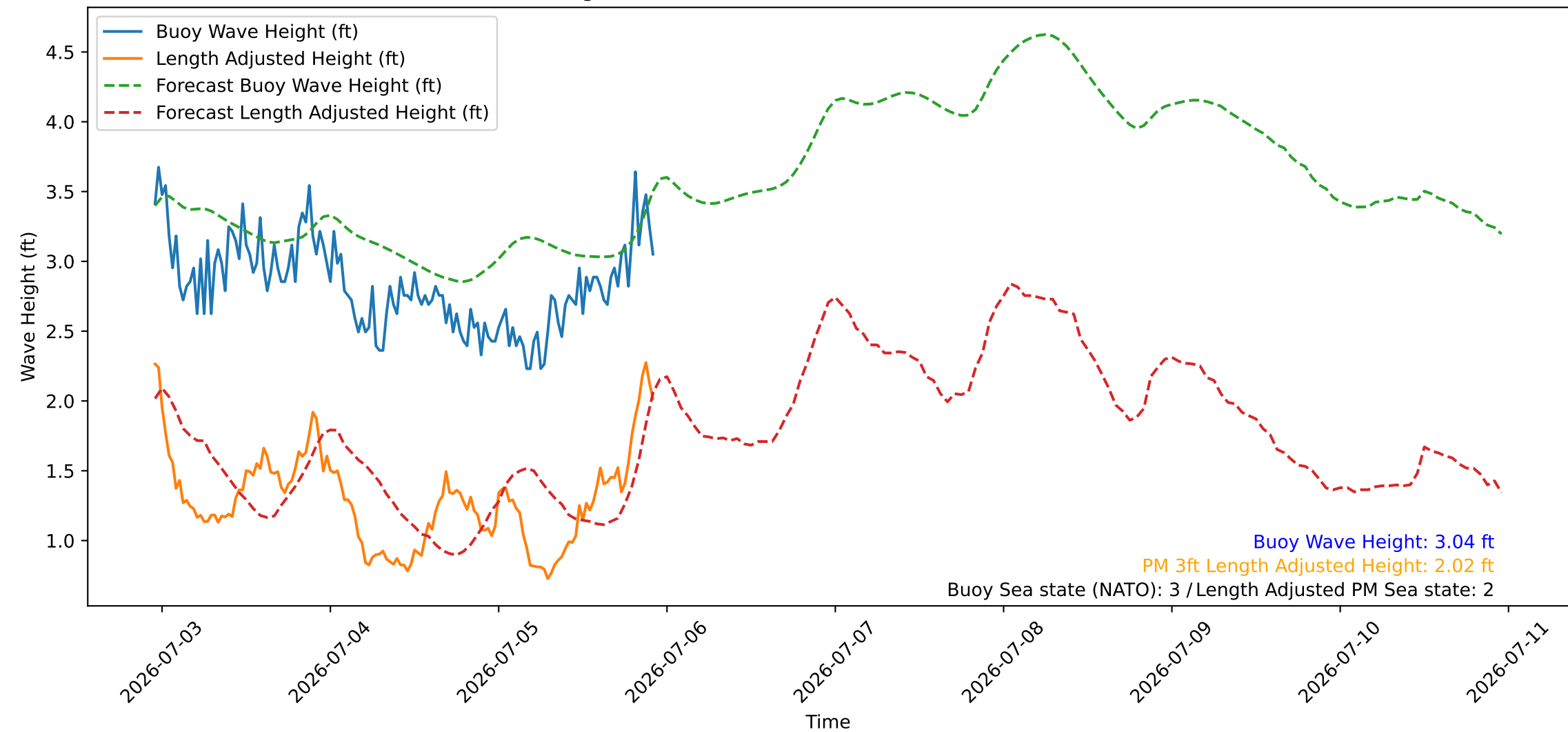
Wave Heights over Time for Red Beach at 2026-07-05 22:40:46
