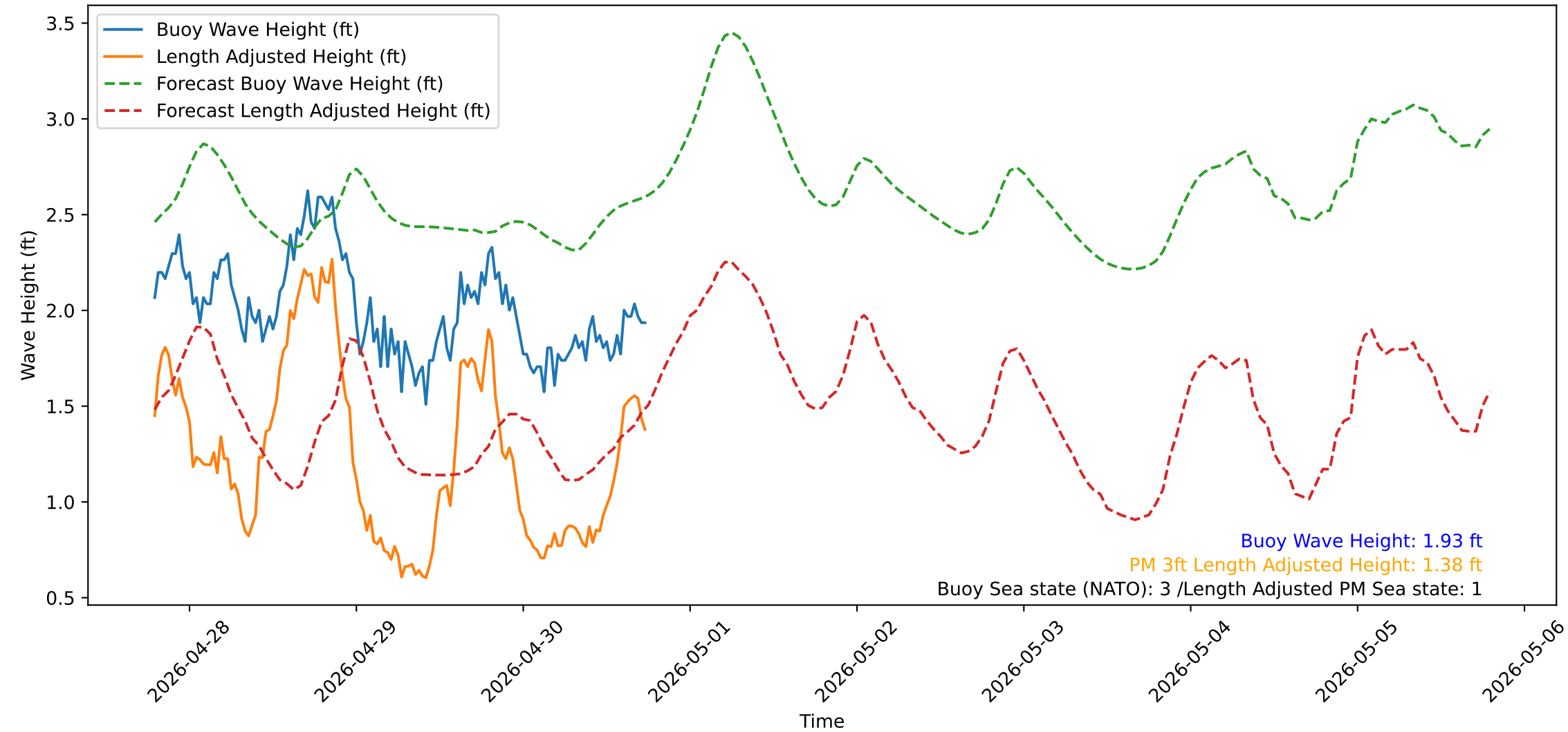
Wave Heights over Time for Red Beach at 2026-04-30 18:30:51
