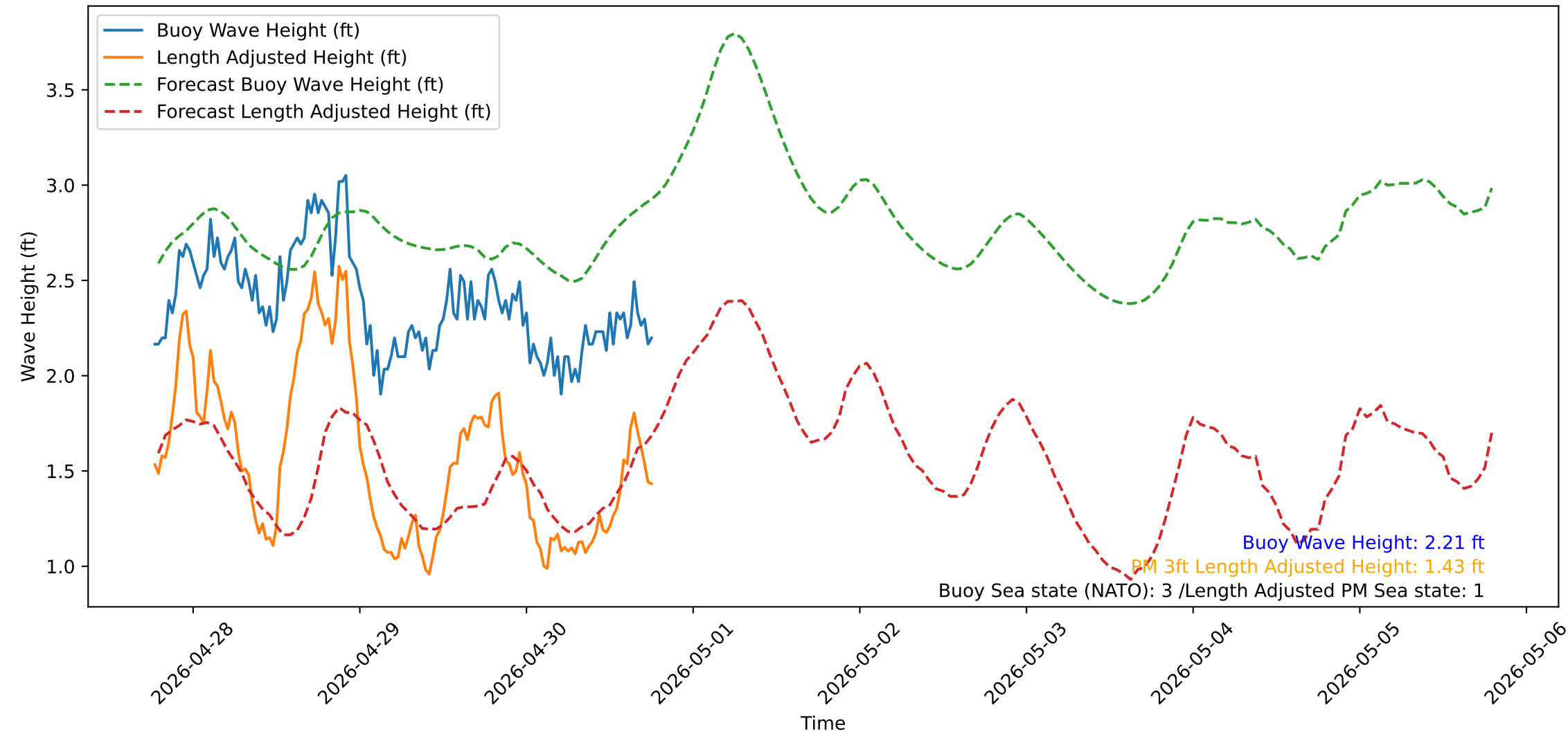
Wave Heights over Time for Oceanside Harbor at 2026-04-30 18:30:31
