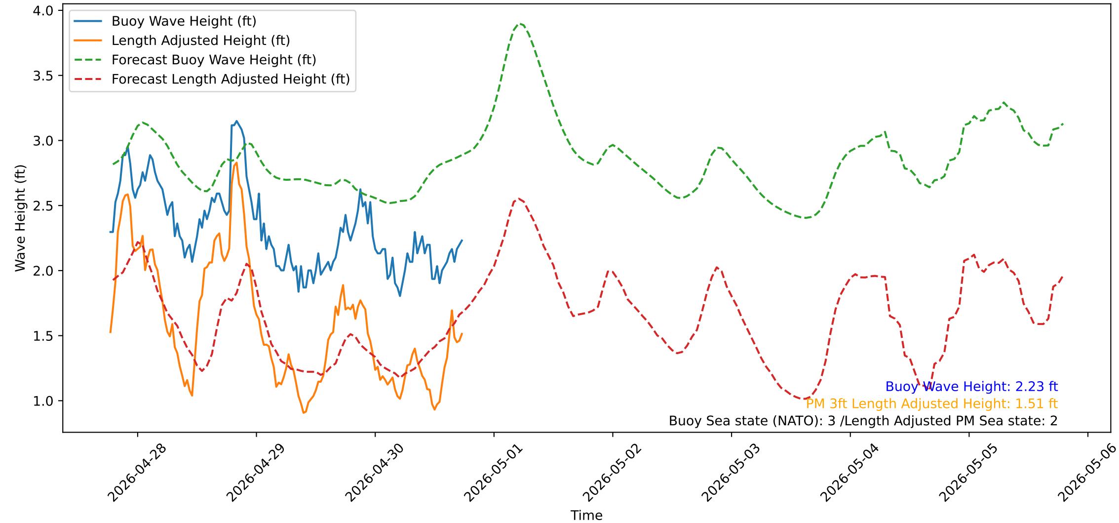
Wave Heights over Time for Green Beach at 2026-04-30 18:31:13
