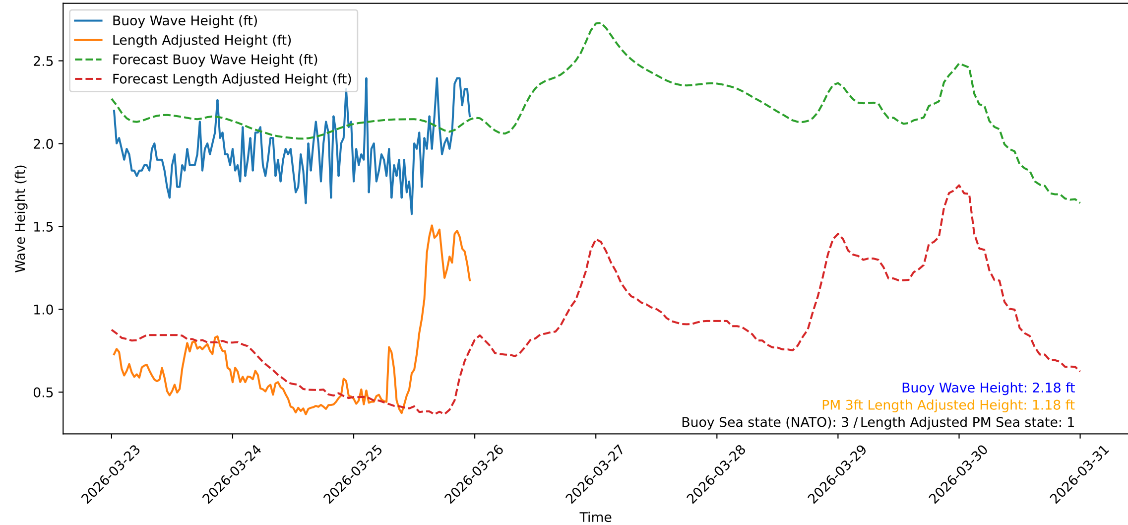
Wave Heights over Time for Red Beach at 2026-03-26 00:00:47
