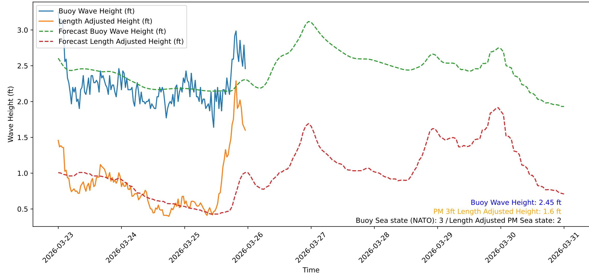
Wave Heights over Time for Green Beach at 2026-03-26 00:01:09
