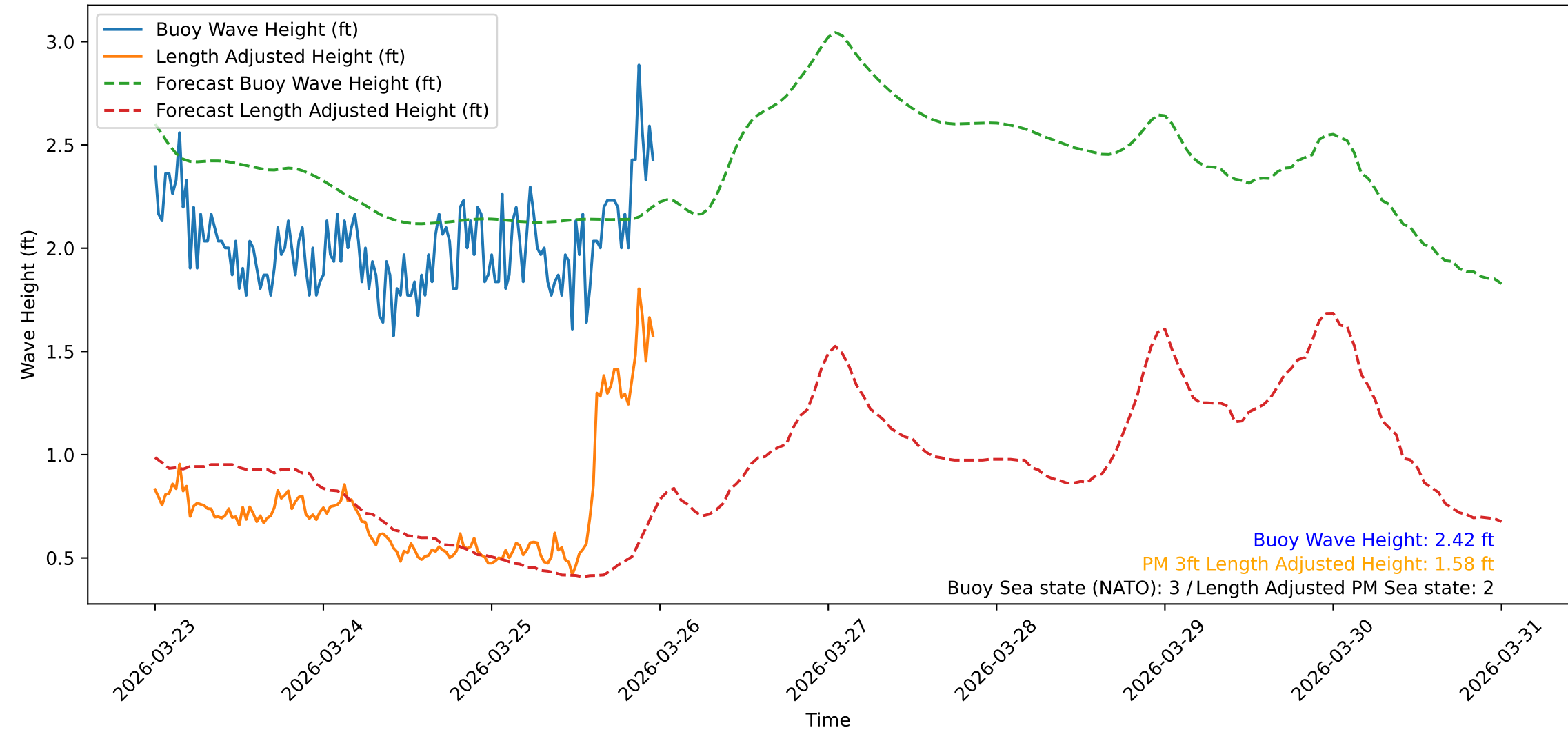
Wave Heights over Time for Oceanside Harbor at 2026-03-26 00:00:31
