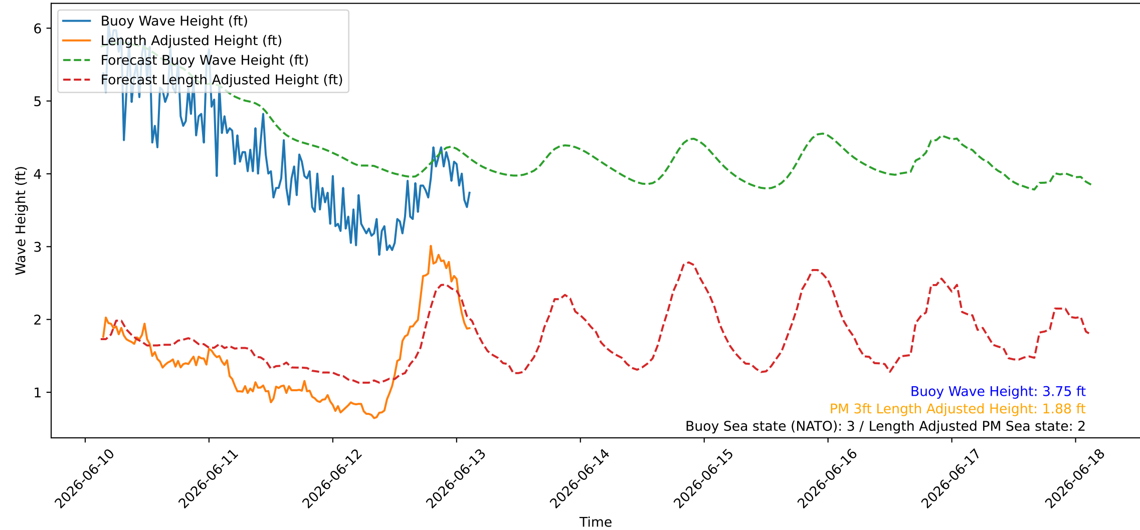
Wave Heights over Time for Green Beach at 2026-06-13 03:21:08
