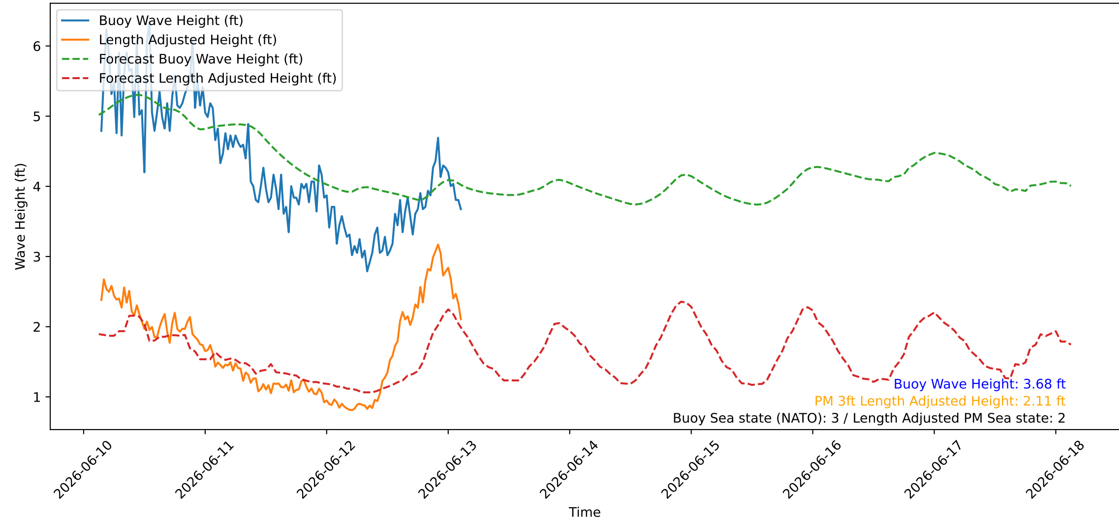
Wave Heights over Time for Oceanside Harbor at 2026-06-13 03:20:25
