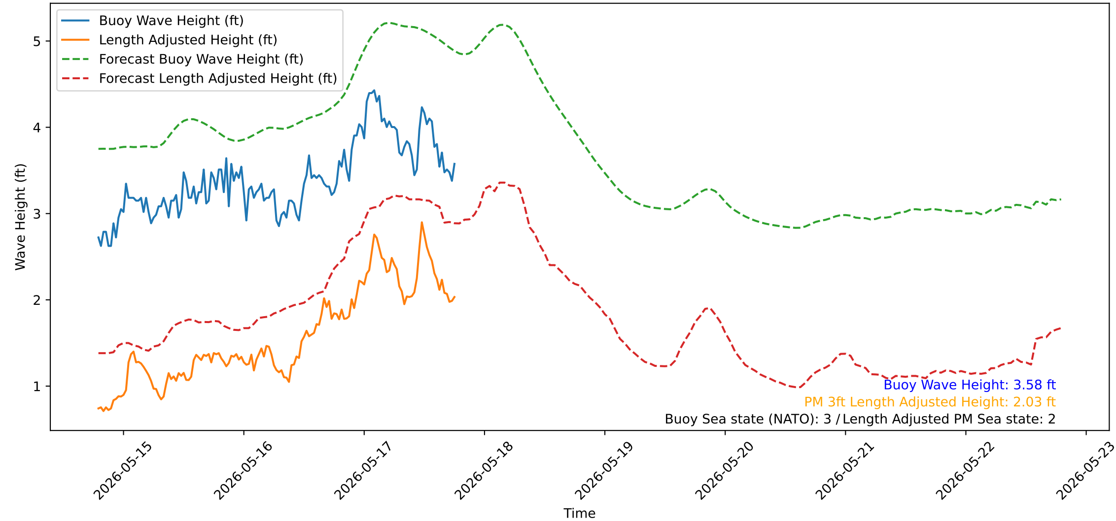
Wave Heights over Time for Green Beach at 2026-05-17 18:51:15
