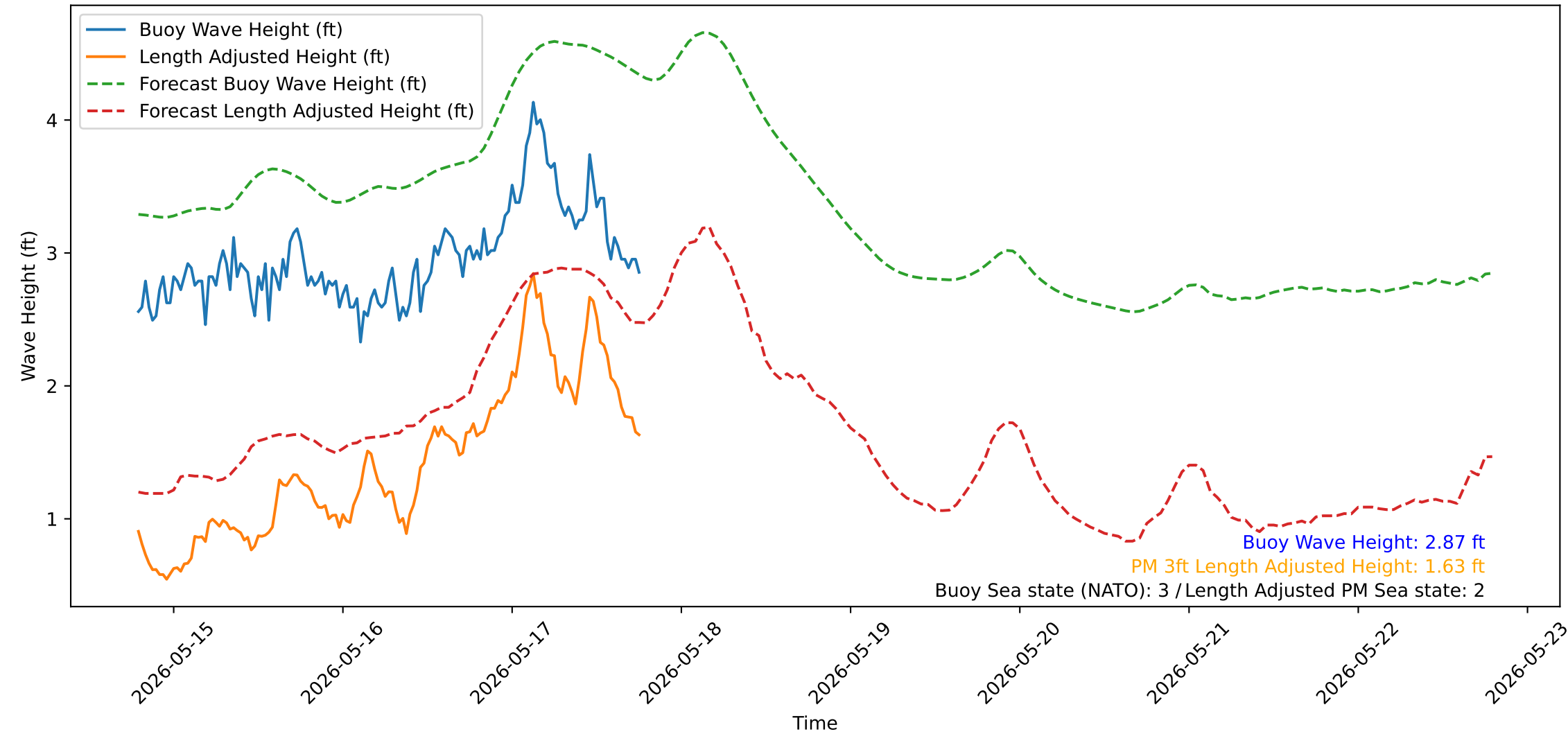
Wave Heights over Time for Red Beach at 2026-05-17 18:50:52
