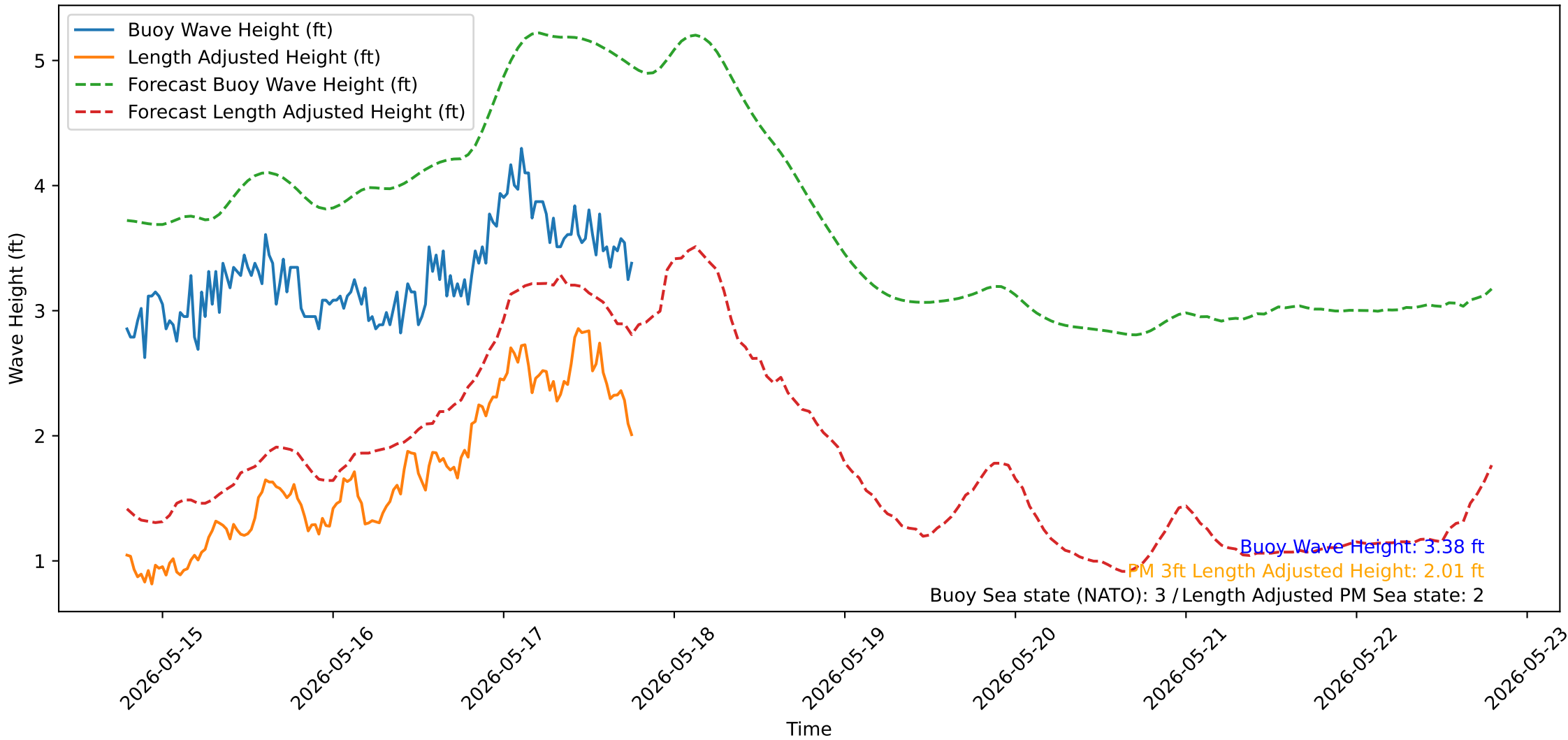
Wave Heights over Time for Oceanside Harbor at 2026-05-17 18:50:32
