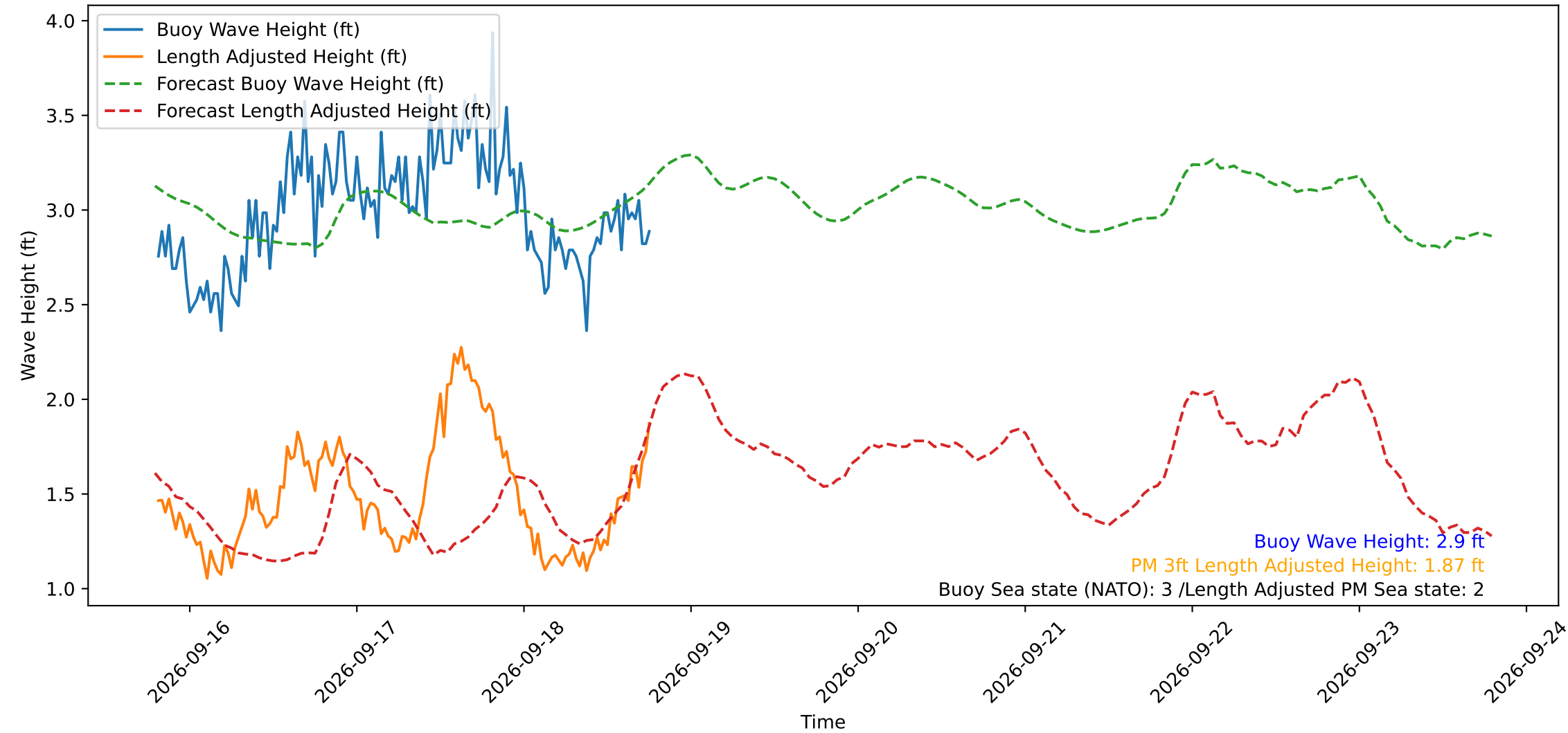
Wave Heights over Time for Oceanside Harbor at 2026-09-18 19:20:30
