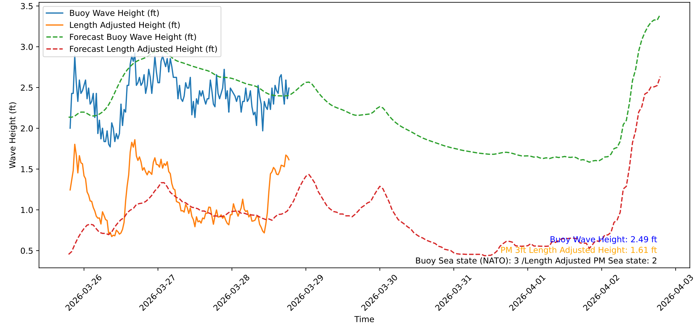
Wave Heights over Time for Oceanside Harbor at 2026-03-28 19:20:31
