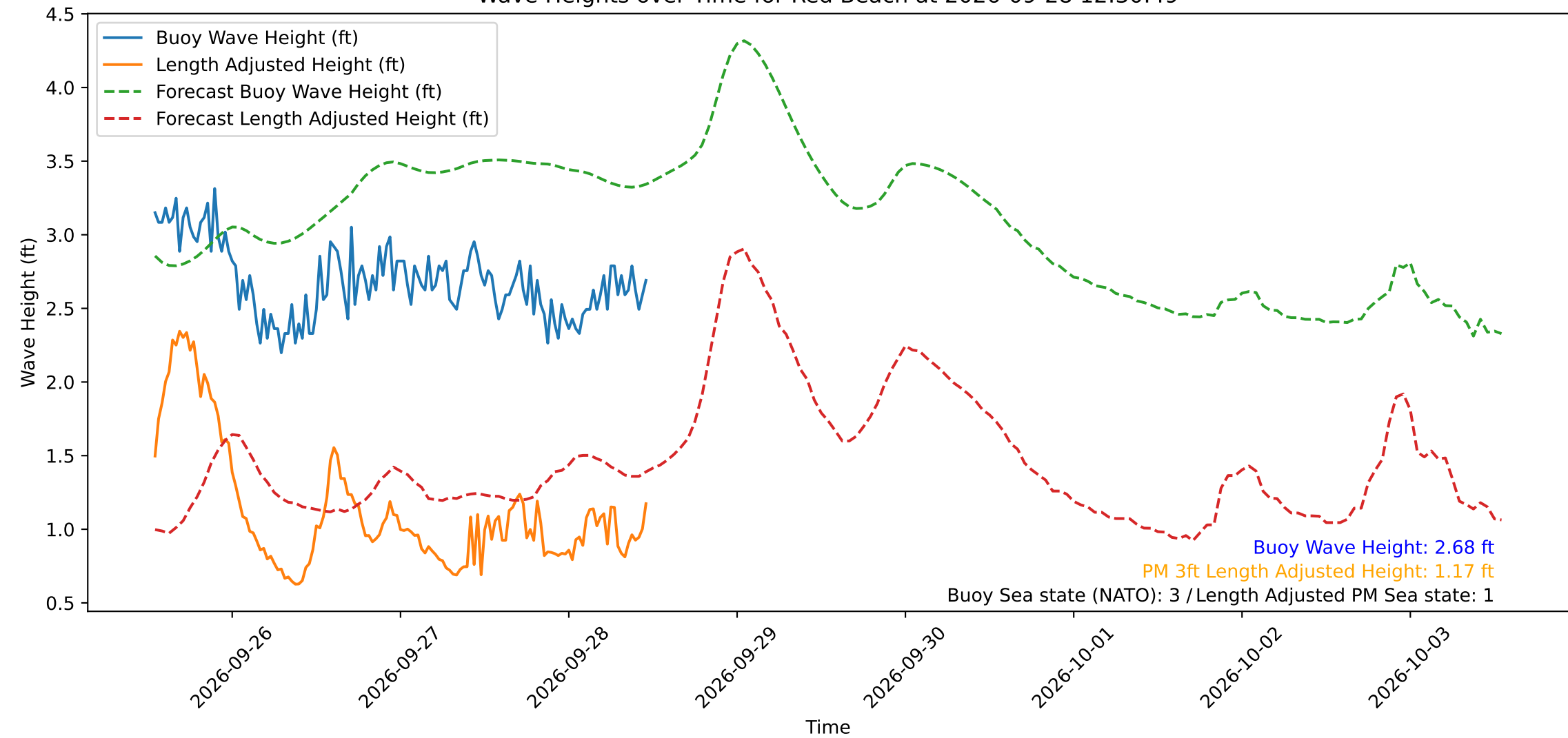
Wave Heights over Time for Red Beach at 2026-09-28 12:30:49
