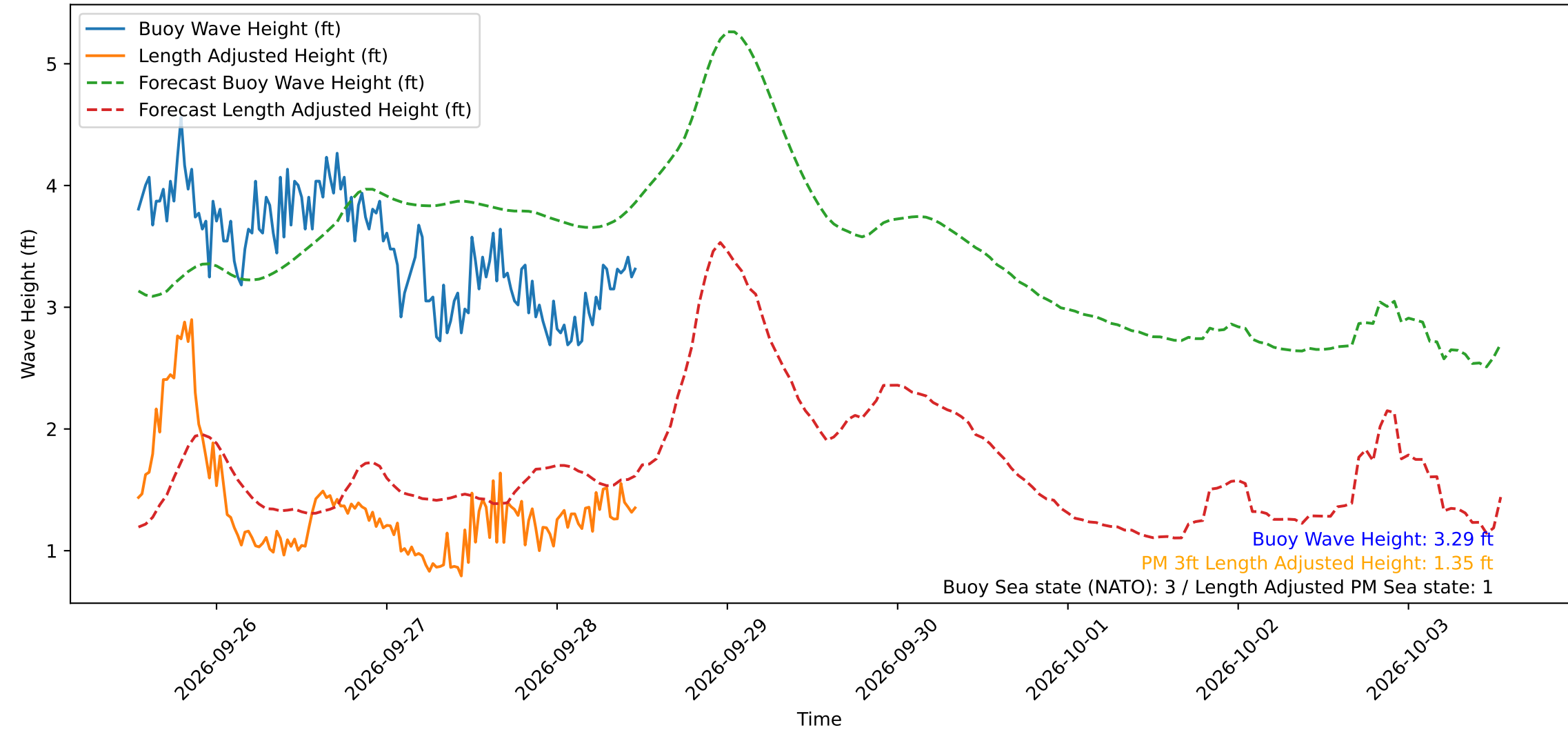
Wave Heights over Time for Green Beach at 2026-09-28 12:31:11
