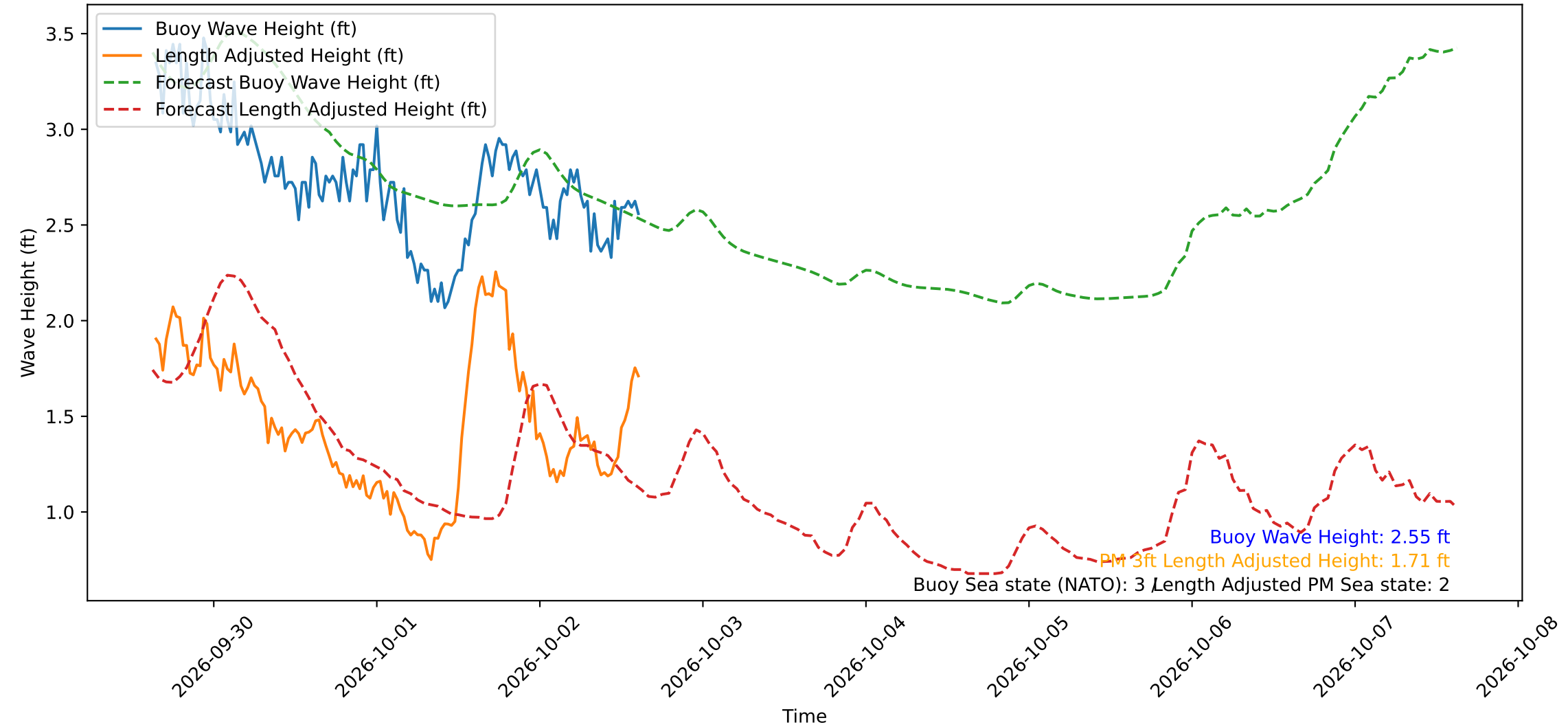
Wave Heights over Time for Red Beach at 2026-10-02 15:20:50
