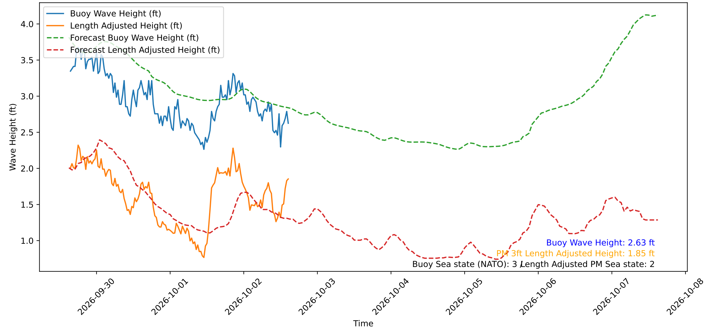
Wave Heights over Time for Oceanside Harbor at 2026-10-02 15:20:29
