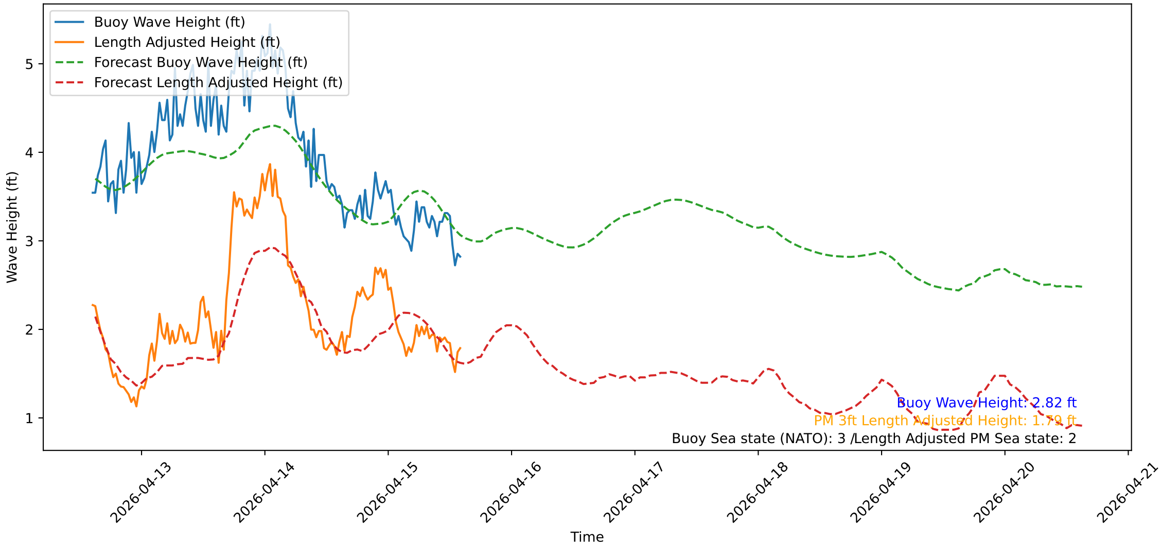
Wave Heights over Time for Oceanside Harbor at 2026-04-15 14:30:31
