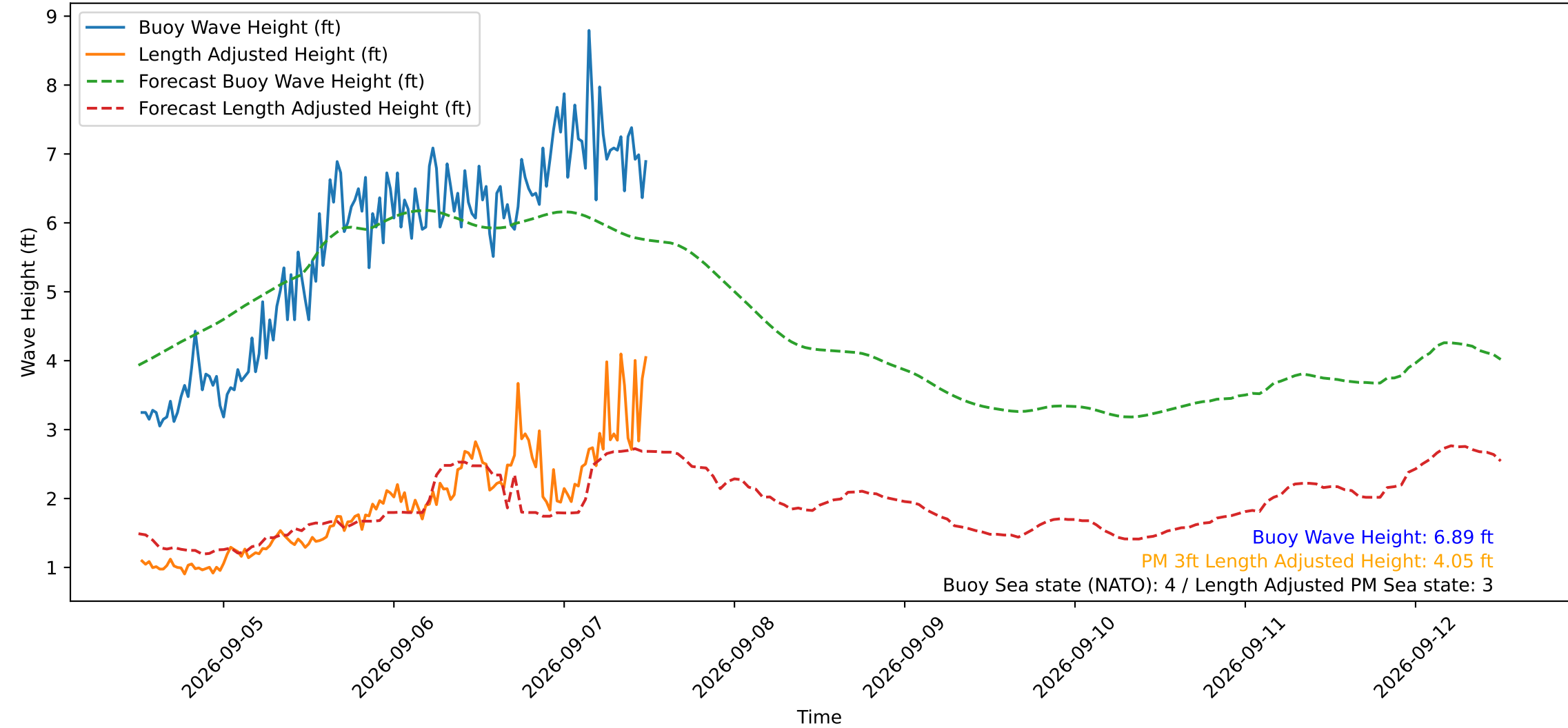
Wave Heights over Time for Green Beach at 2026-09-07 12:11:13
