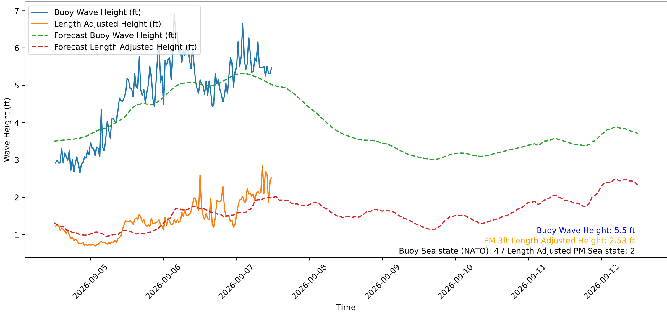
Wave Heights over Time for Red Beach at 2026-09-07 12:10:50
