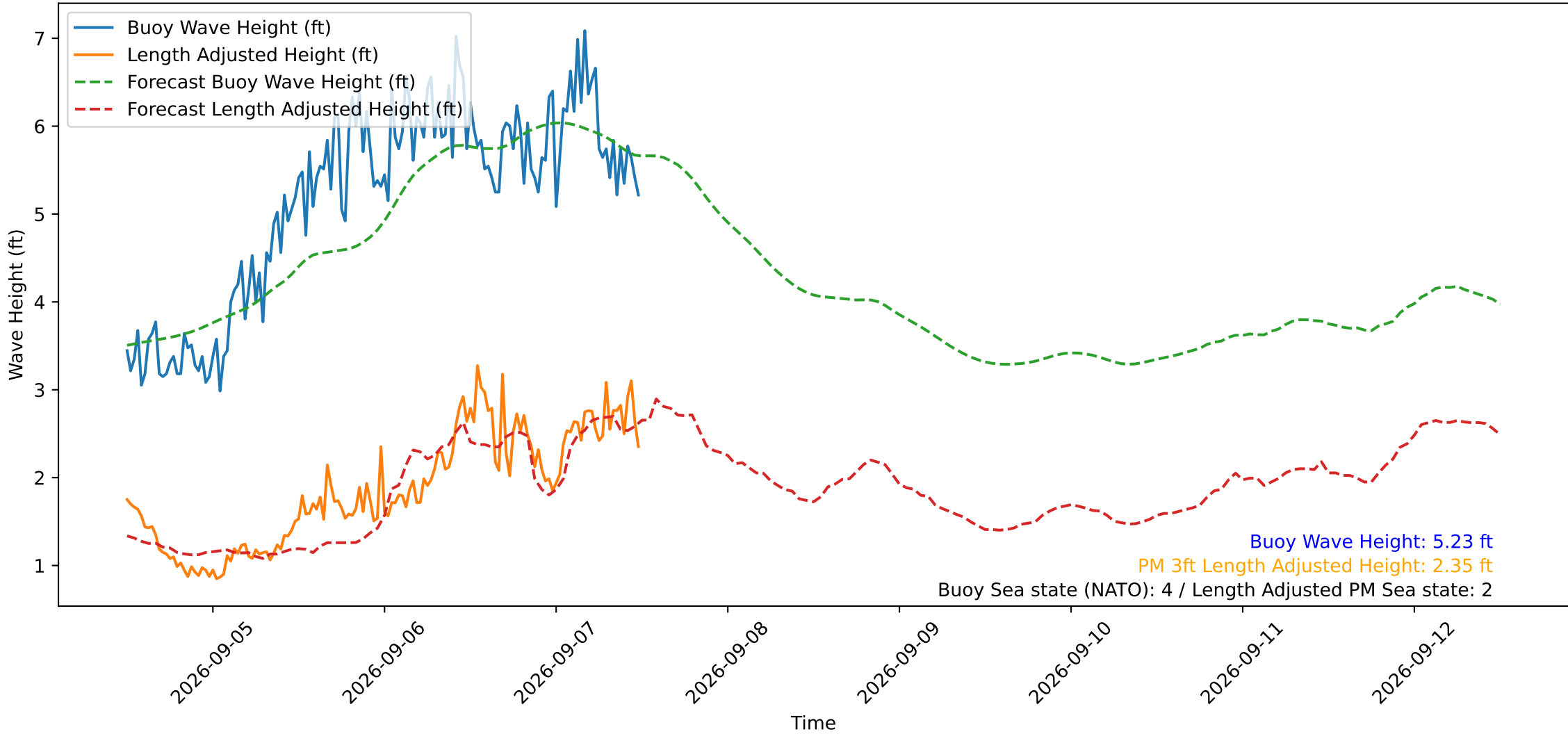
Wave Heights over Time for Oceanside Harbor at 2026-09-07 12:10:30
