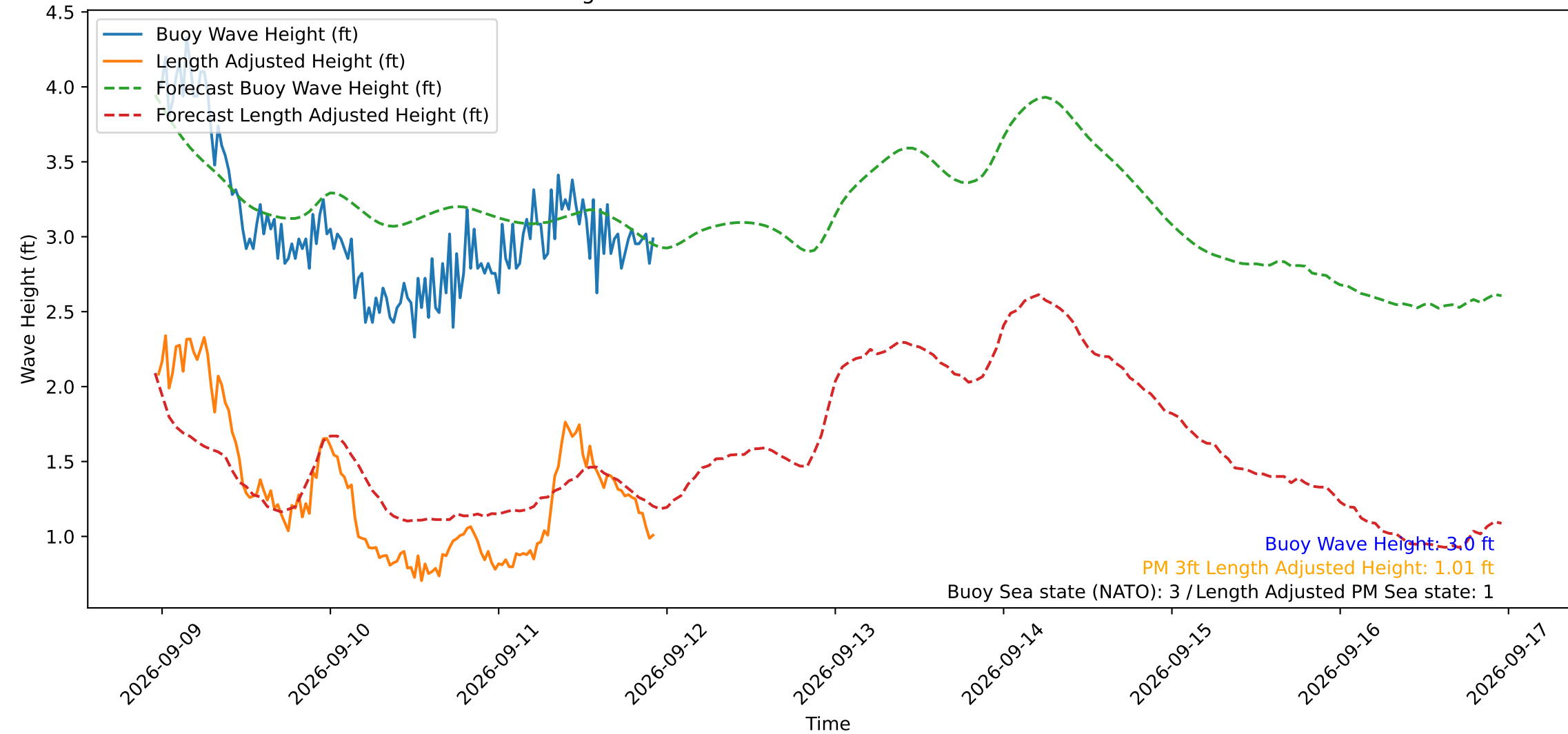
Wave Heights over Time for Red Beach at 2026-09-11 23:00:50
