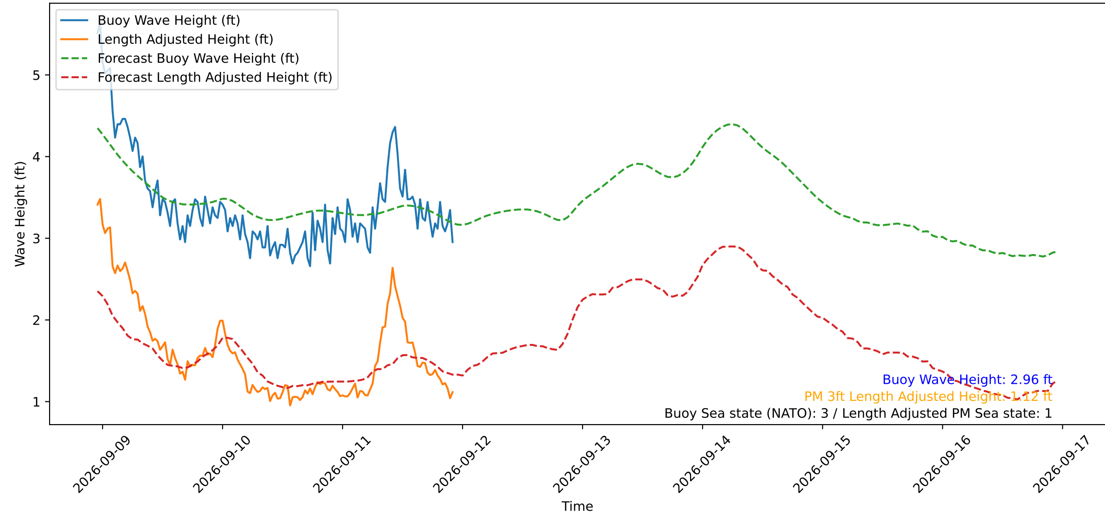
Wave Heights over Time for Oceanside Harbor at 2026-09-11 23:00:30
