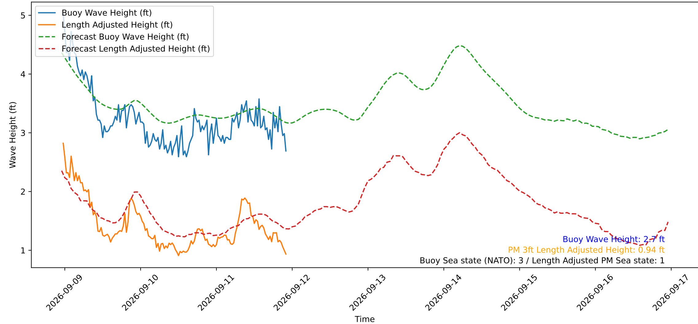
Wave Heights over Time for Green Beach at 2026-09-11 23:01:14
