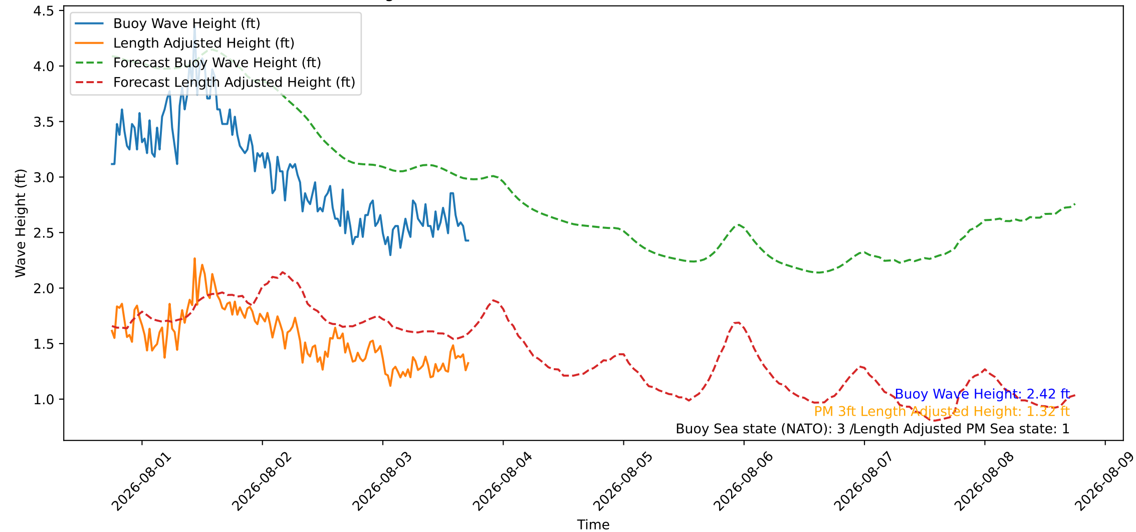
Wave Heights over Time for Oceanside Harbor at 2026-08-03 17:50:26
