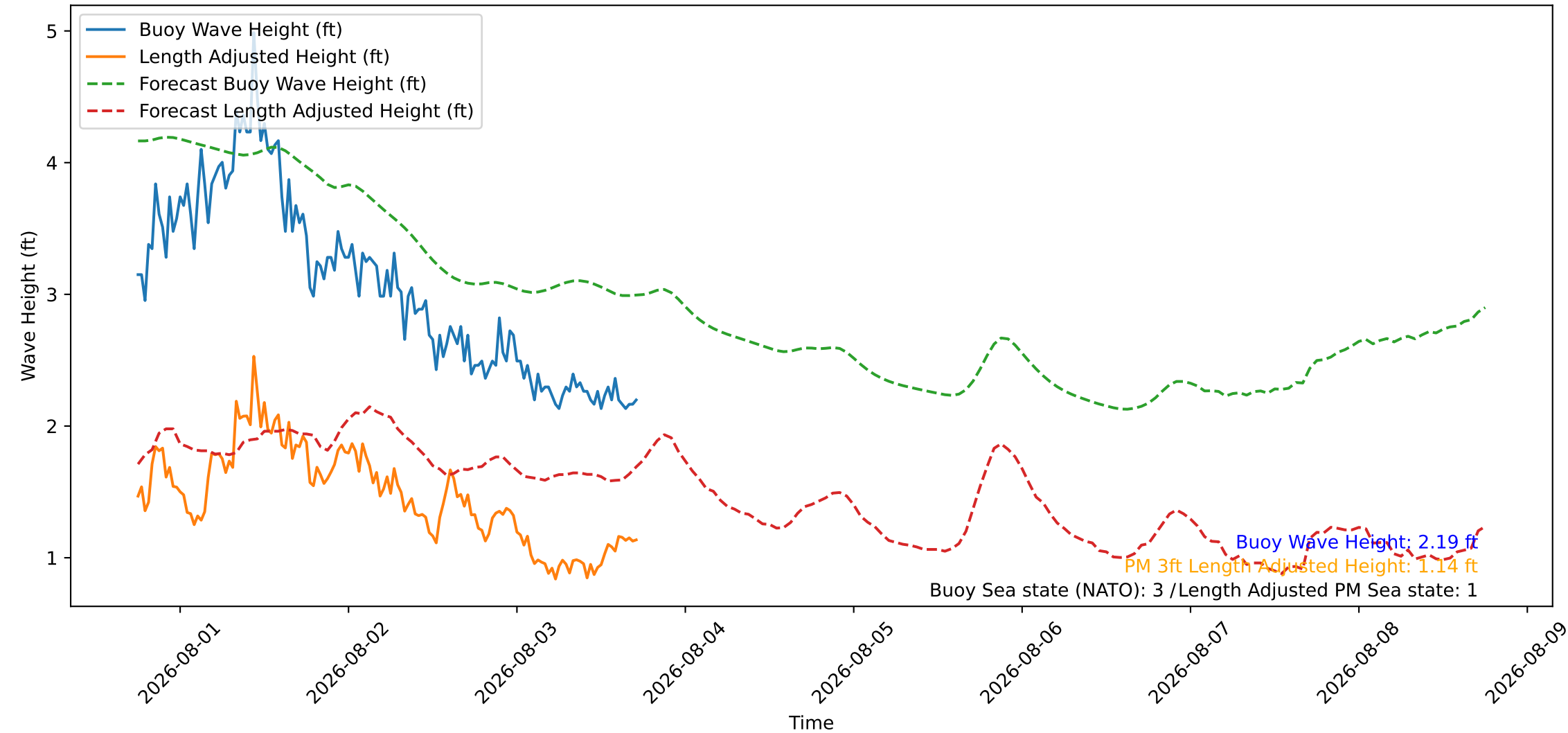
Wave Heights over Time for Green Beach at 2026-08-03 17:51:09
