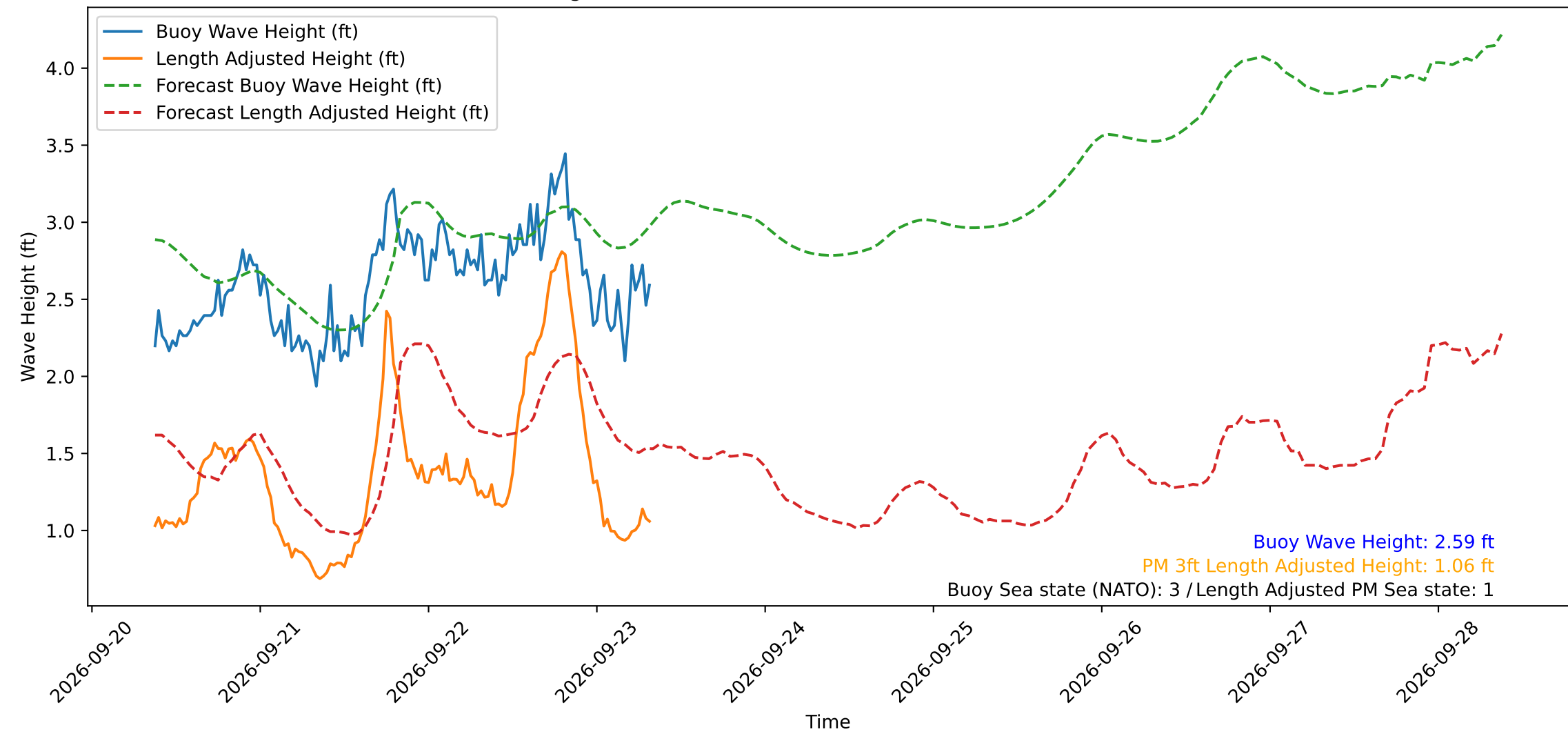
Wave Heights over Time for Green Beach at 2026-09-23 08:31:11
