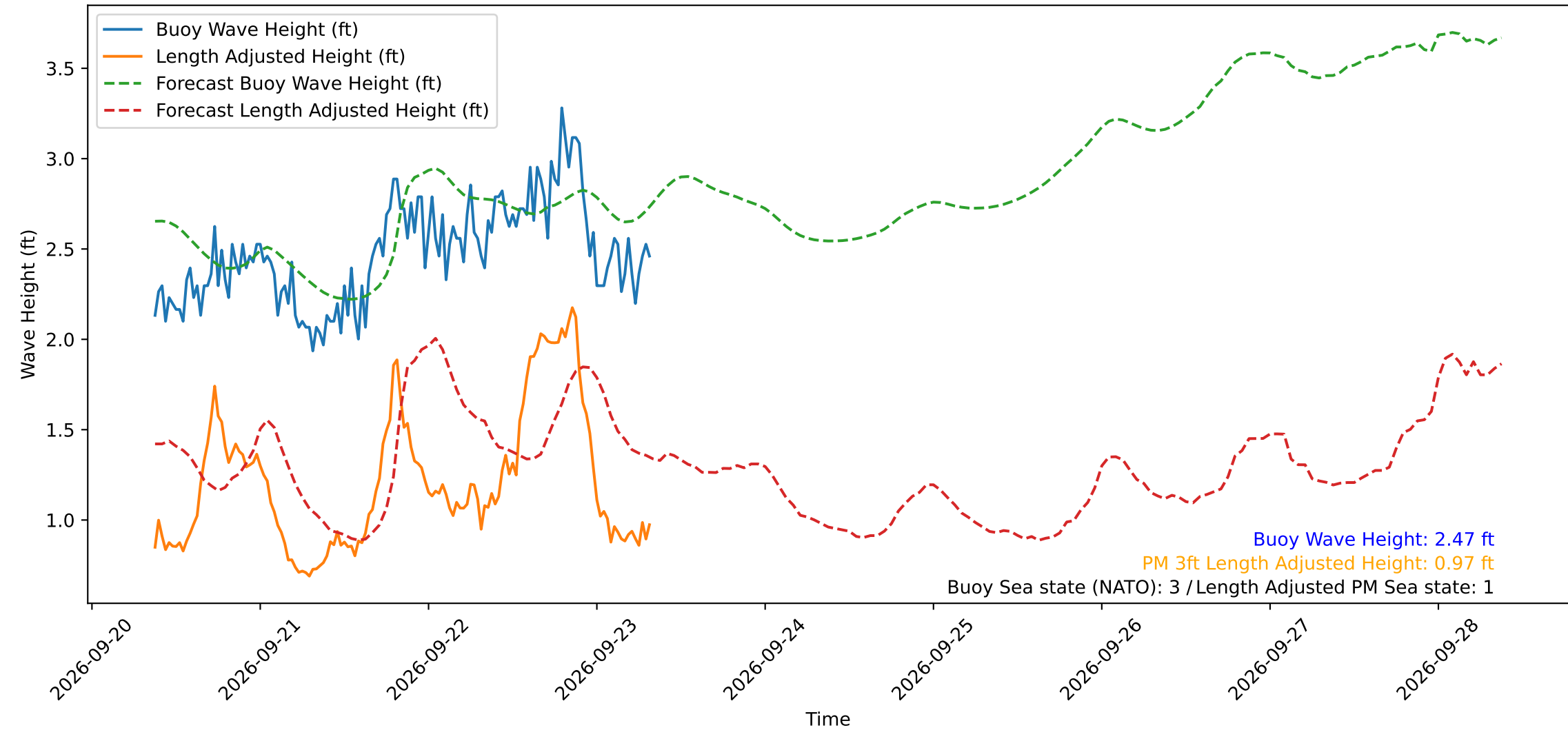
Wave Heights over Time for Red Beach at 2026-09-23 08:30:49
