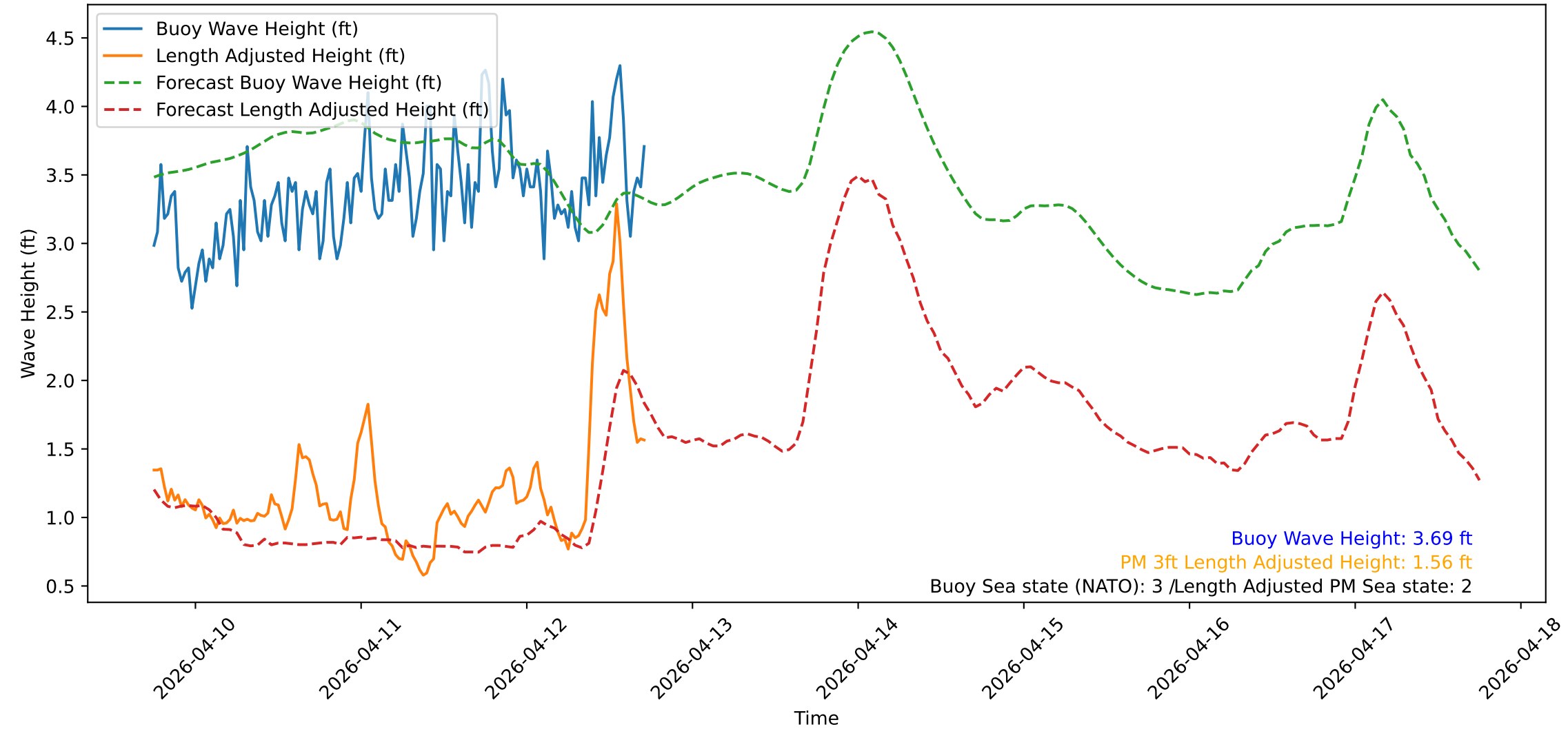
Wave Heights over Time for Red Beach at 2026-04-12 17:40:51
