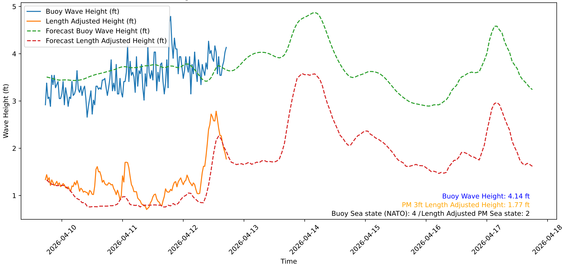
Wave Heights over Time for Oceanside Harbor at 2026-04-12 17:40:31
