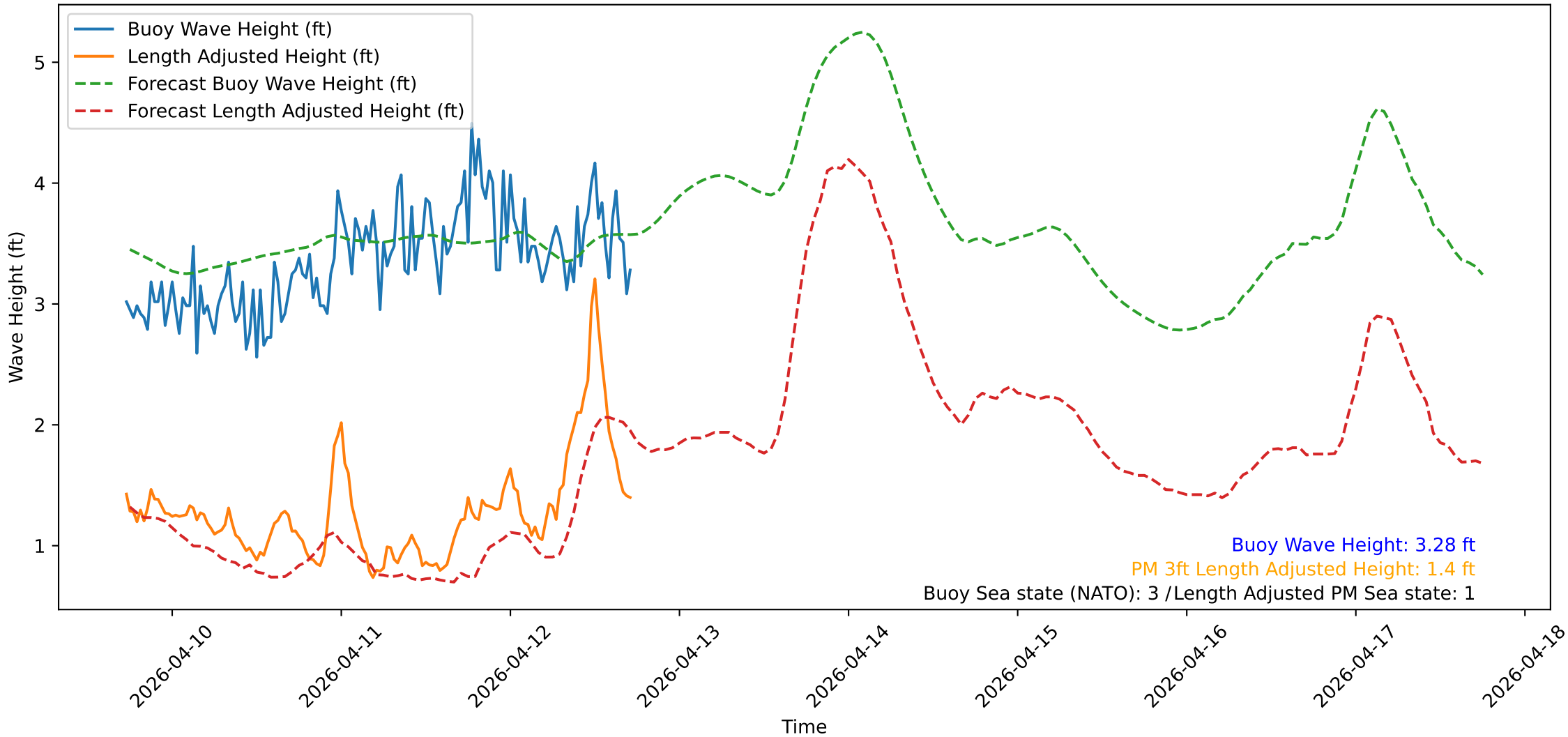
Wave Heights over Time for Green Beach at 2026-04-12 17:41:13
