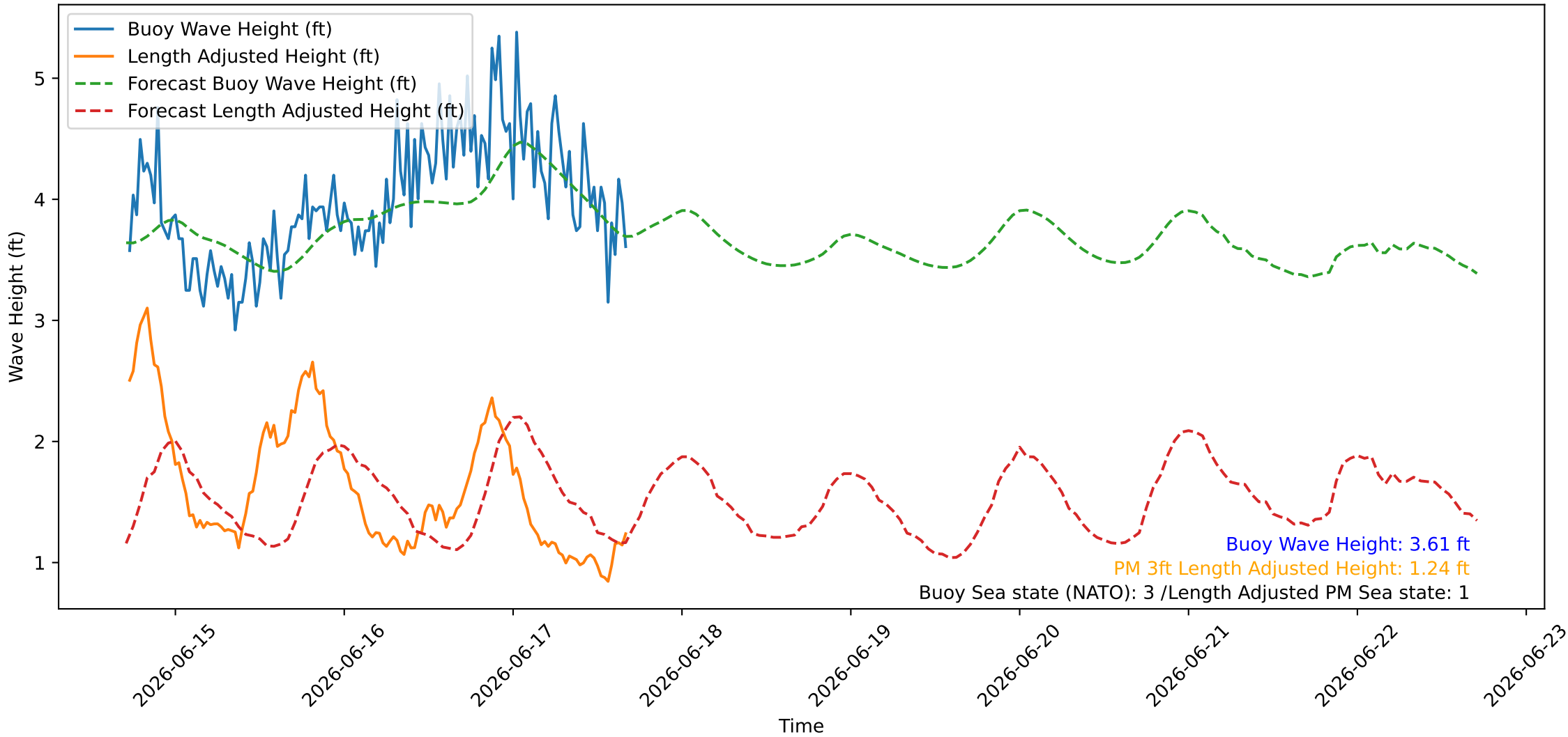
Wave Heights over Time for Red Beach at 2026-06-17 17:00:46
