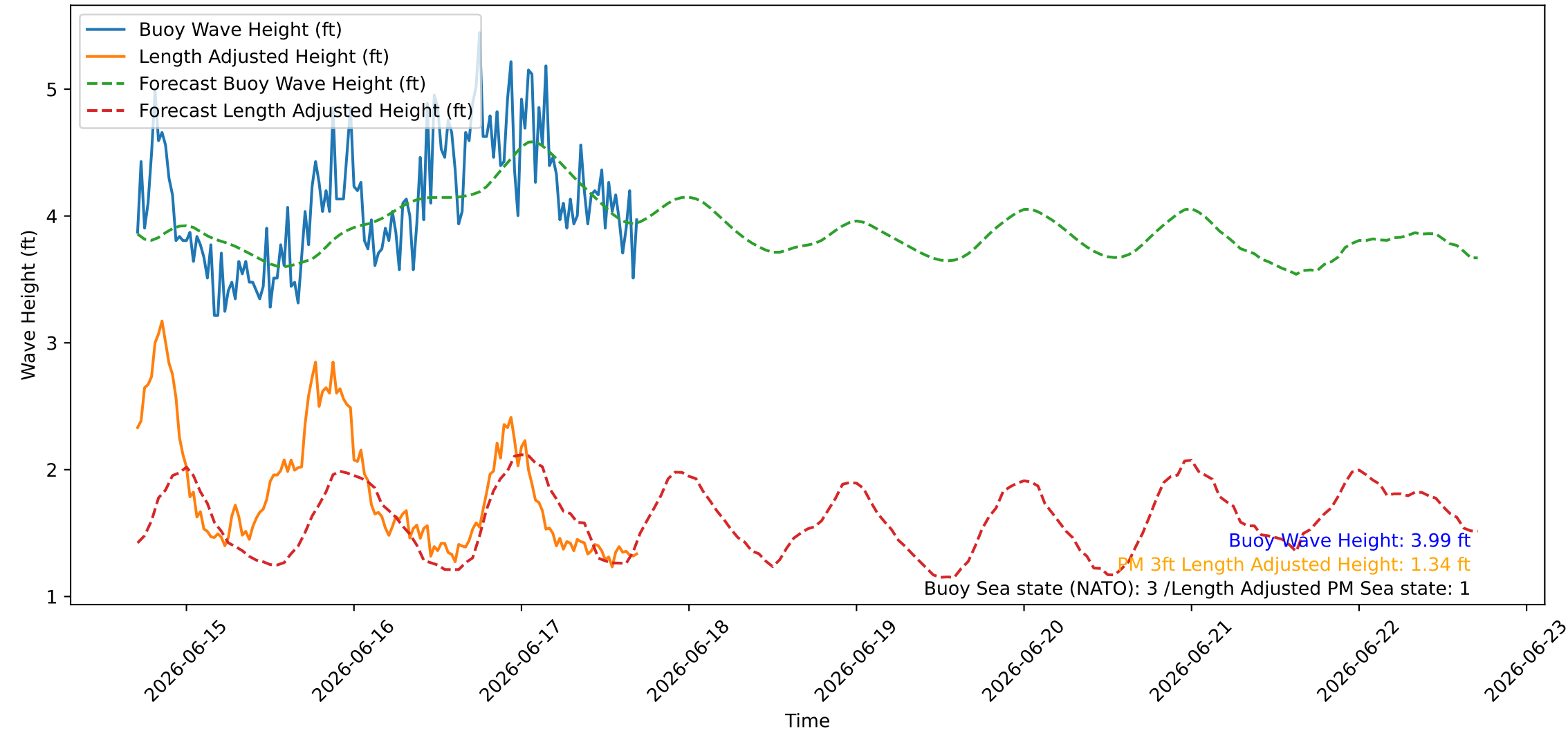
Wave Heights over Time for Oceanside Harbor at 2026-06-17 17:00:27
