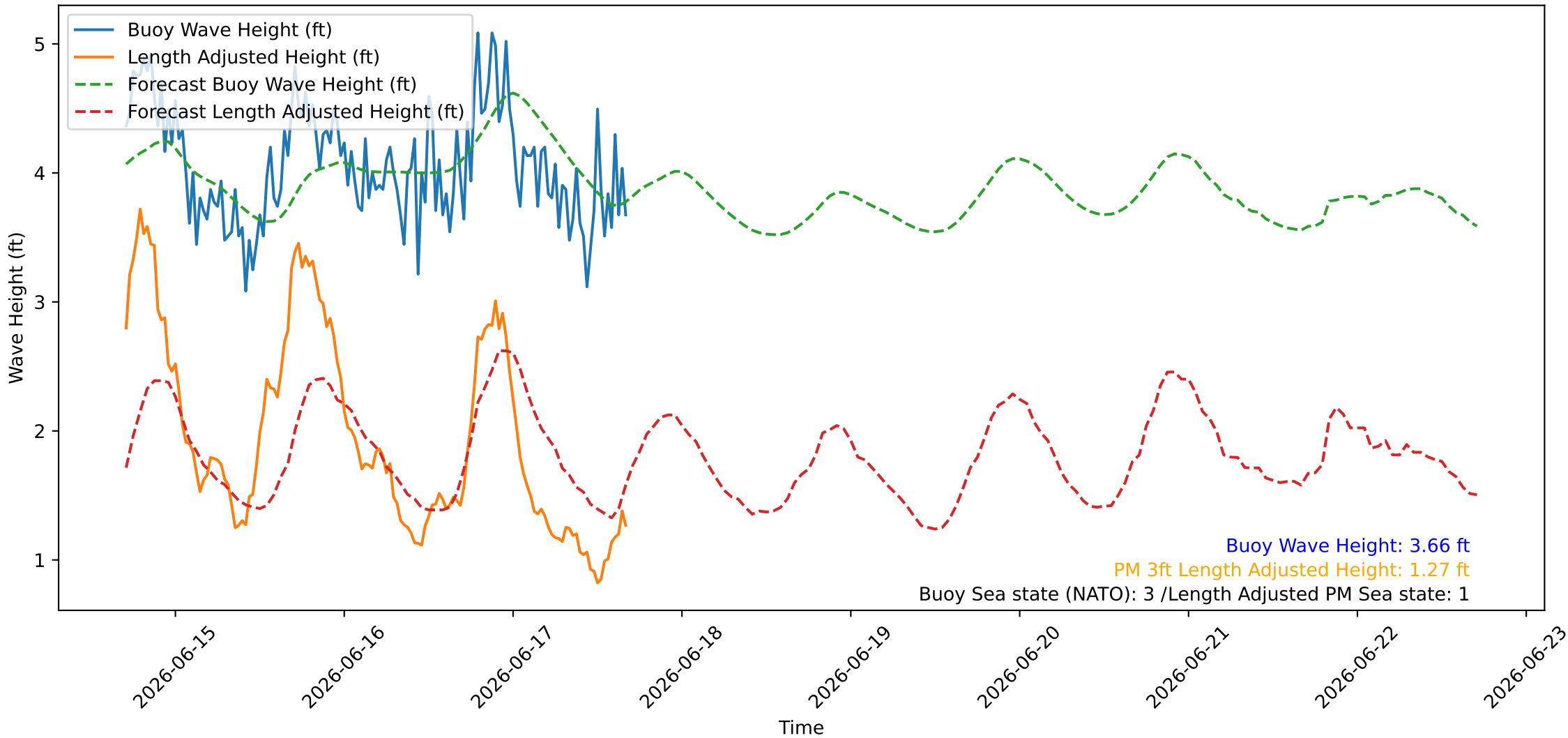
Wave Heights over Time for Green Beach at 2026-06-17 17:01:08
