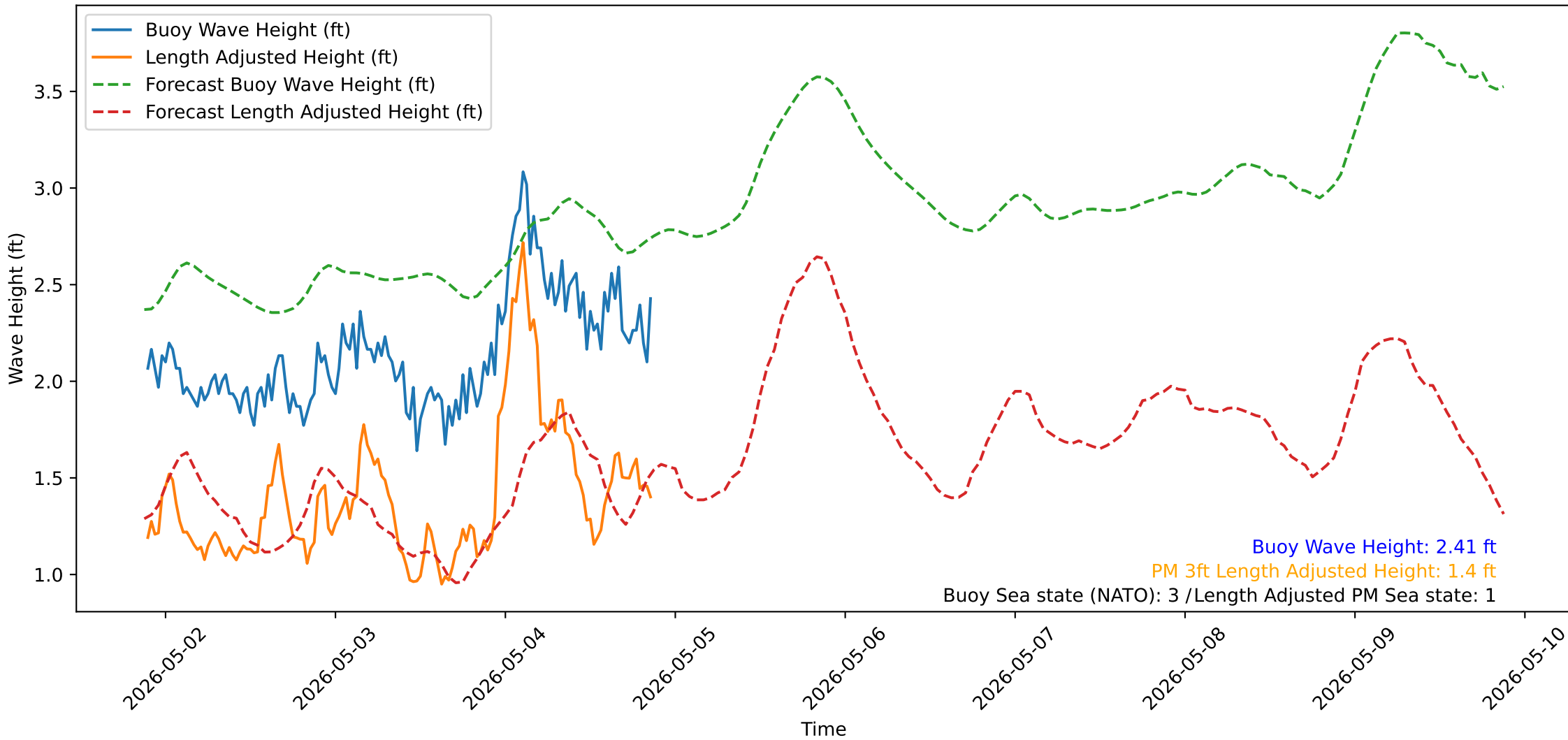
Wave Heights over Time for Oceanside Harbor at 2026-05-04 21:20:31
