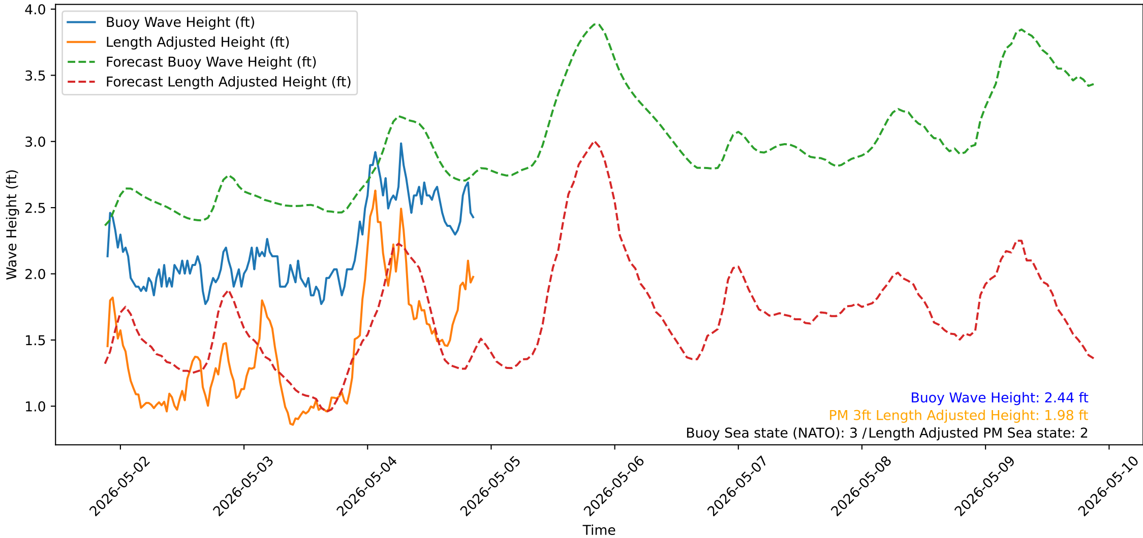
Wave Heights over Time for Green Beach at 2026-05-04 21:21:14
