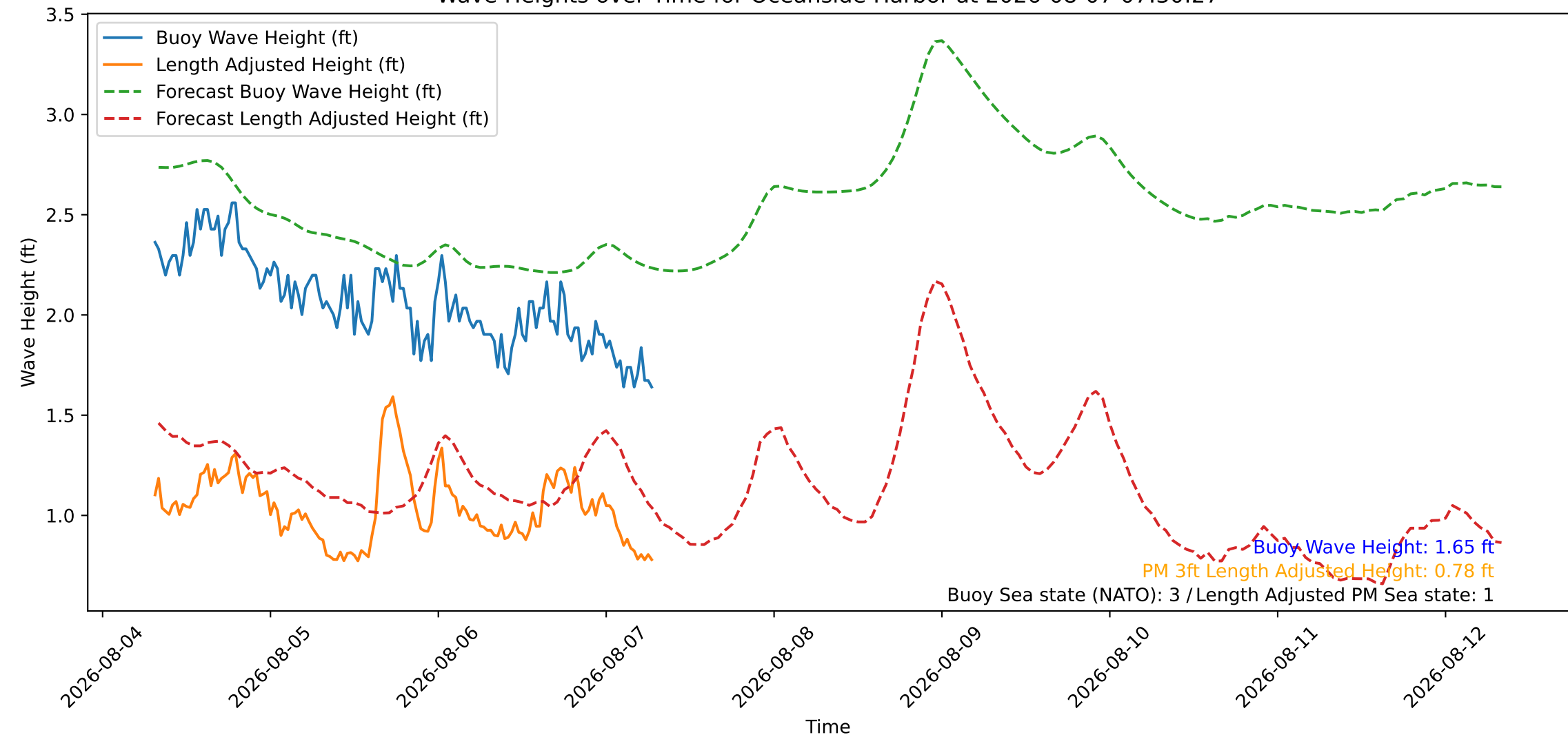
Wave Heights over Time for Oceanside Harbor at 2026-08-07 07:30:27
