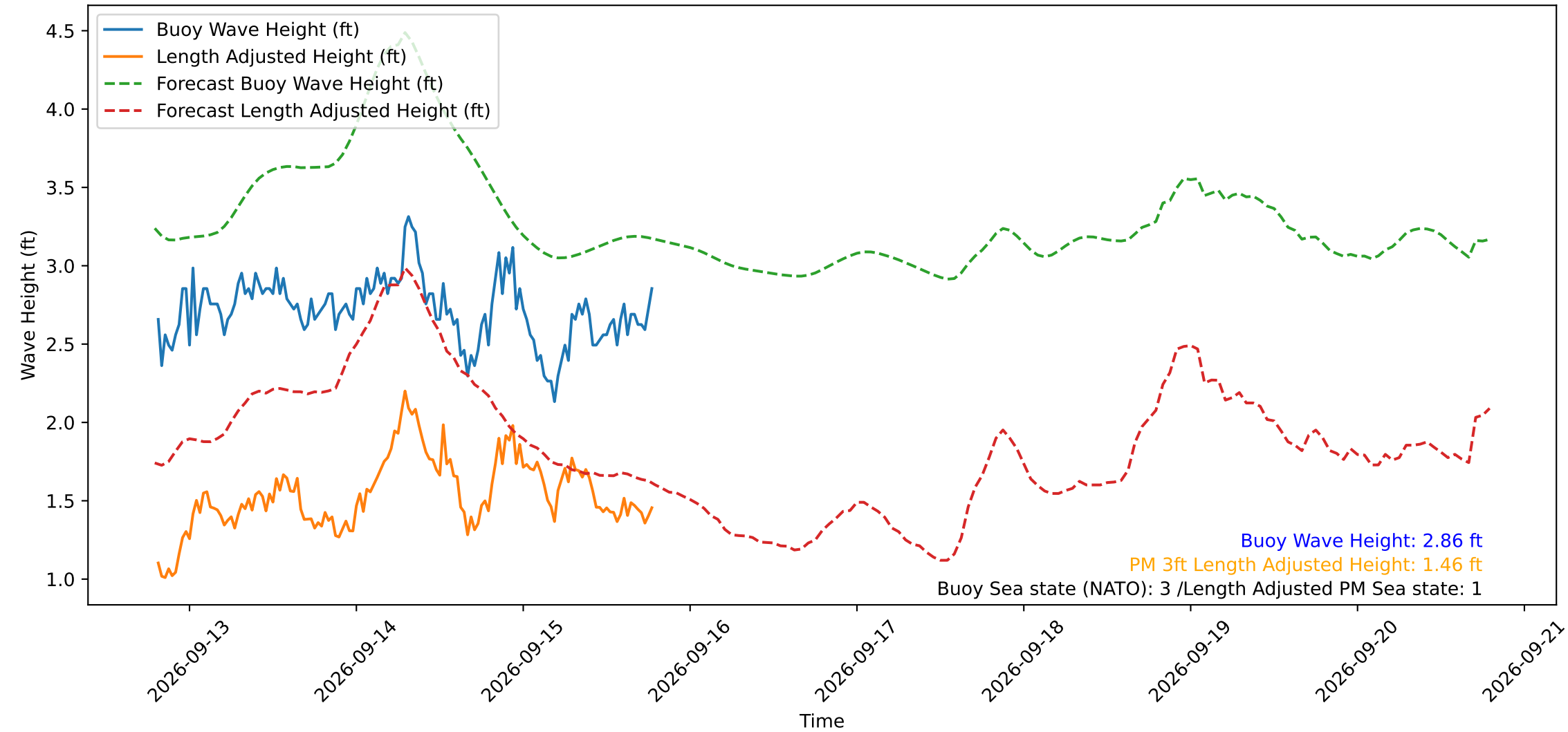
Wave Heights over Time for Green Beach at 2026-09-15 19:21:15
