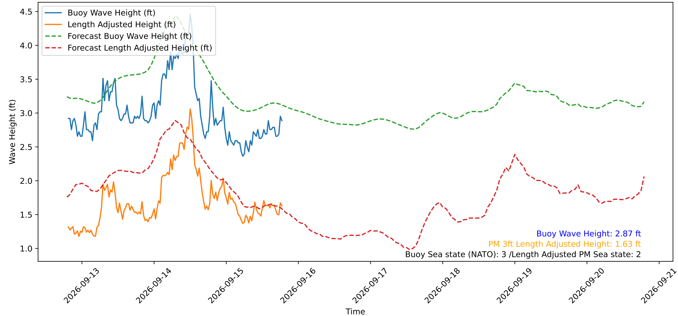
Wave Heights over Time for Oceanside Harbor at 2026-09-15 19:20:30
