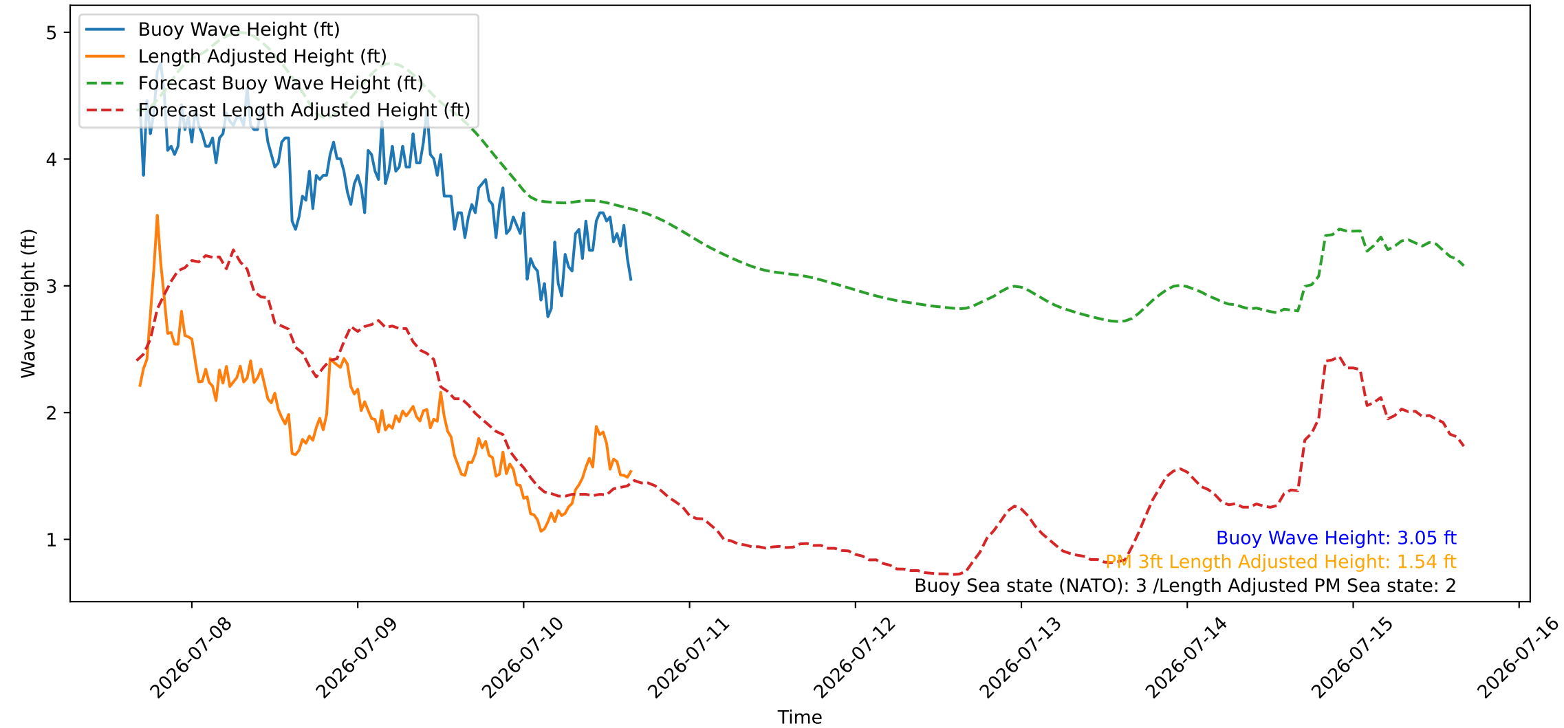
Wave Heights over Time for Green Beach at 2026-07-10 16:21:08
