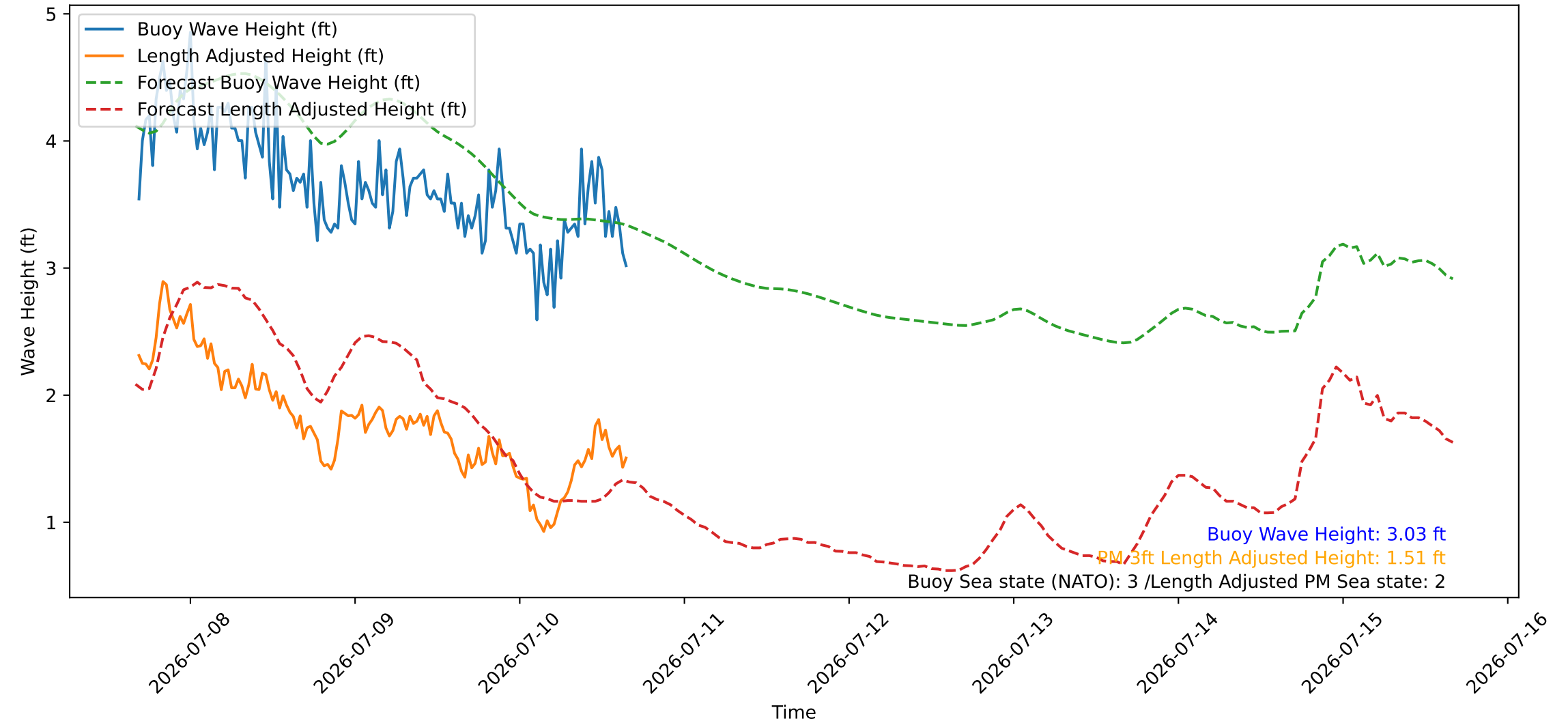
Wave Heights over Time for Red Beach at 2026-07-10 16:20:46
