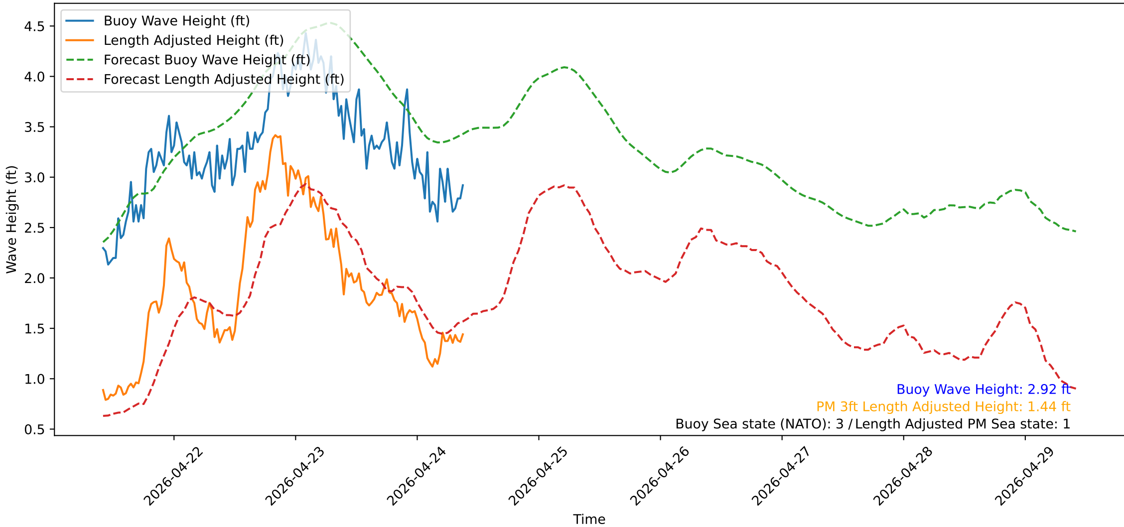
Wave Heights over Time for Oceanside Harbor at 2026-04-24 09:50:30
