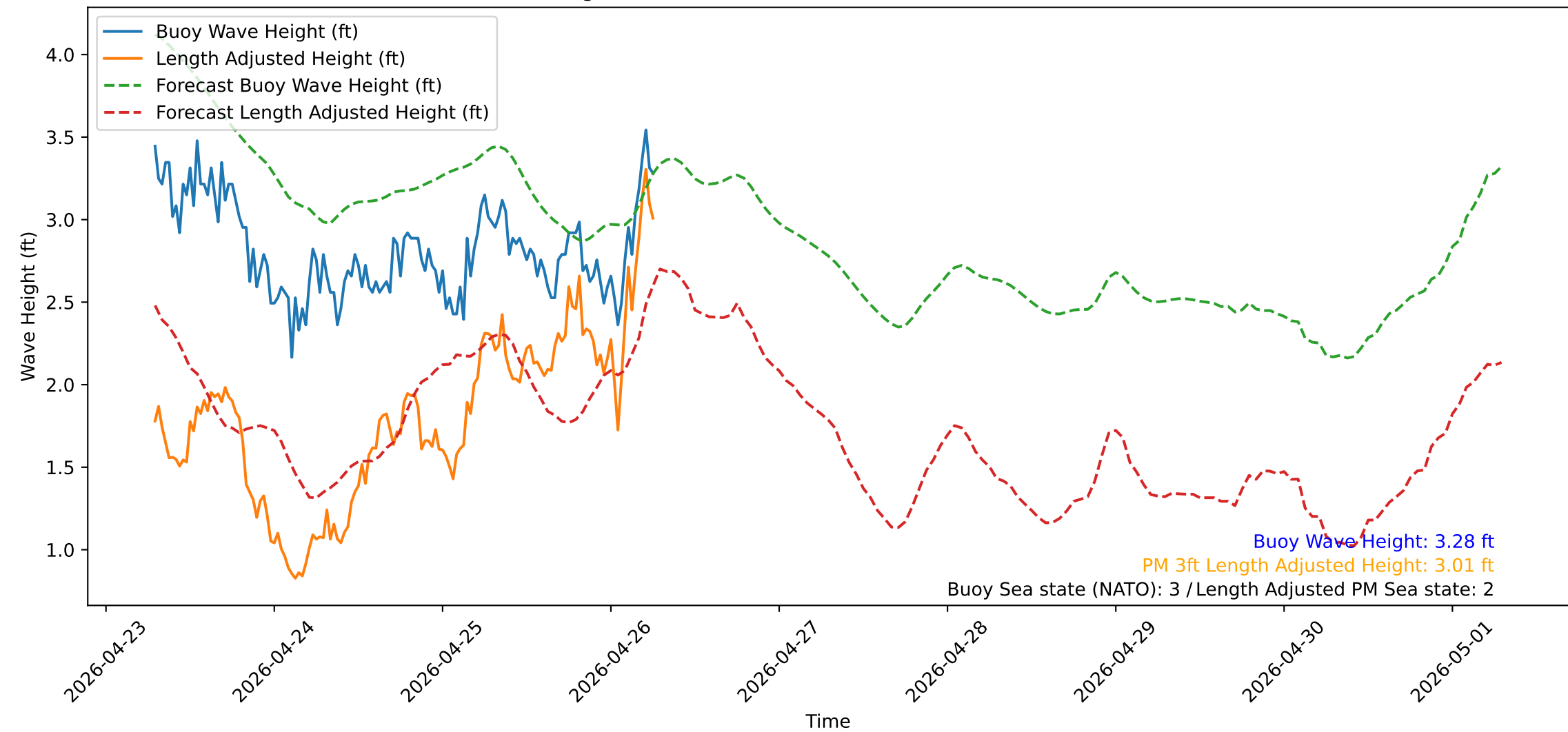
Wave Heights over Time for Red Beach at 2026-04-26 06:50:51
