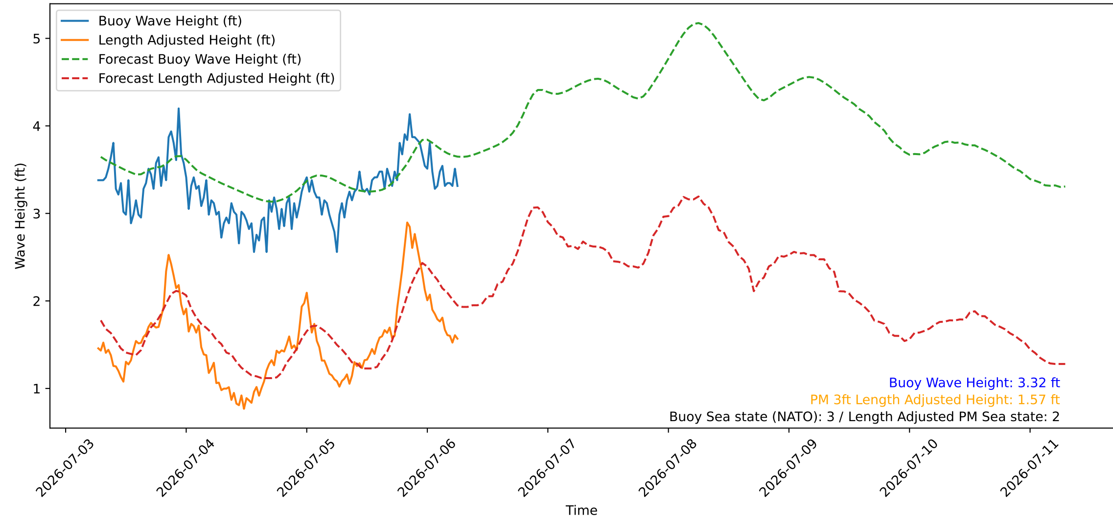
Wave Heights over Time for Green Beach at 2026-07-06 06:41:09
