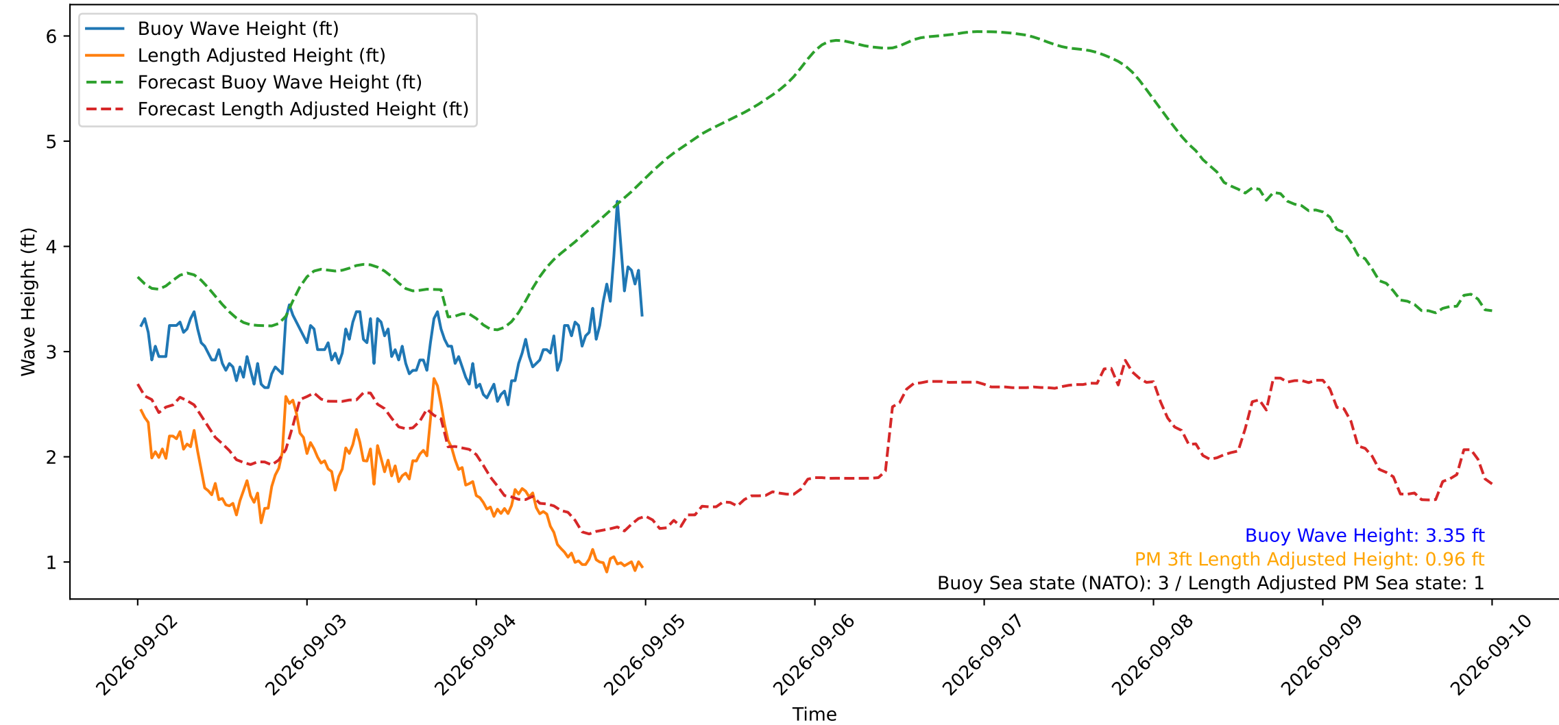
Wave Heights over Time for Green Beach at 2026-09-05 00:11:13
