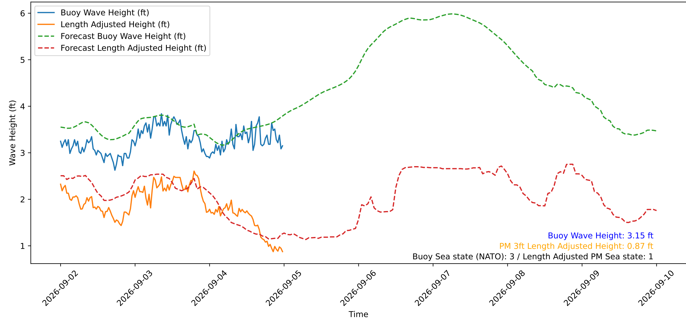
Wave Heights over Time for Oceanside Harbor at 2026-09-05 00:10:30
