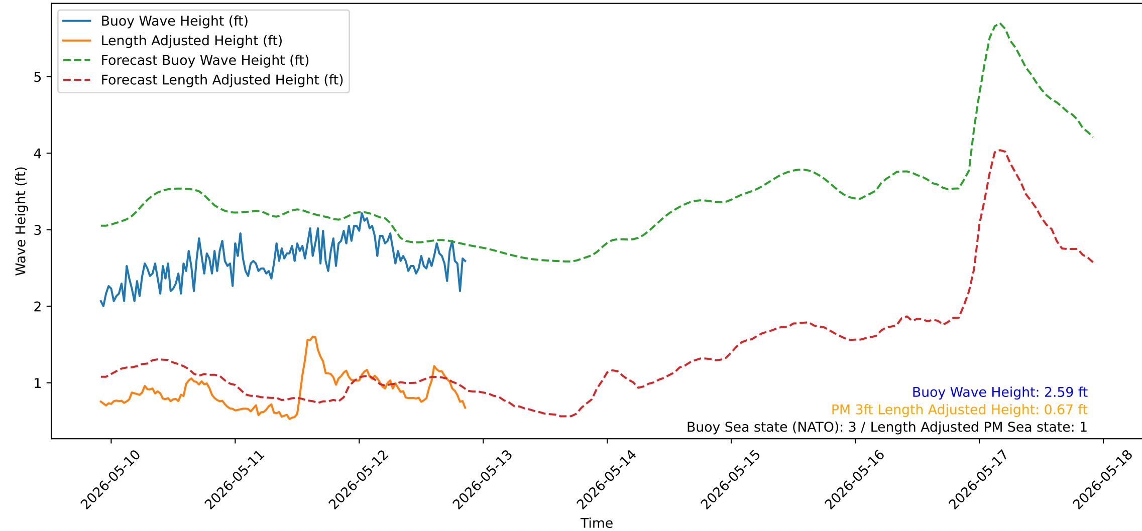
Wave Heights over Time for Red Beach at 2026-05-12 21:30:52
