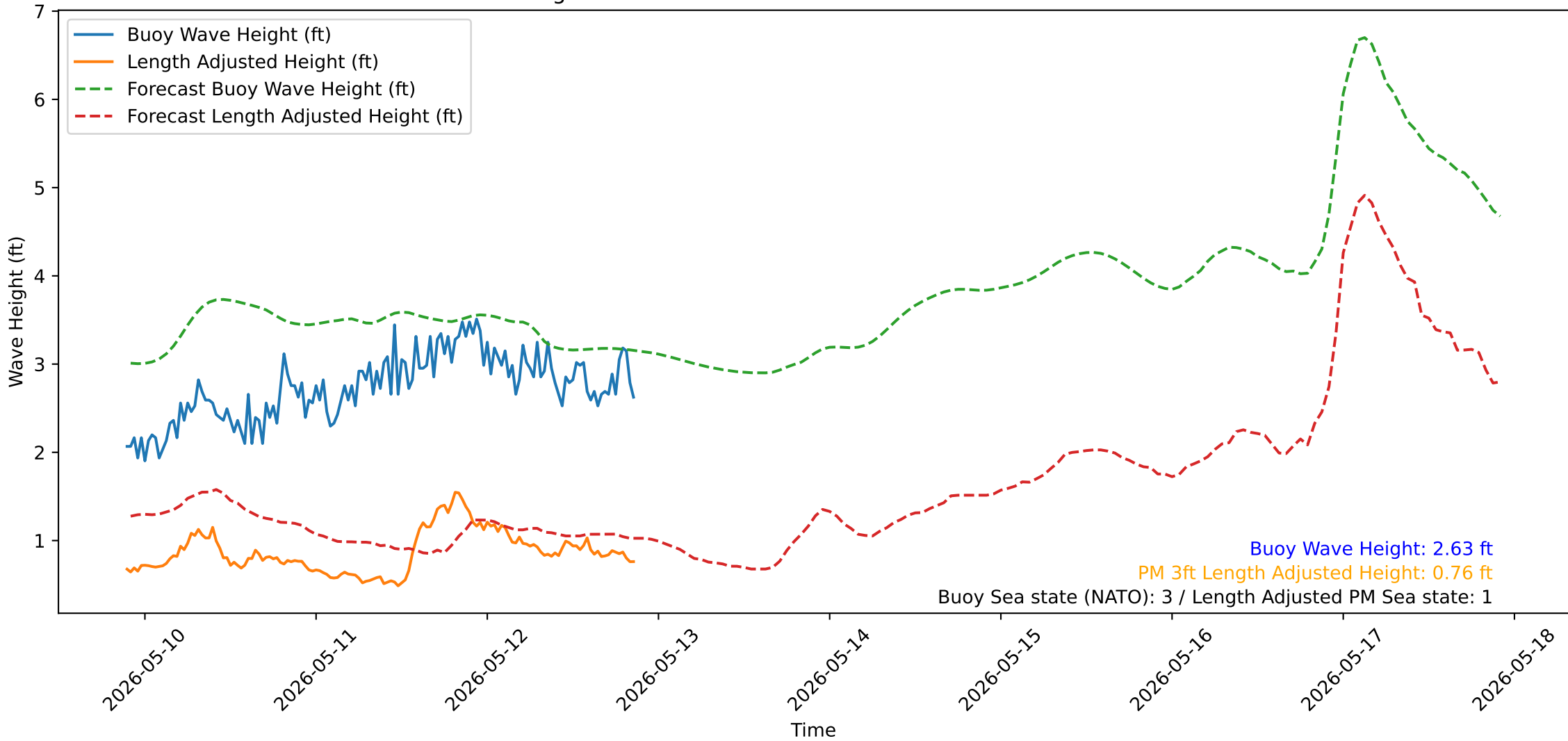
Wave Heights over Time for Green Beach at 2026-05-12 21:31:15
