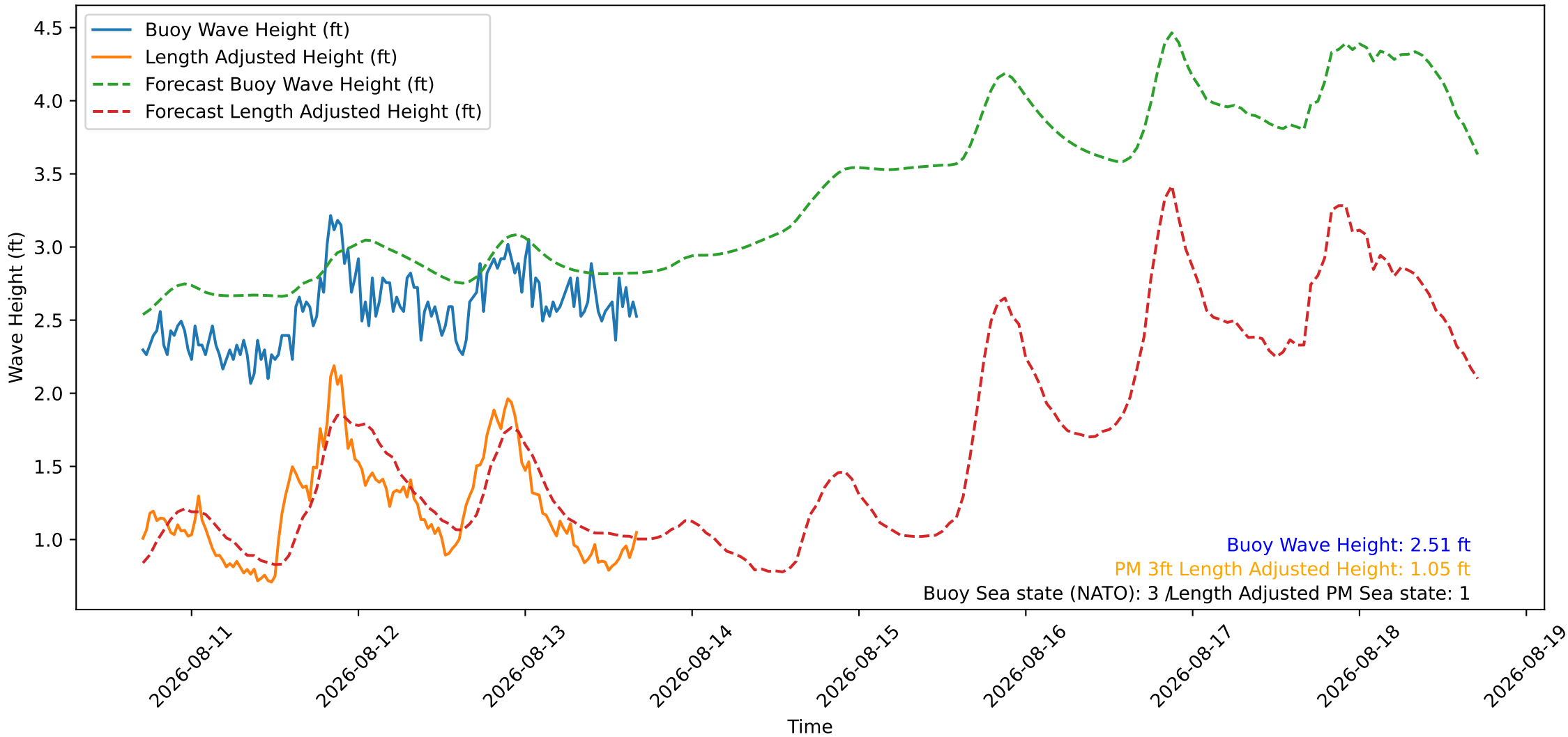
Wave Heights over Time for Green Beach at 2026-08-13 17:01:08
