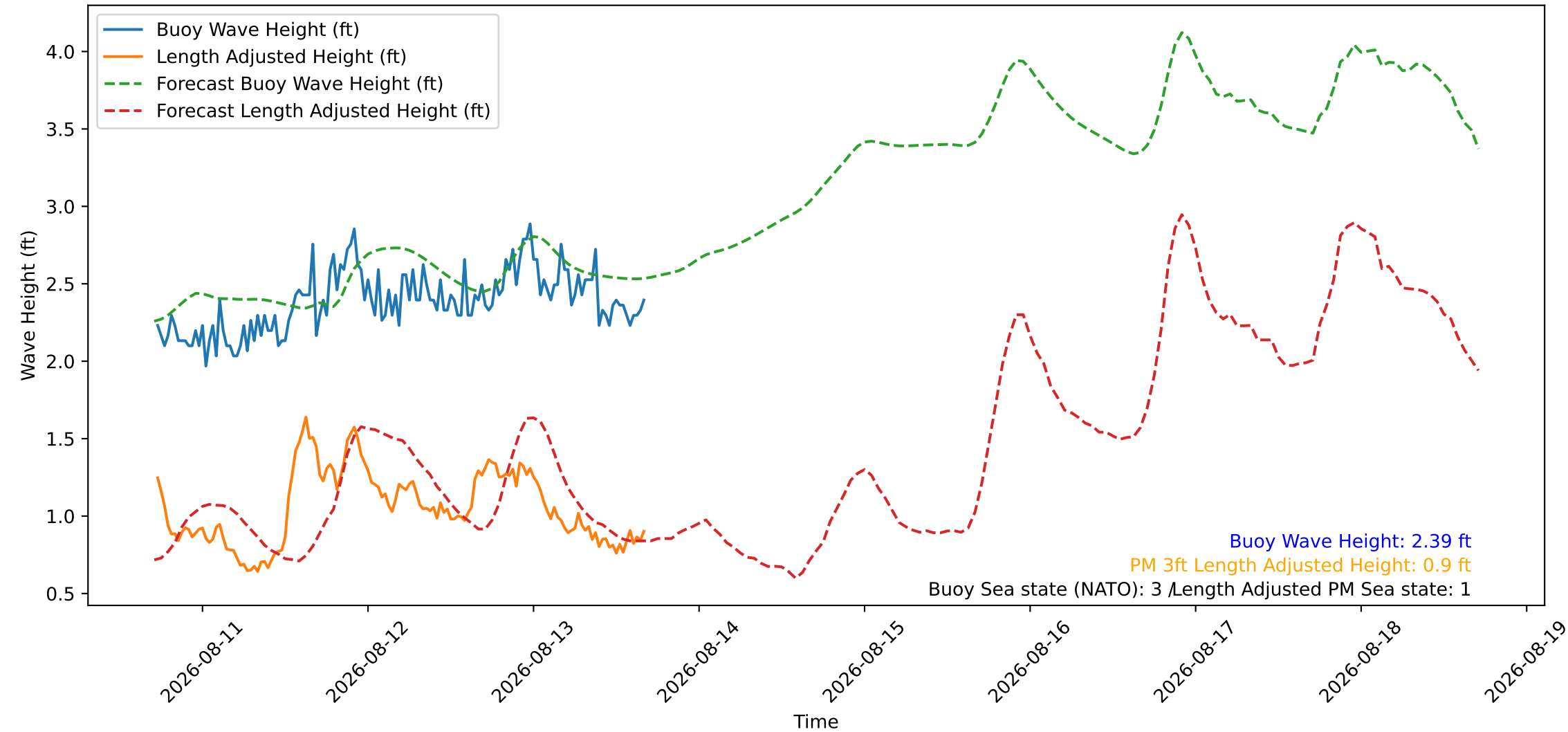
Wave Heights over Time for Red Beach at 2026-08-13 17:00:46
