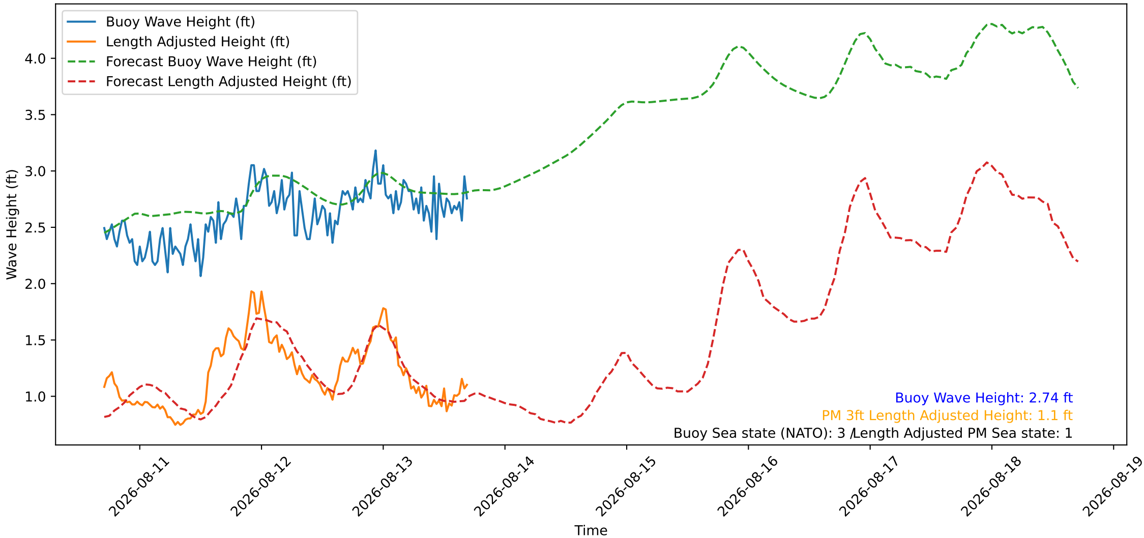
Wave Heights over Time for Oceanside Harbor at 2026-08-13 17:00:26
