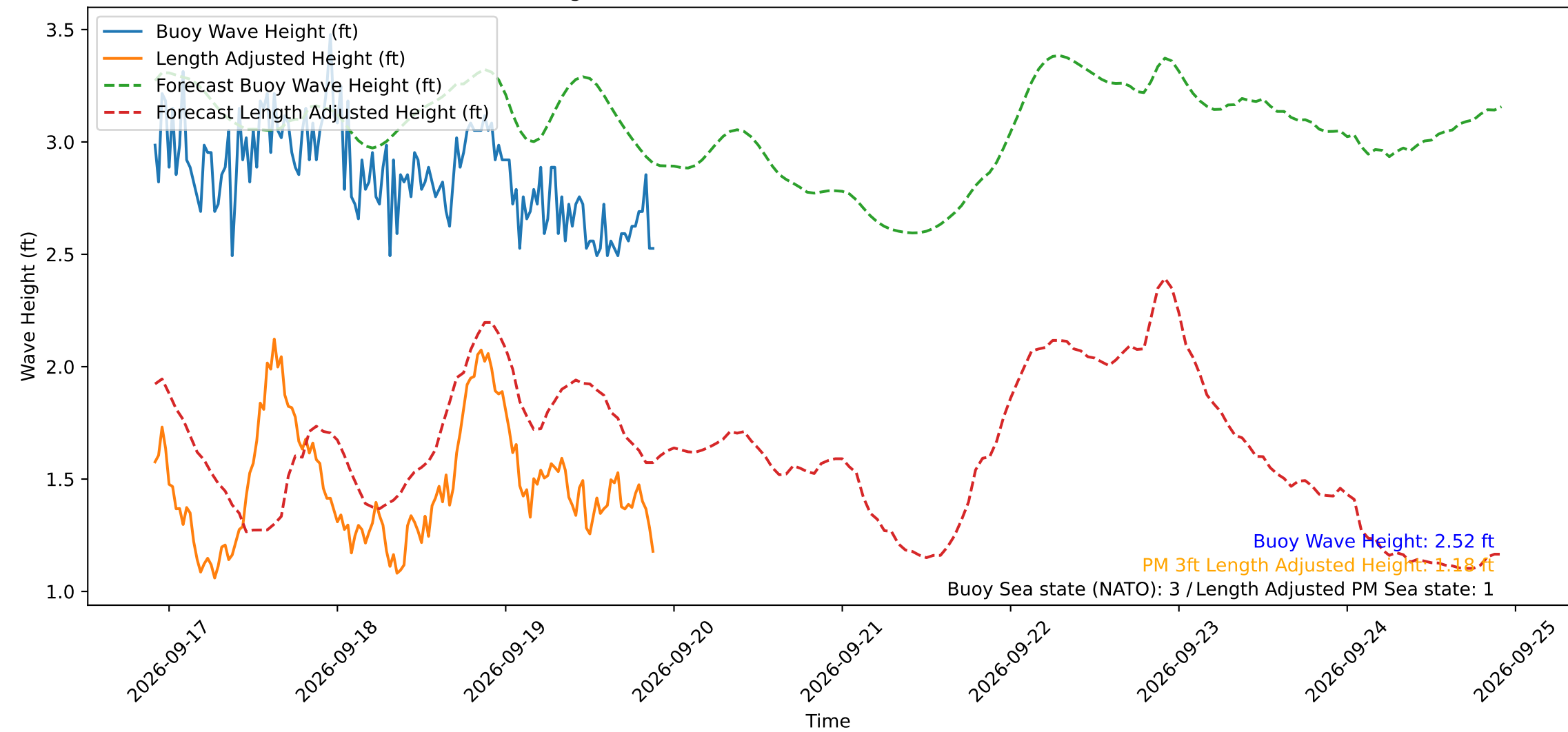
Wave Heights over Time for Green Beach at 2026-09-19 21:51:13
