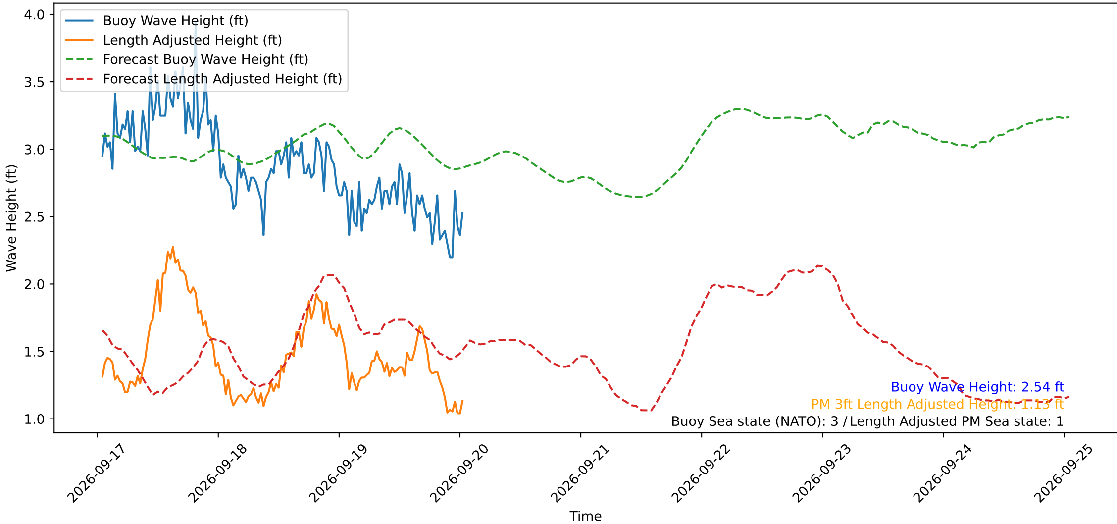
Wave Heights over Time for Oceanside Harbor at 2026-09-20 01:10:29
