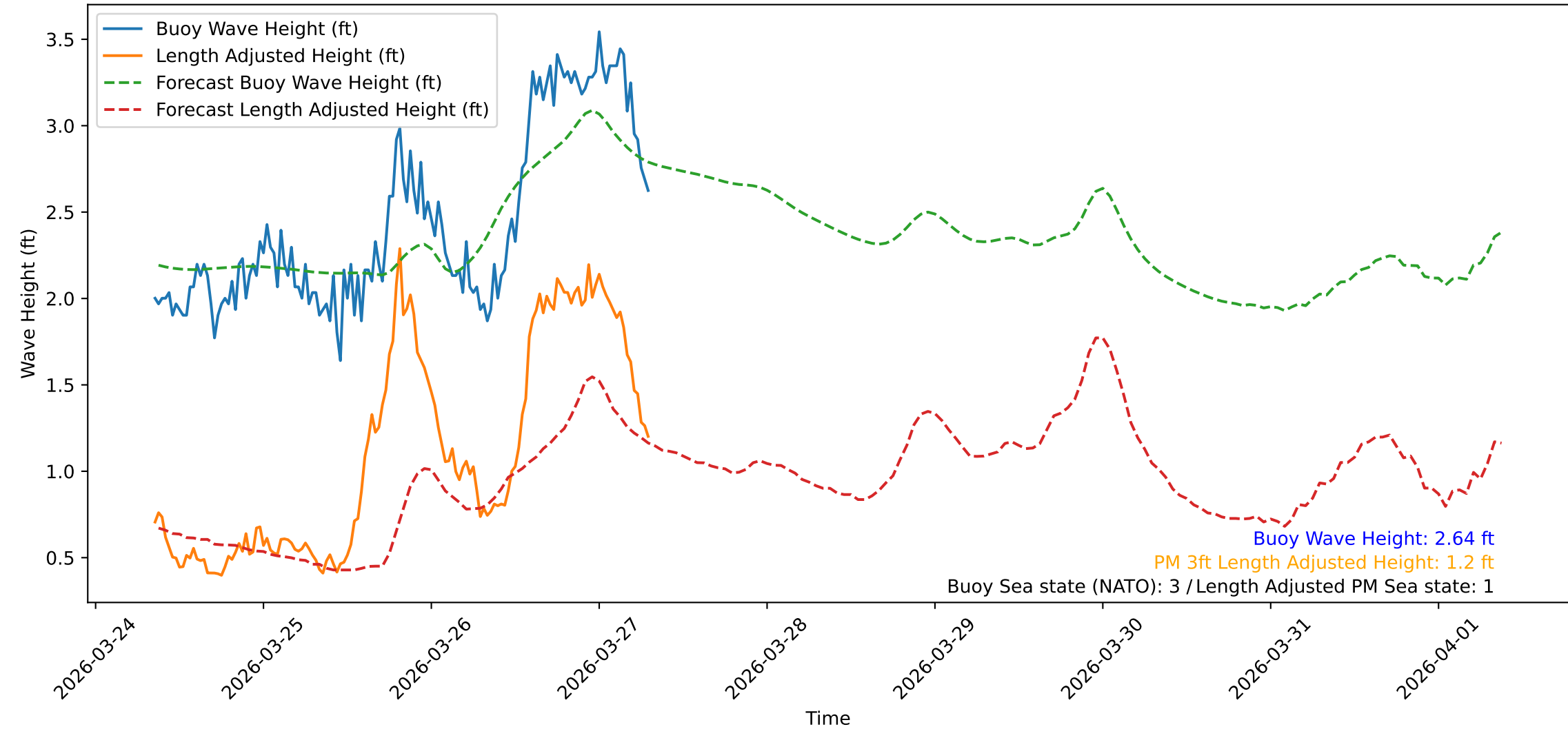
Wave Heights over Time for Green Beach at 2026-03-27 08:31:10
