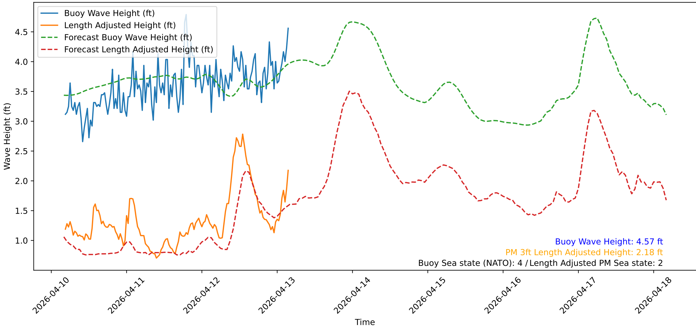
Wave Heights over Time for Oceanside Harbor at 2026-04-13 04:20:31
