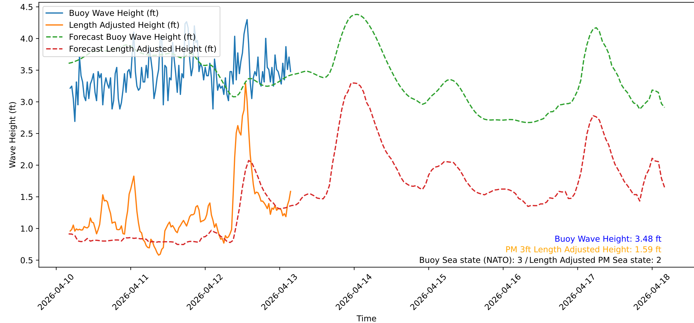
Wave Heights over Time for Red Beach at 2026-04-13 04:20:51
