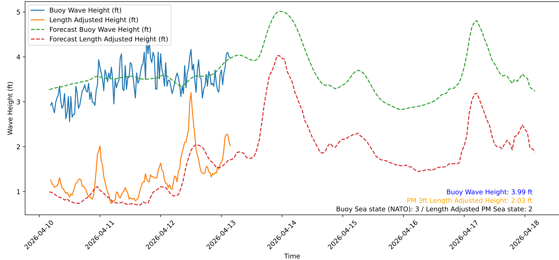
Wave Heights over Time for Green Beach at 2026-04-13 04:21:13
