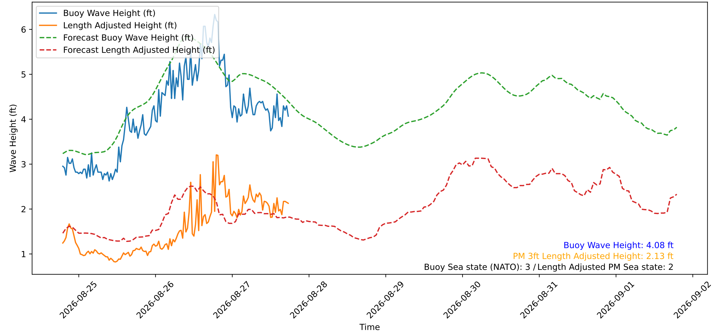
Wave Heights over Time for Green Beach at 2026-08-27 18:31:11
