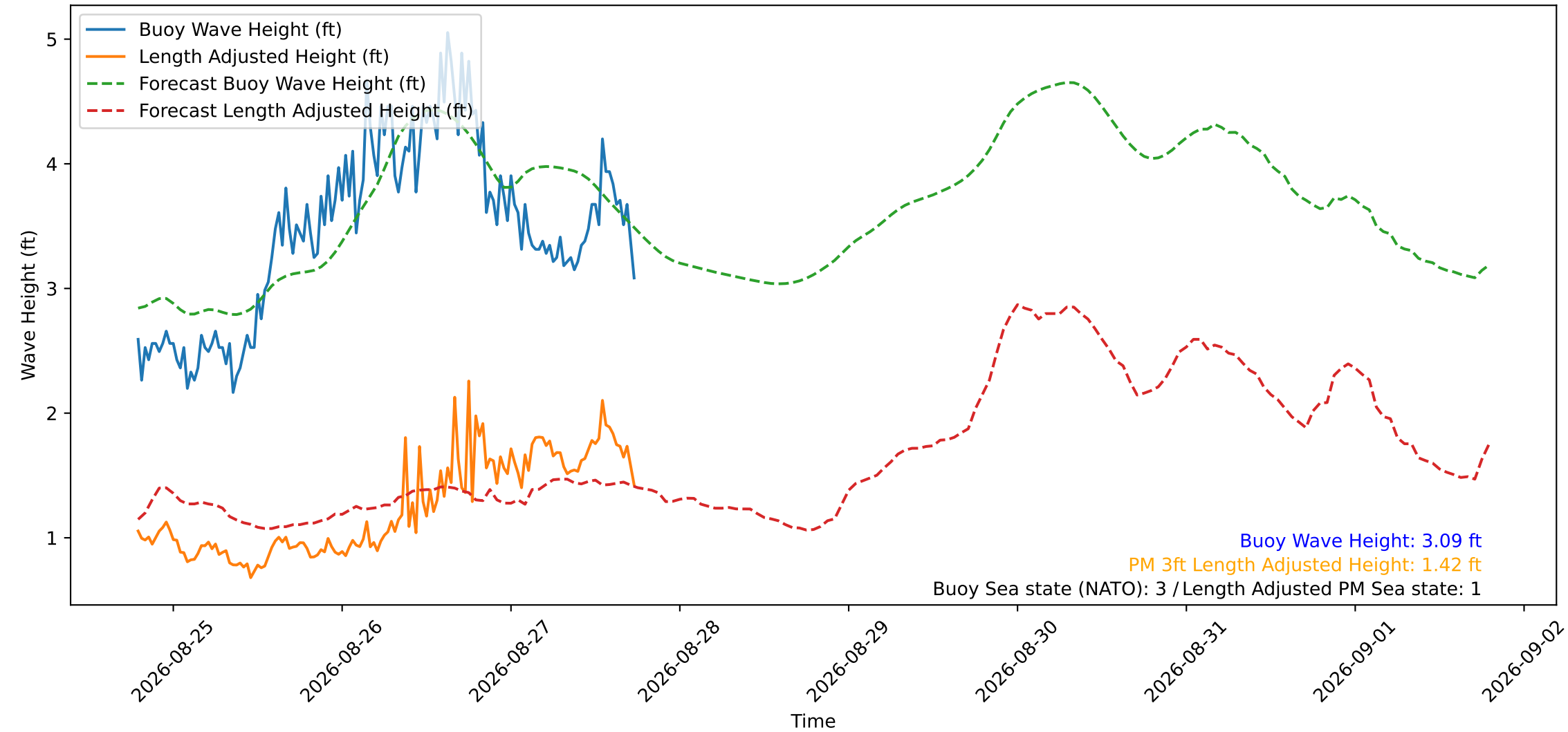
Wave Heights over Time for Red Beach at 2026-08-27 18:30:49
