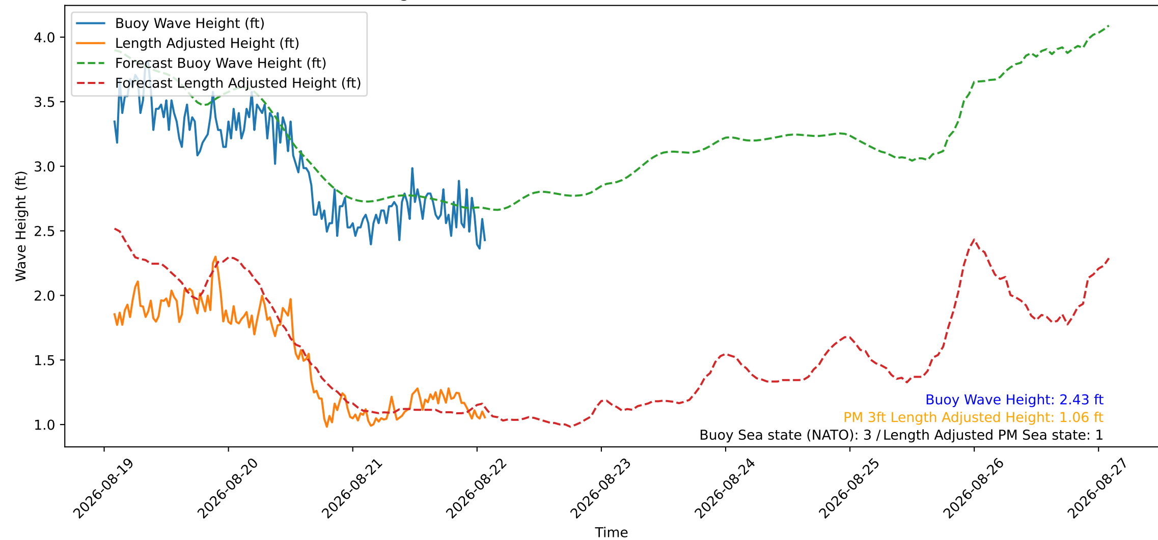
Wave Heights over Time for Oceanside Harbor at 2026-08-22 02:10:30
