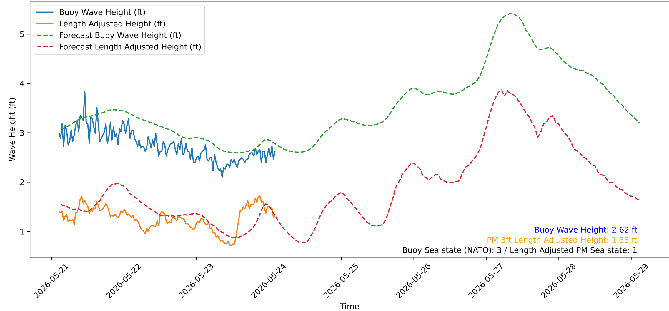
Wave Heights over Time for Oceanside Harbor at 2026-05-24 02:30:33
