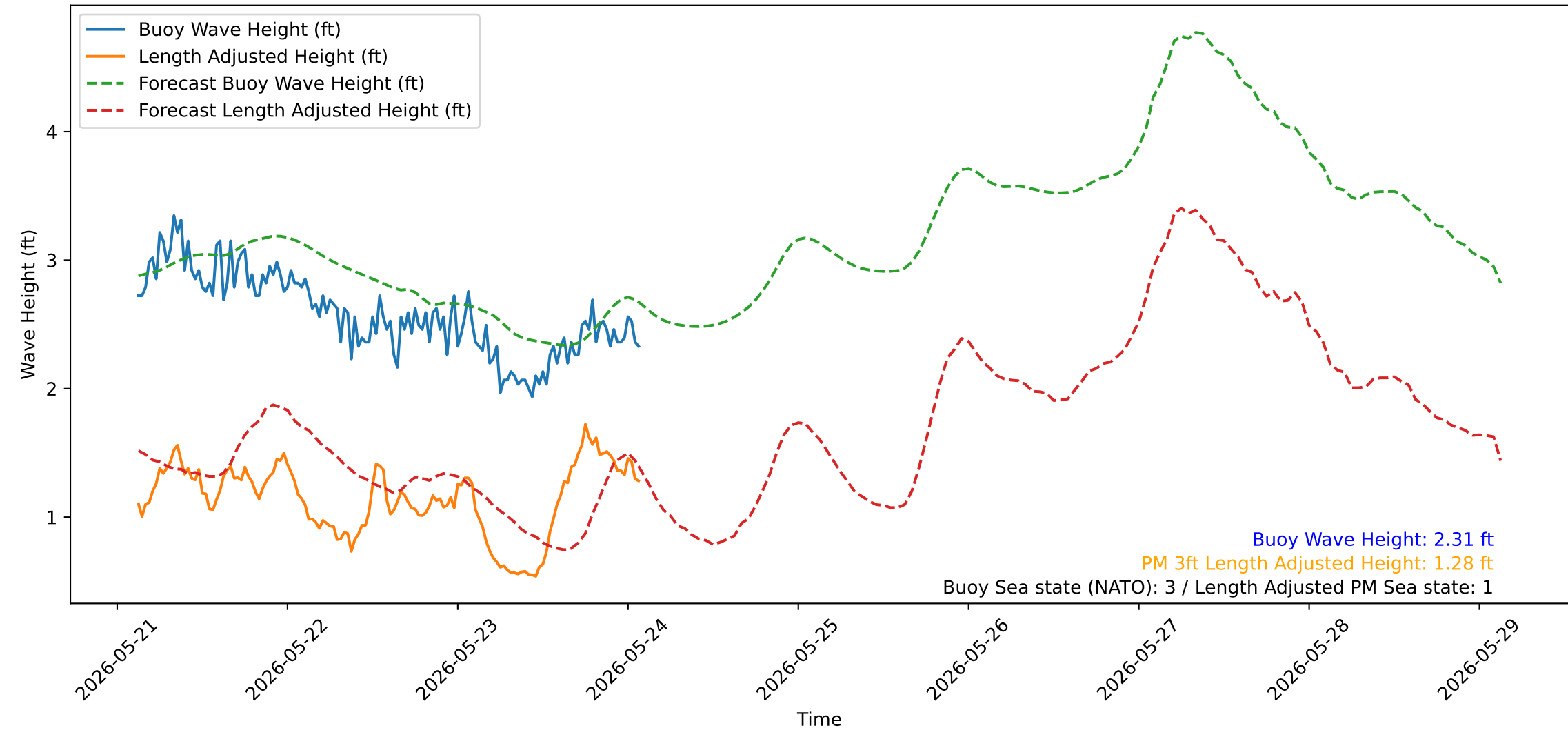
Wave Heights over Time for Red Beach at 2026-05-24 02:30:52
