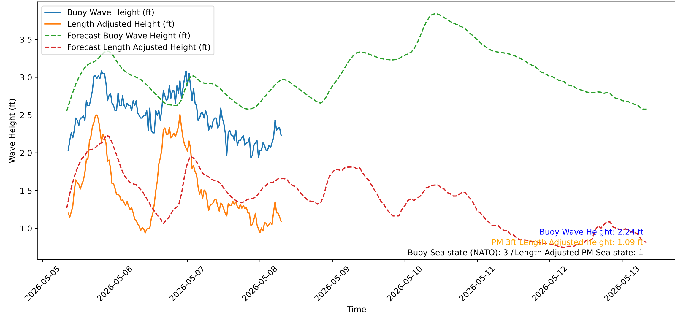
Wave Heights over Time for Red Beach at 2026-05-08 08:10:51
