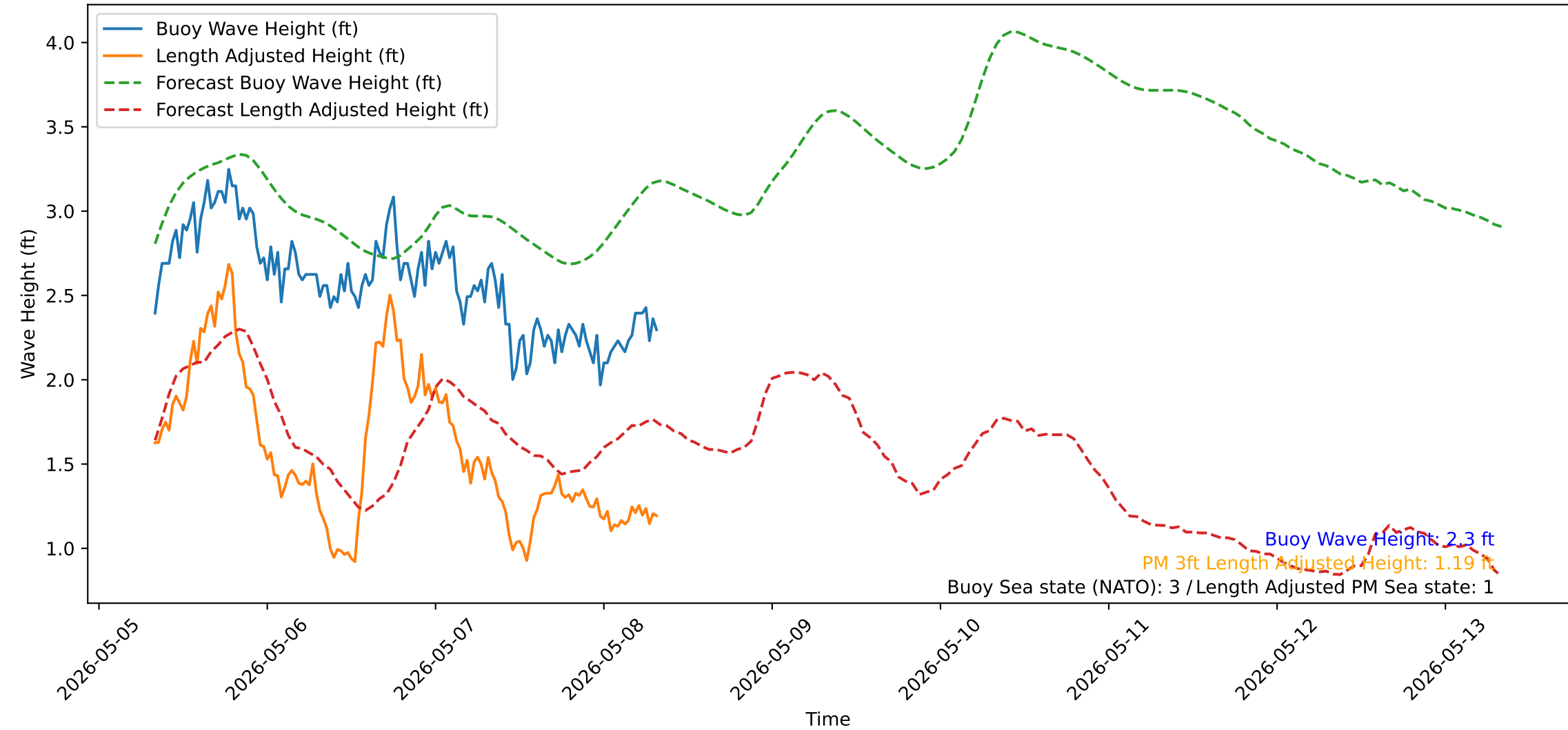
Wave Heights over Time for Oceanside Harbor at 2026-05-08 08:10:32
