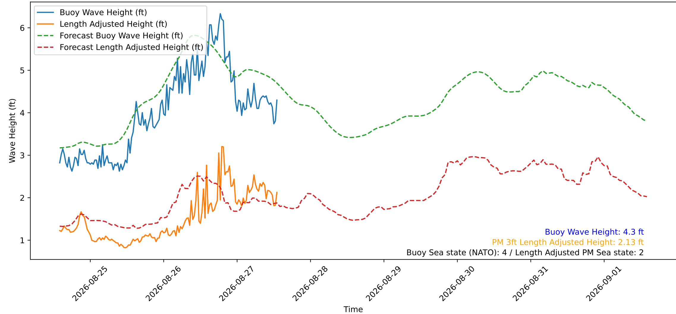
Wave Heights over Time for Green Beach at 2026-08-27 13:41:12
