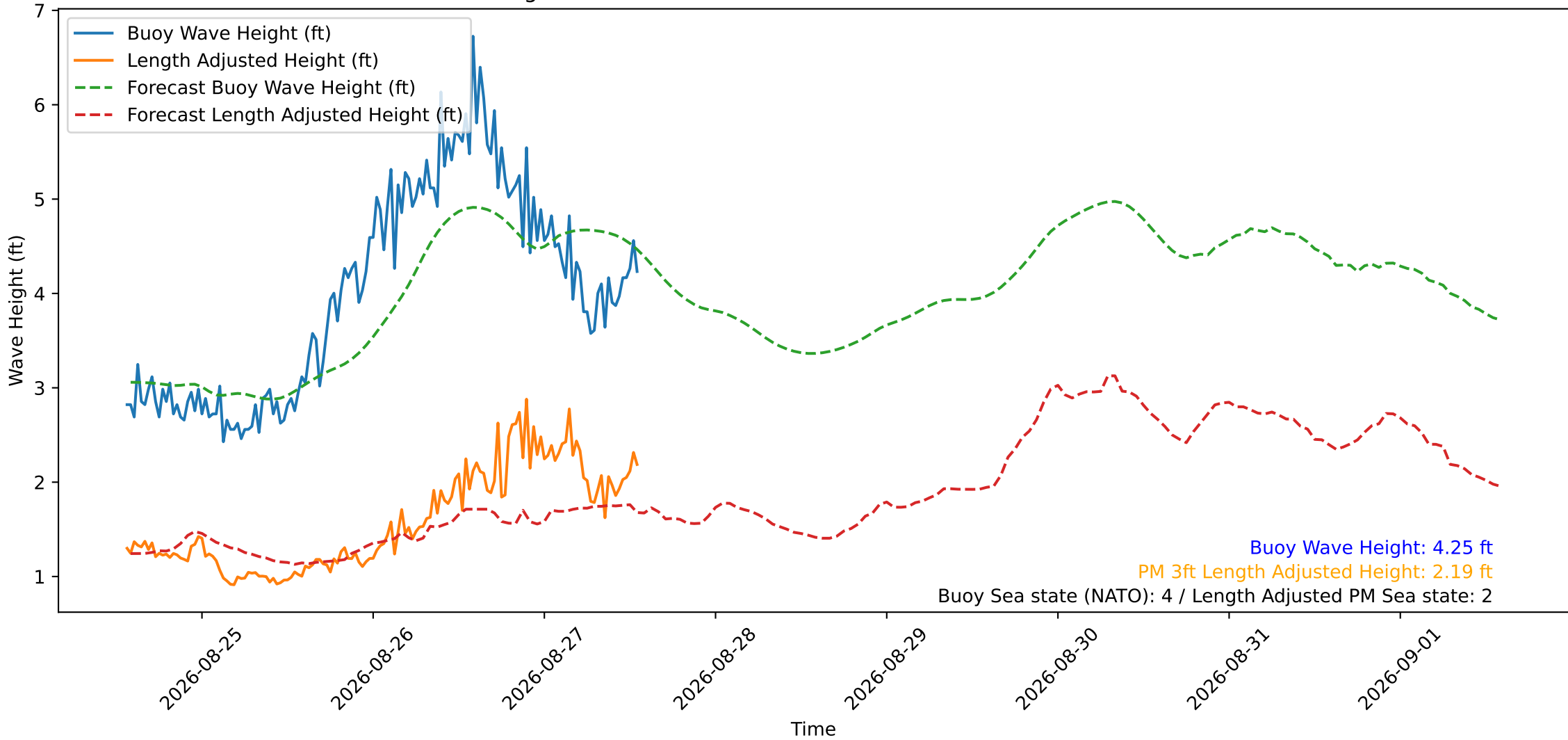
Wave Heights over Time for Oceanside Harbor at 2026-08-27 13:40:29
