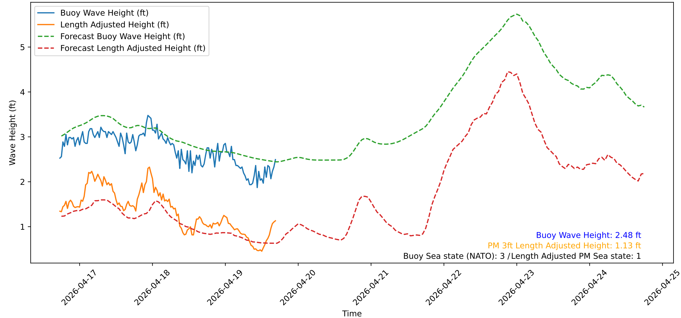
Wave Heights over Time for Green Beach at 2026-04-19 17:31:13
