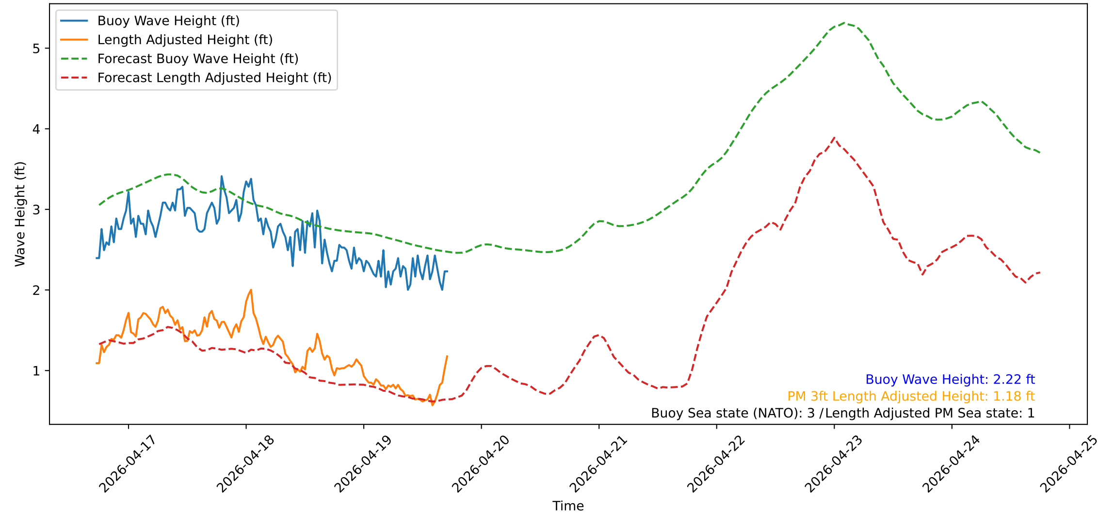
Wave Heights over Time for Oceanside Harbor at 2026-04-19 17:30:31
