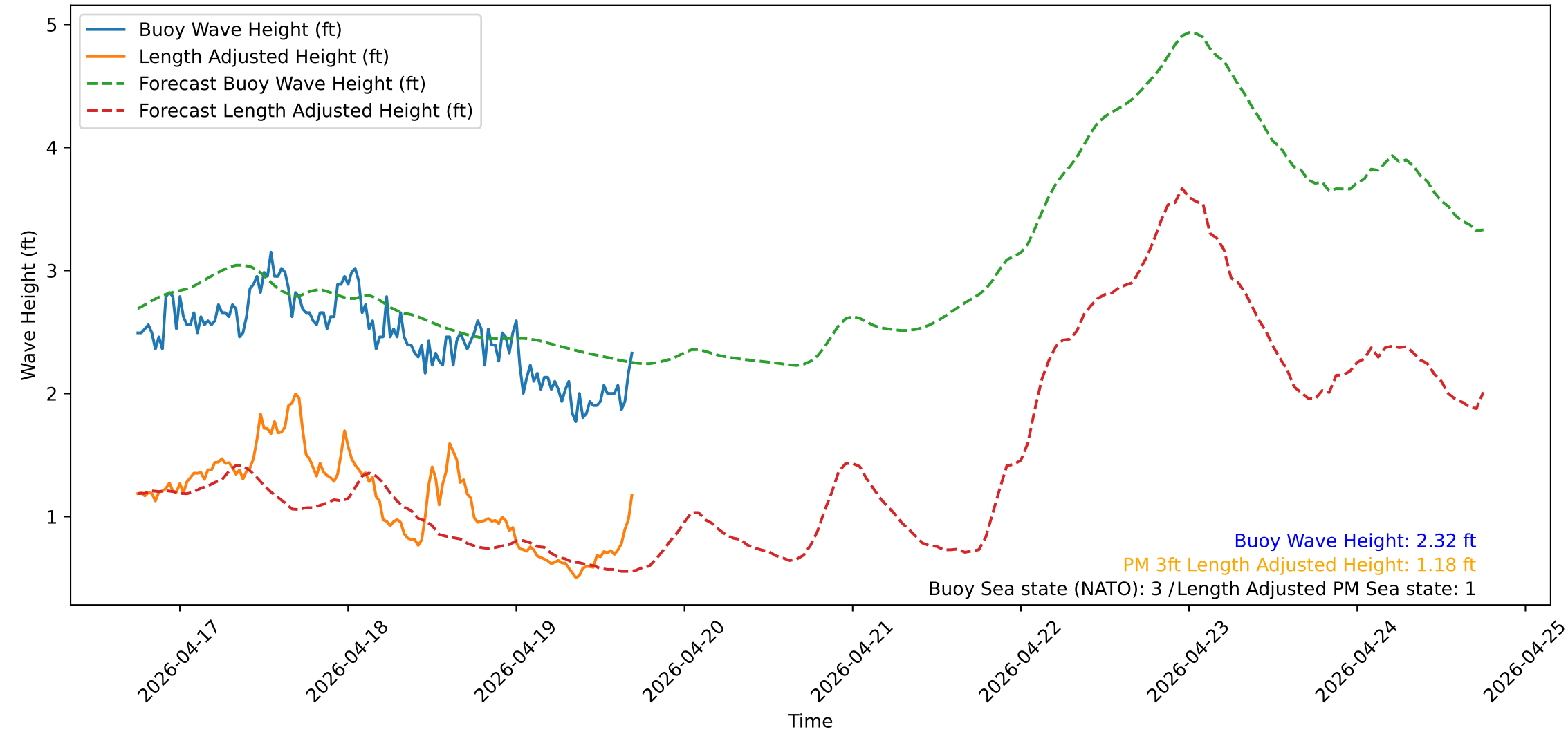
Wave Heights over Time for Red Beach at 2026-04-19 17:30:50
