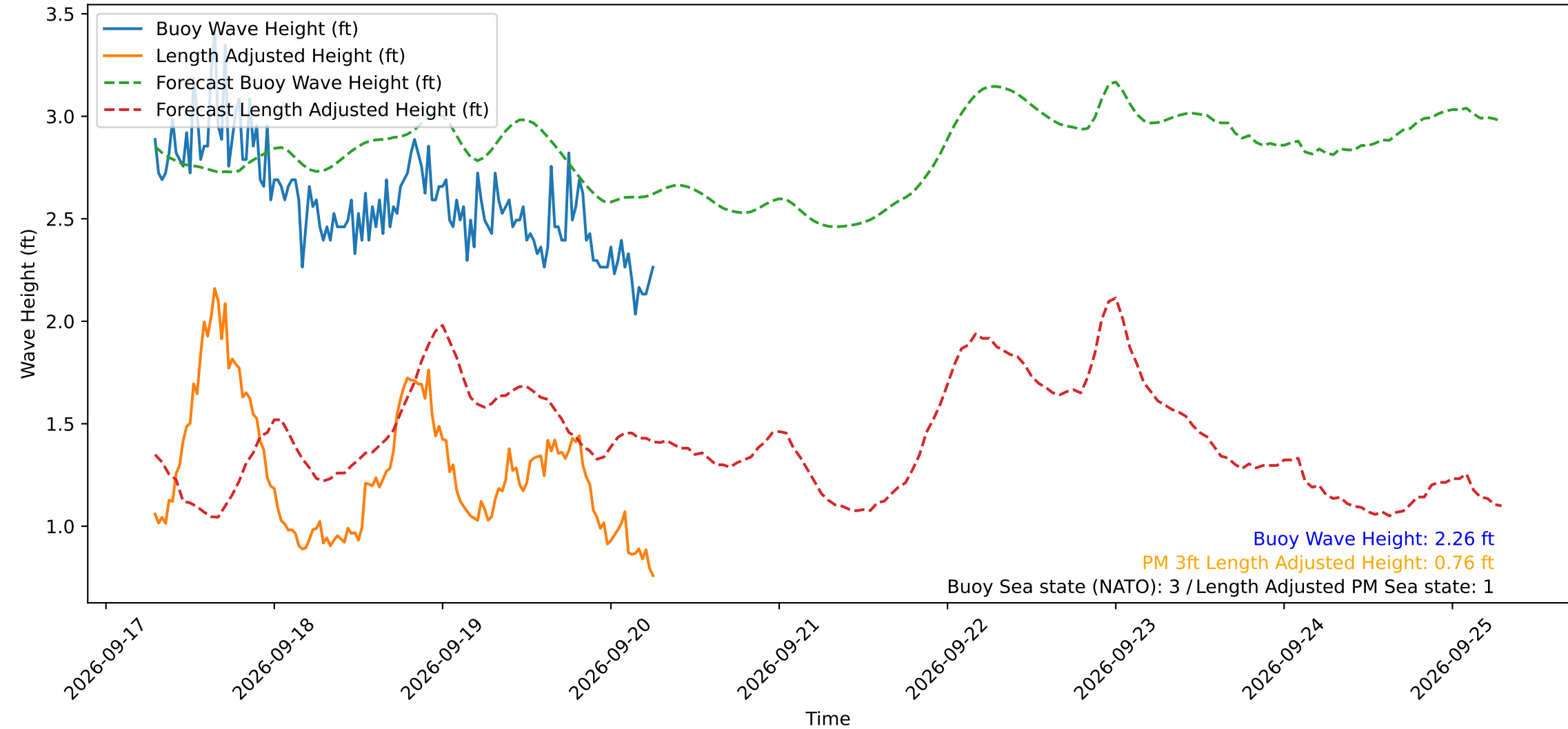
Wave Heights over Time for Red Beach at 2026-09-20 06:40:49
