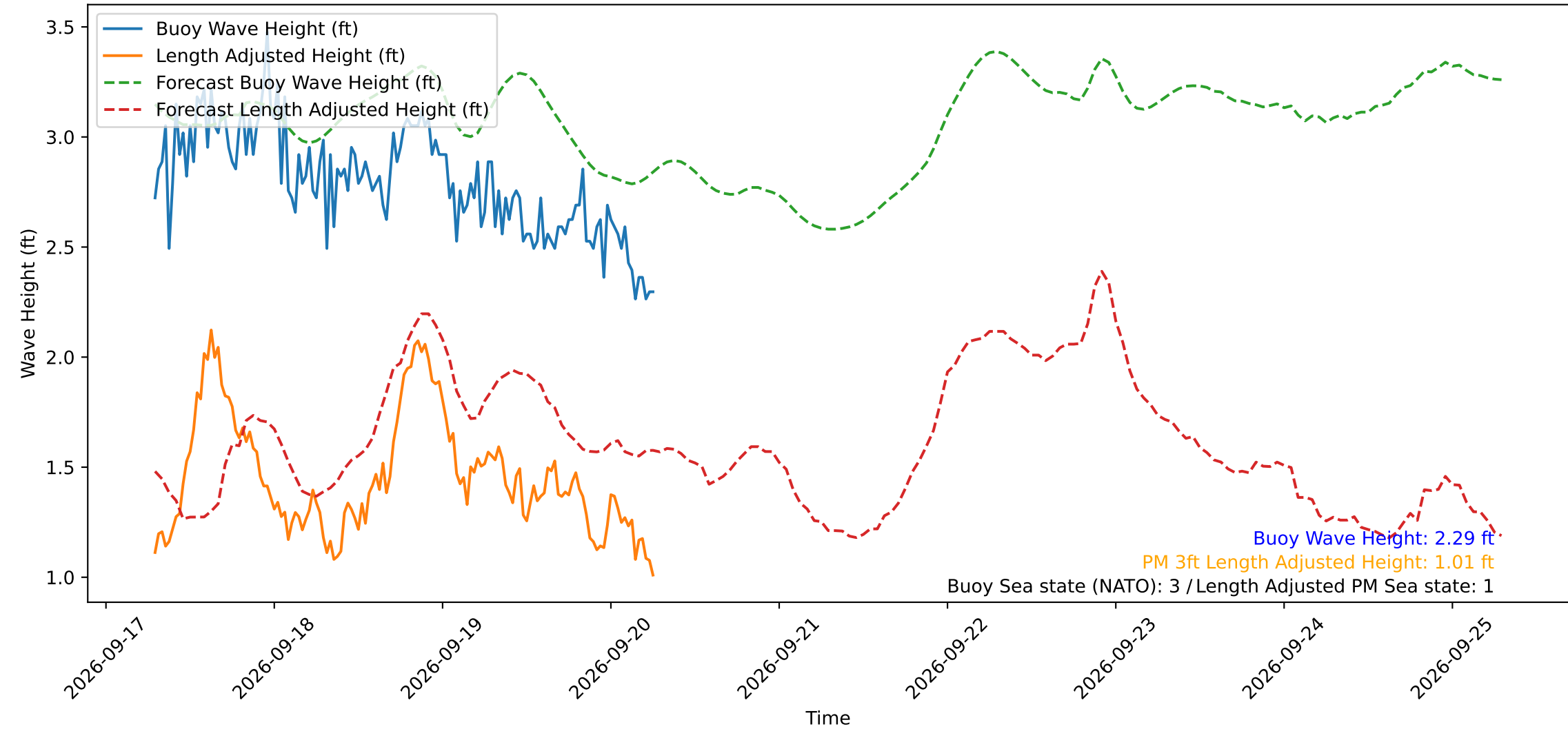
Wave Heights over Time for Green Beach at 2026-09-20 06:41:11
