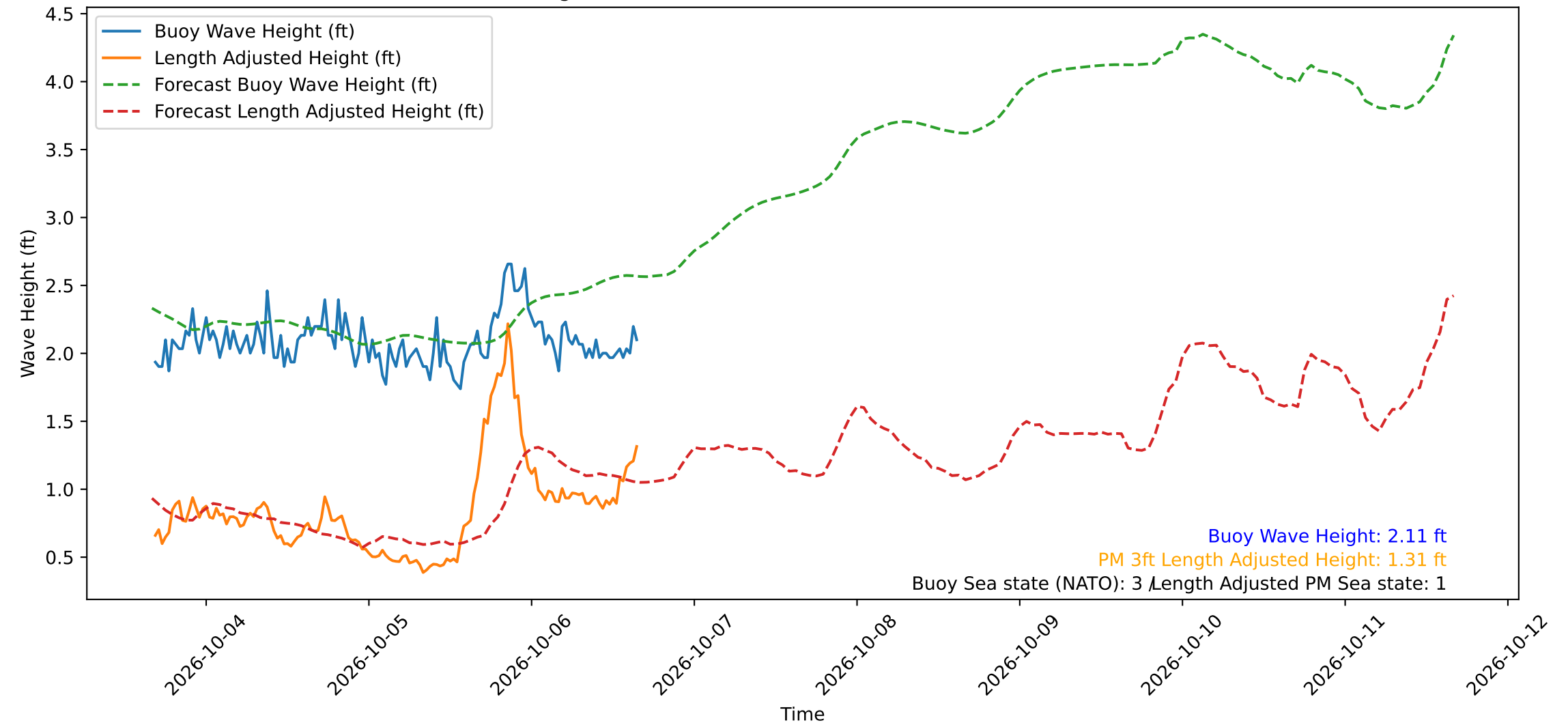
Wave Heights over Time for Red Beach at 2026-10-06 16:10:52
