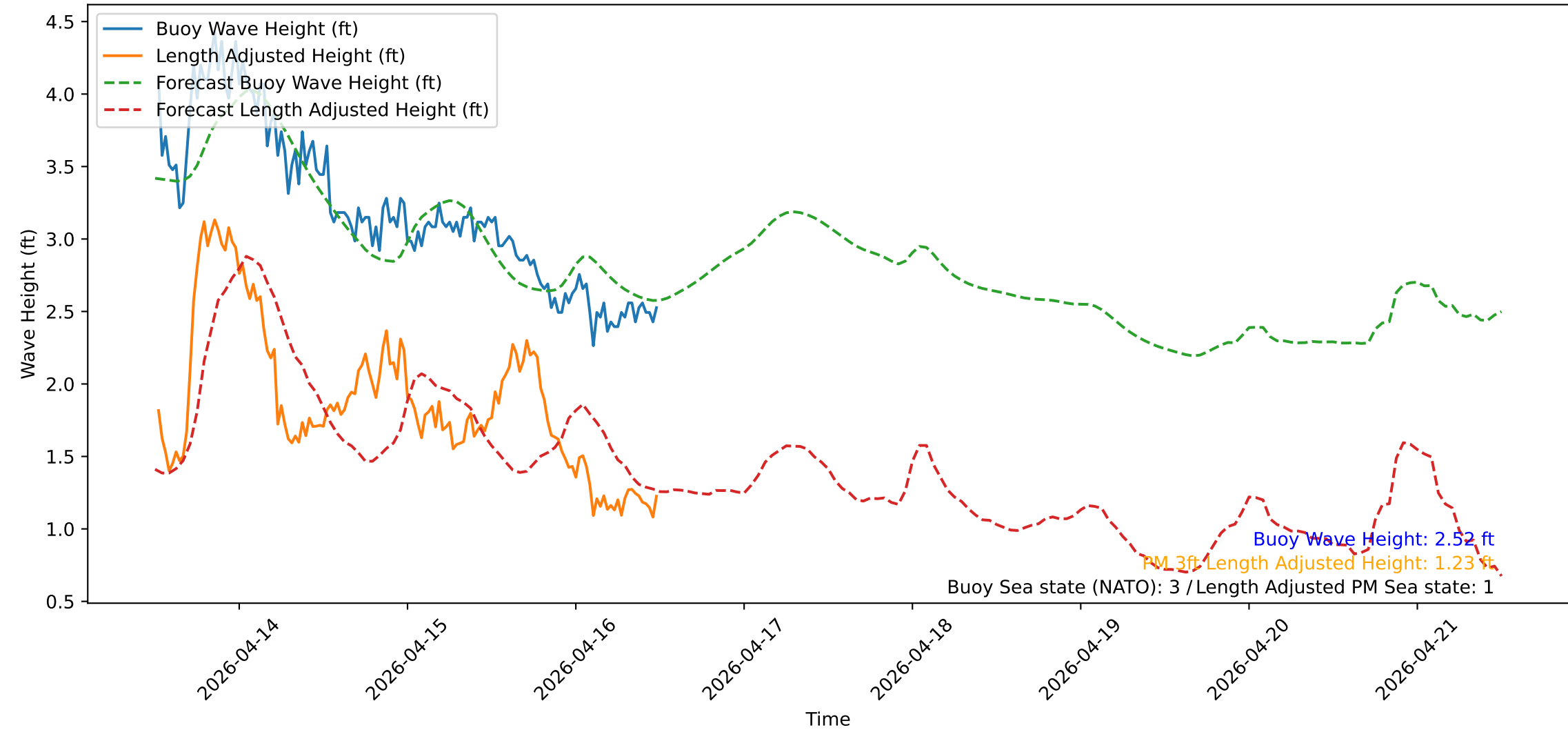
Wave Heights over Time for Red Beach at 2026-04-16 12:10:50
