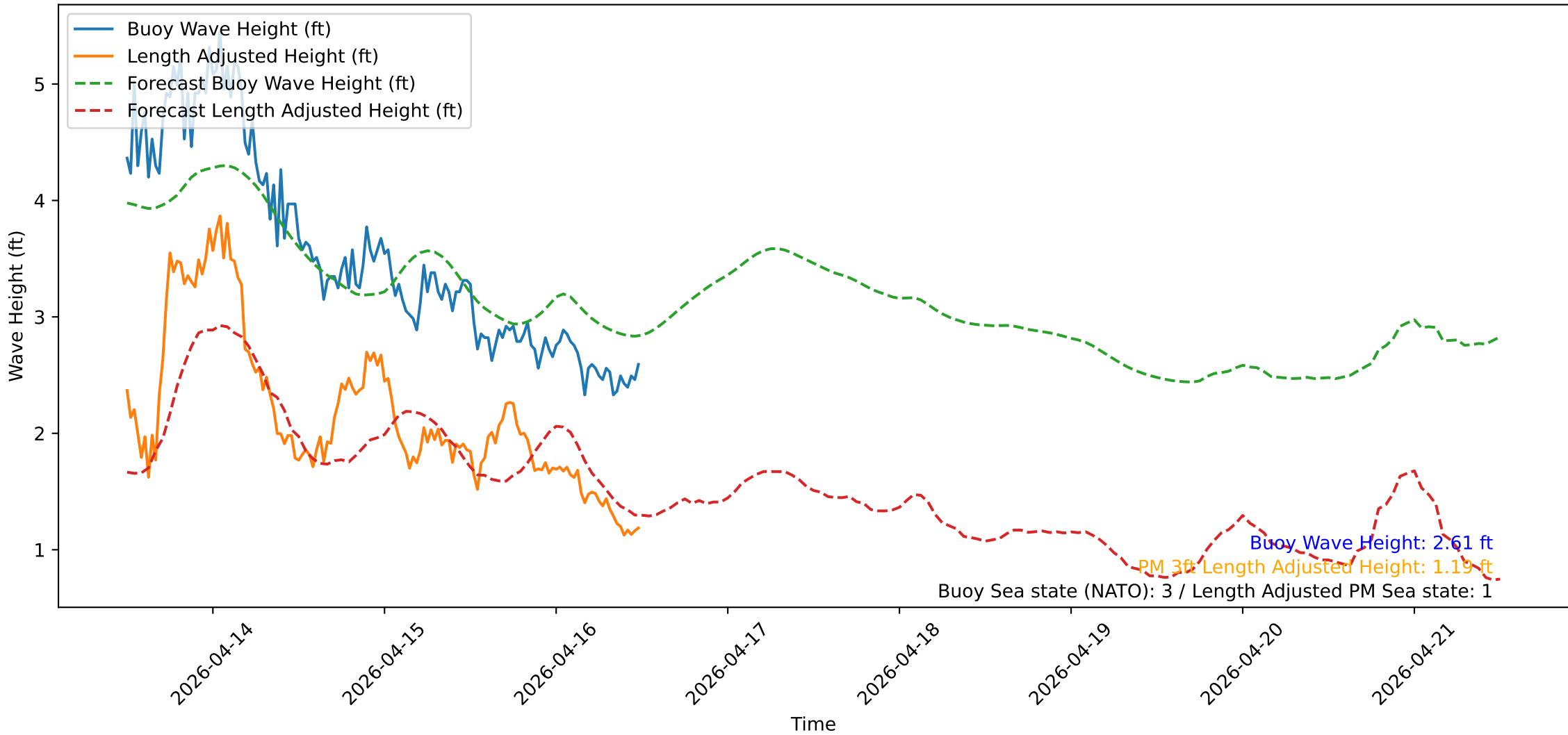
Wave Heights over Time for Oceanside Harbor at 2026-04-16 12:10:31
