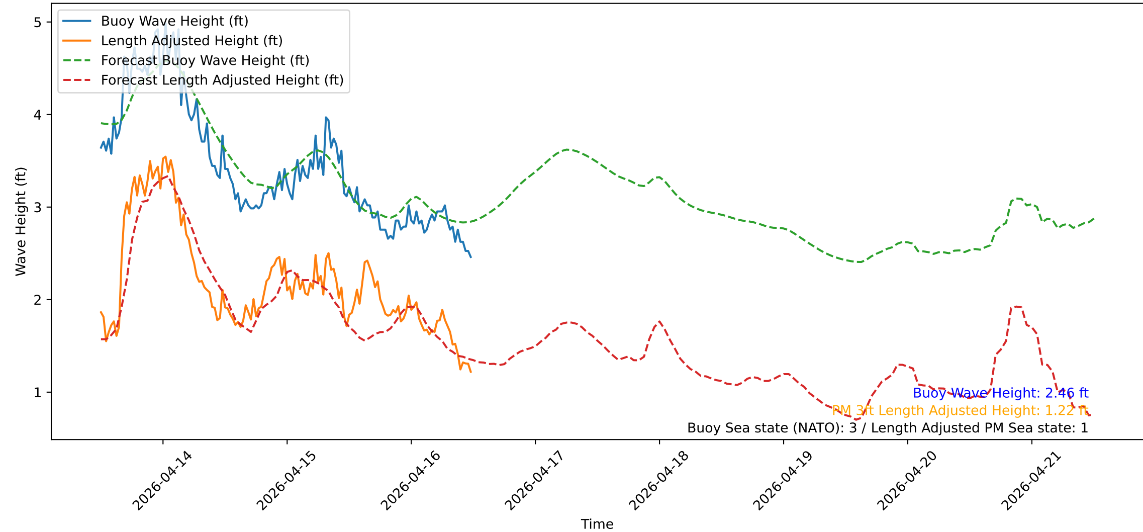
Wave Heights over Time for Green Beach at 2026-04-16 12:11:12
