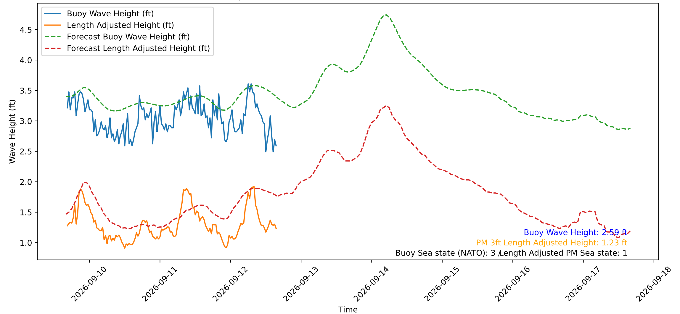
Wave Heights over Time for Green Beach at 2026-09-12 16:11:11
