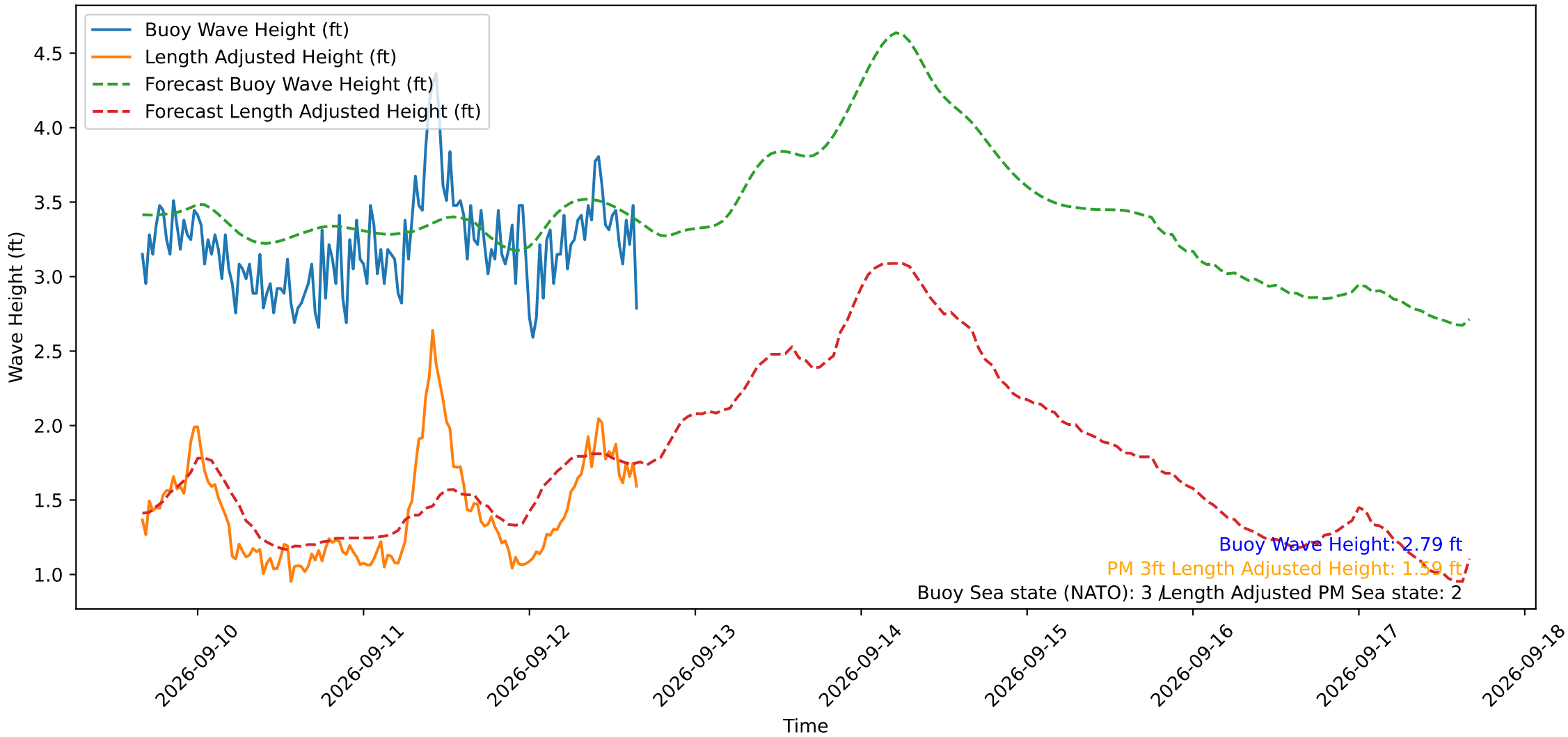
Wave Heights over Time for Oceanside Harbor at 2026-09-12 16:10:29
