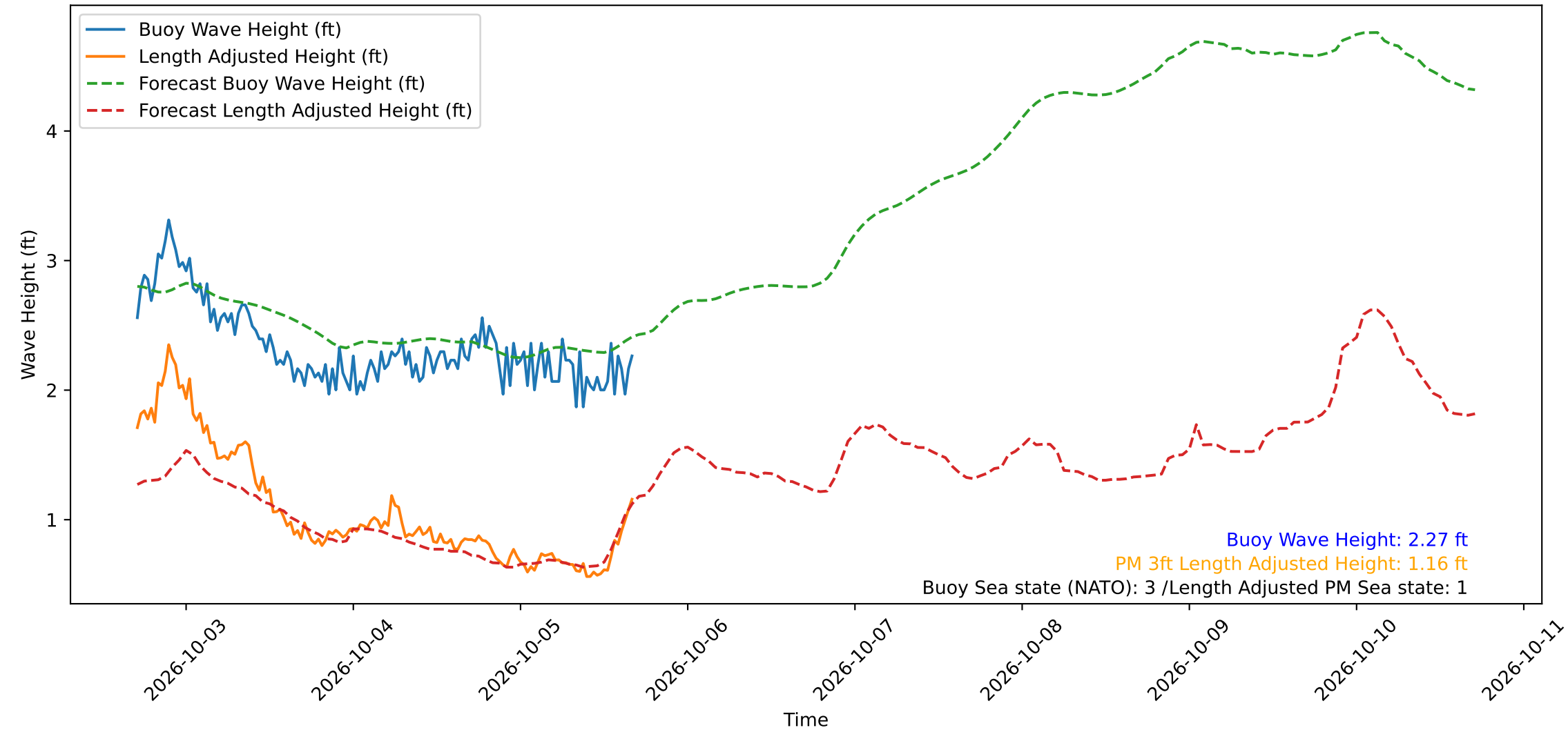
Wave Heights over Time for Oceanside Harbor at 2026-10-05 16:50:30
