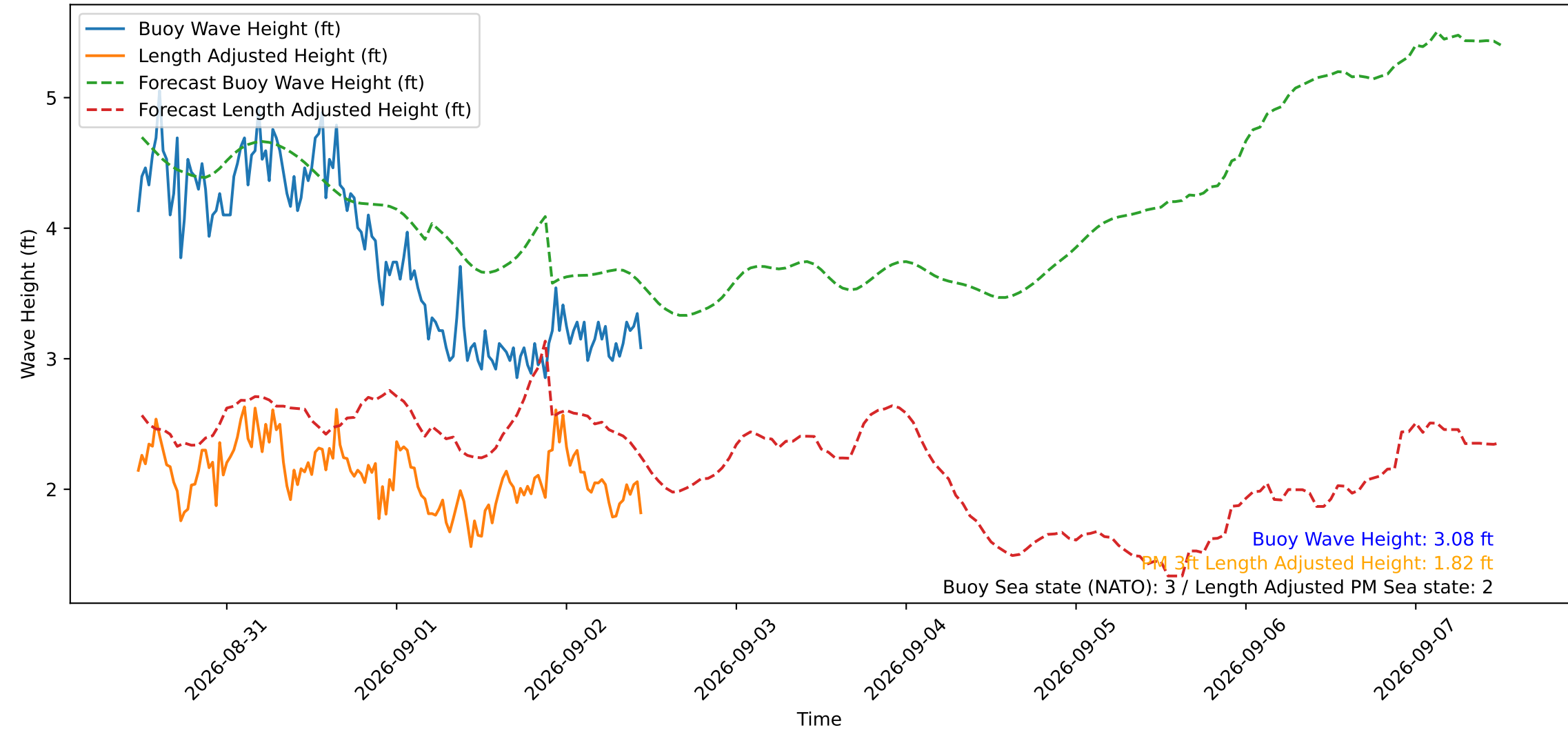
Wave Heights over Time for Oceanside Harbor at 2026-09-02 11:30:30
