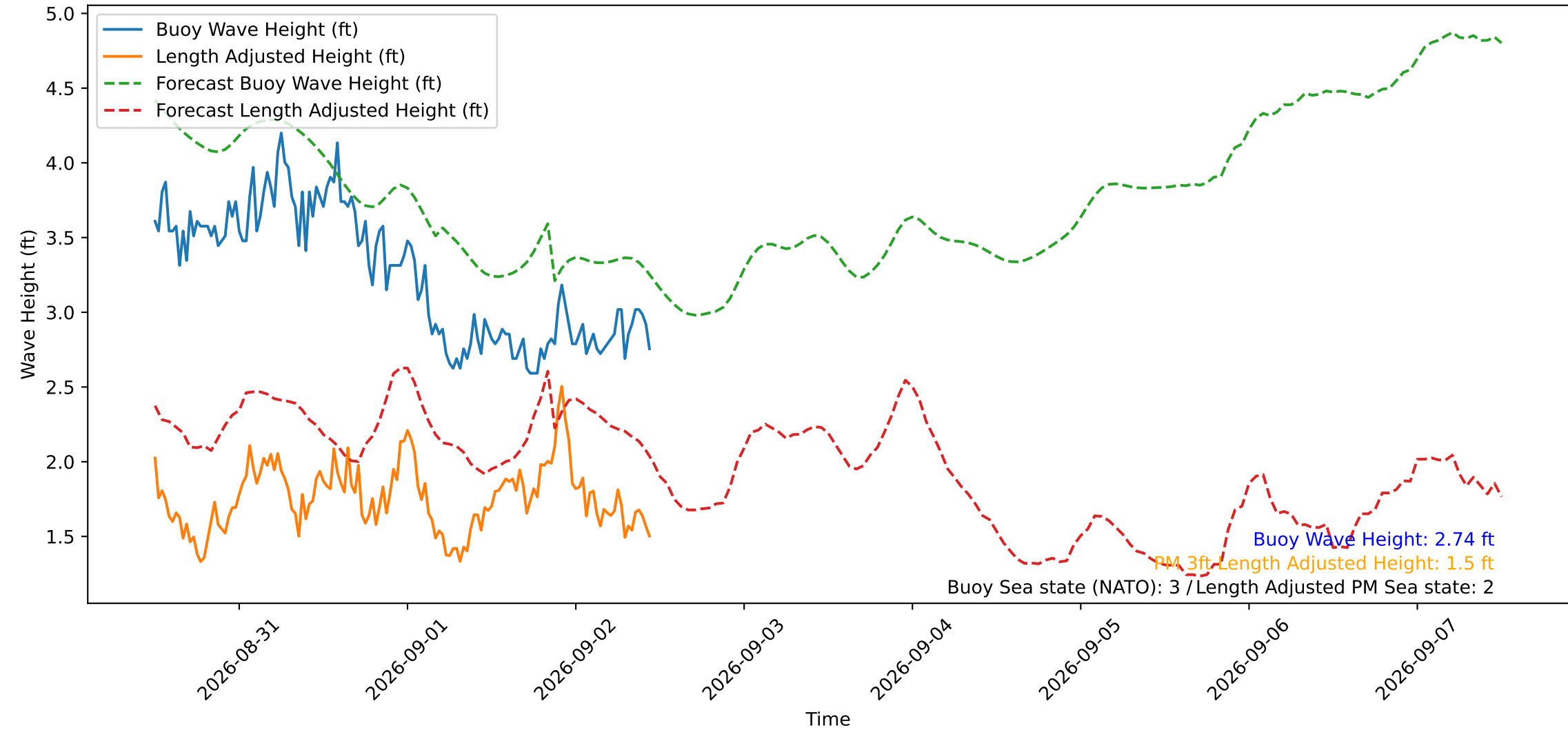
Wave Heights over Time for Red Beach at 2026-09-02 11:30:50
