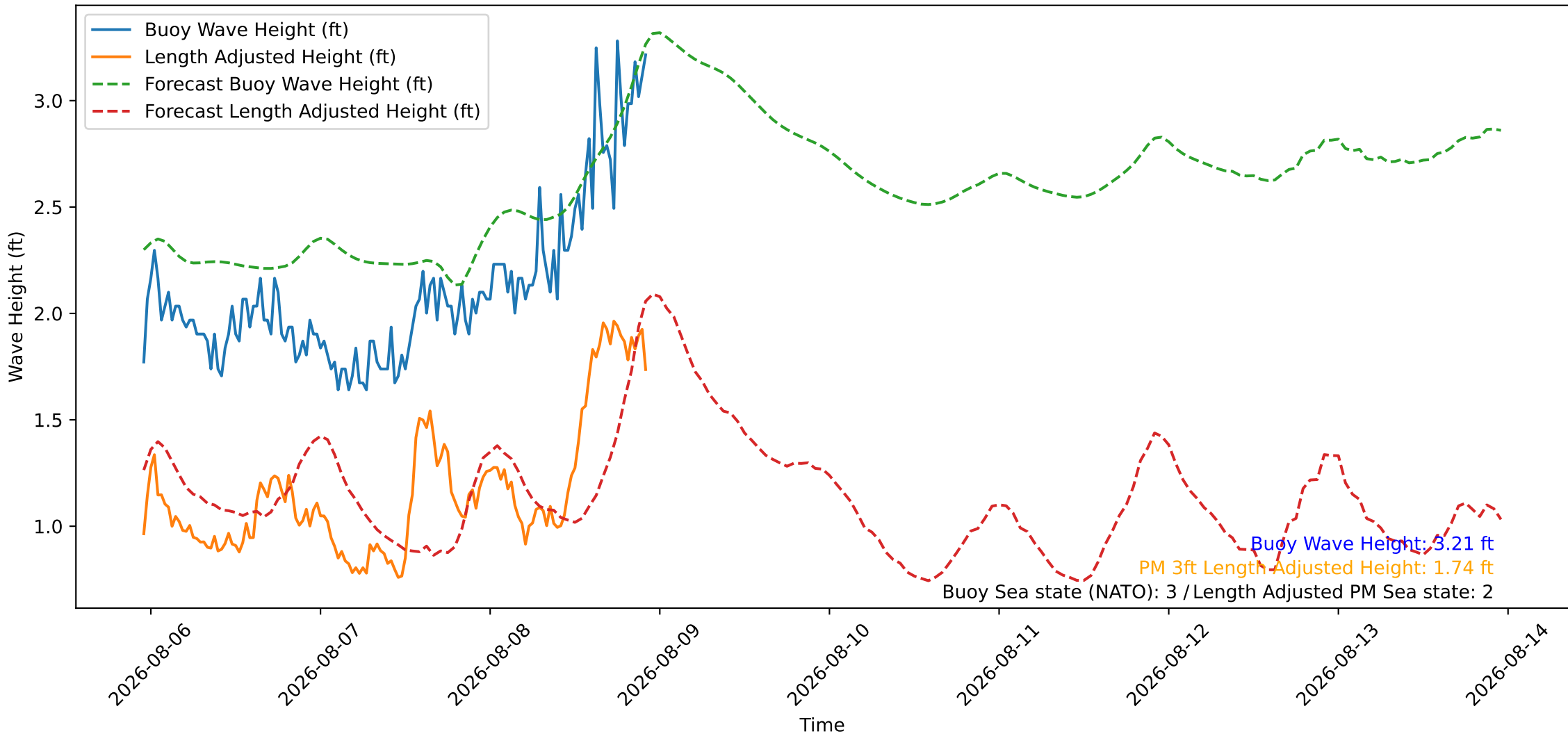
Wave Heights over Time for Oceanside Harbor at 2026-08-08 22:50:26
