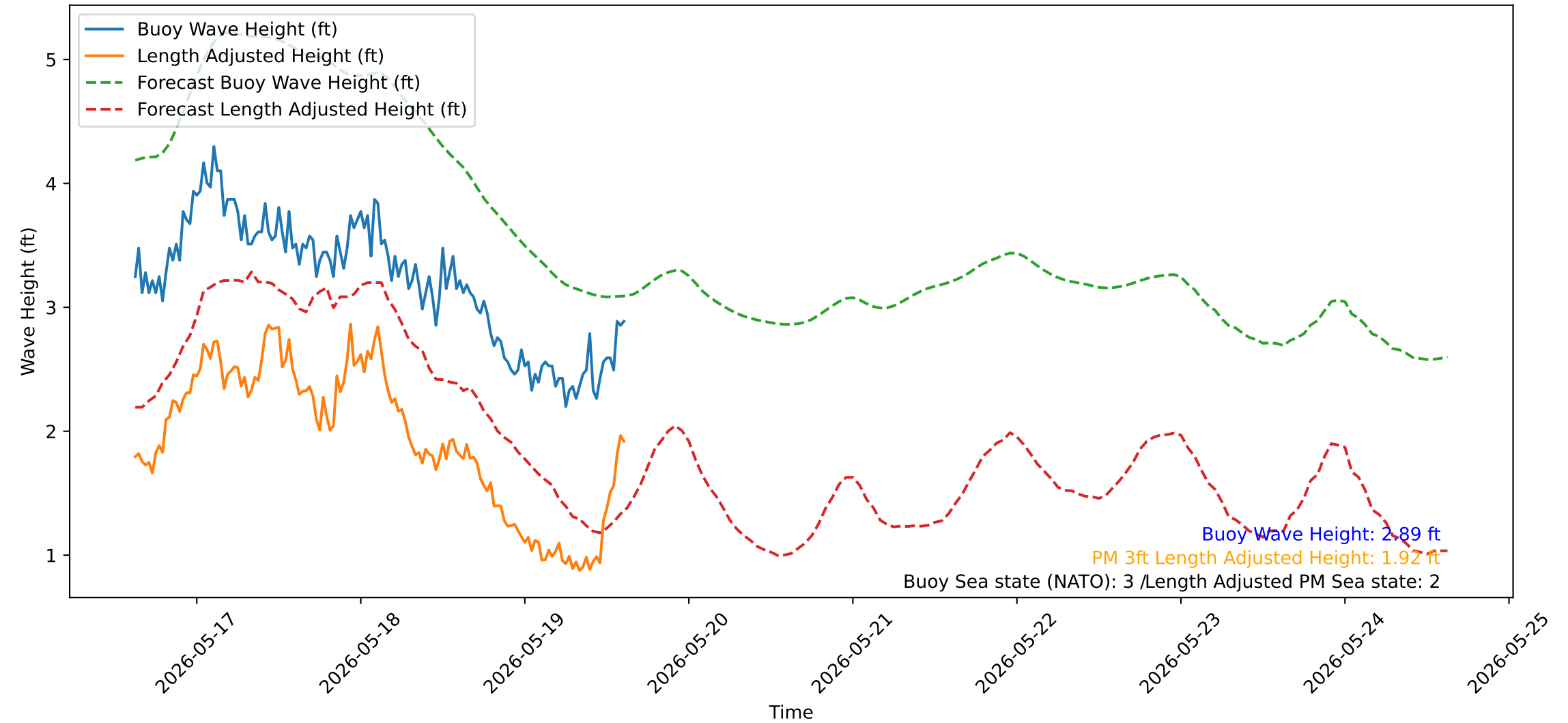
Wave Heights over Time for Oceanside Harbor at 2026-05-19 15:00:31
