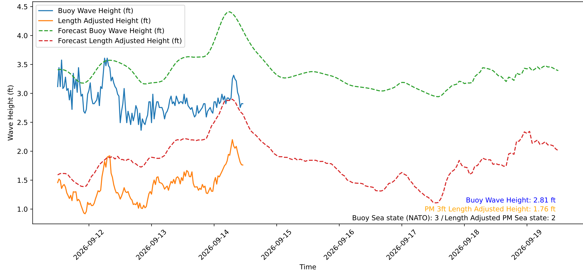
Wave Heights over Time for Green Beach at 2026-09-14 11:41:12
