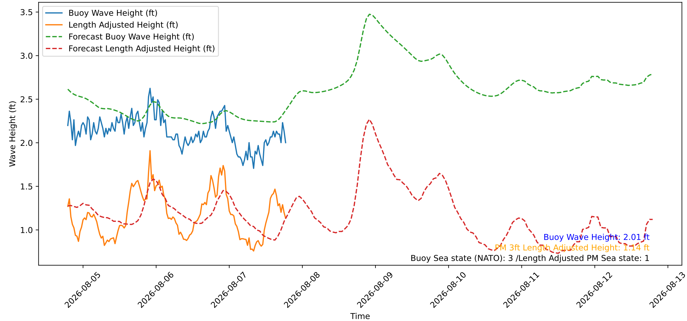
Wave Heights over Time for Green Beach at 2026-08-07 19:11:09
