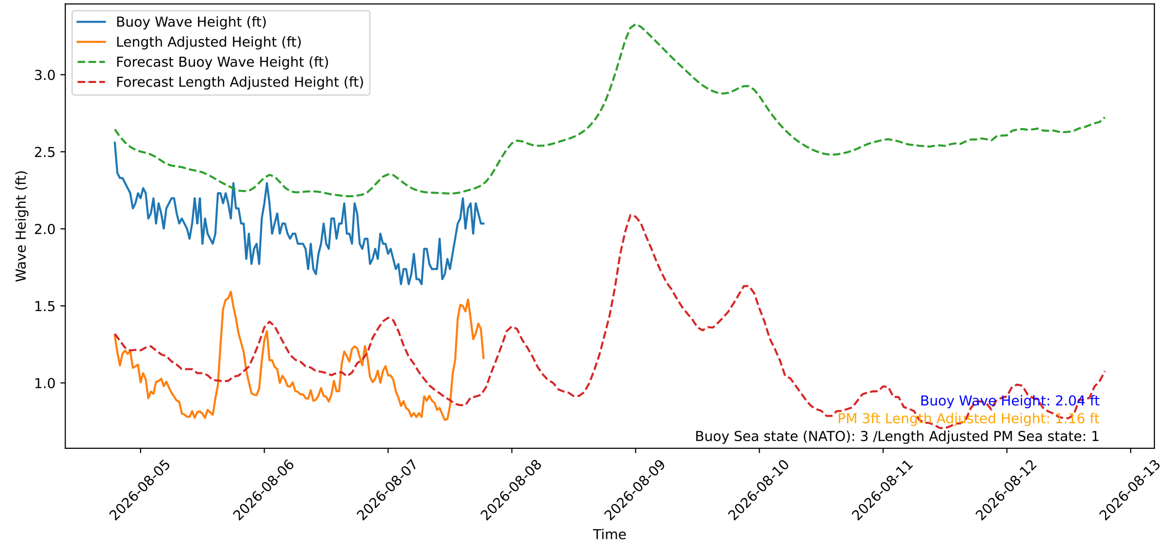
Wave Heights over Time for Oceanside Harbor at 2026-08-07 19:10:26
