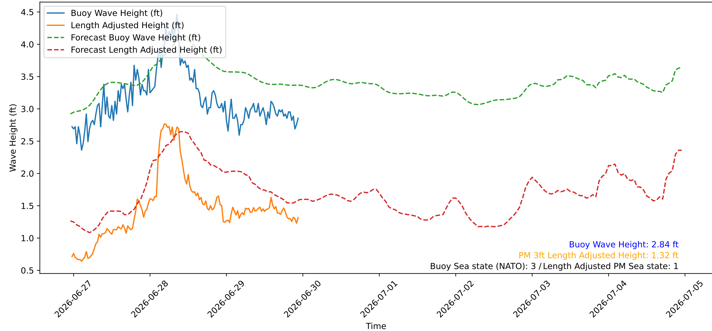
Wave Heights over Time for Red Beach at 2026-06-29 23:10:45
