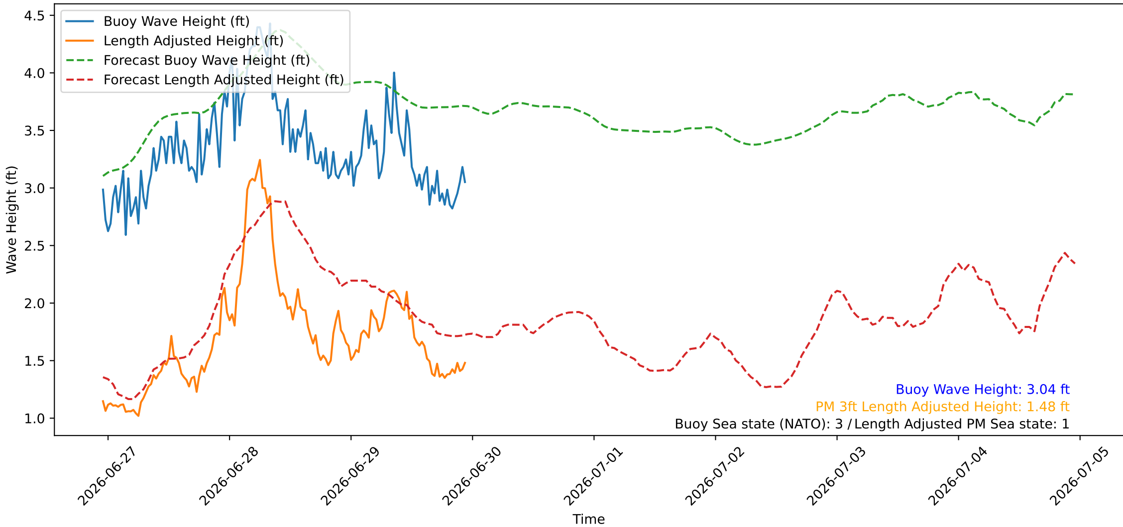
Wave Heights over Time for Oceanside Harbor at 2026-06-29 23:10:26
