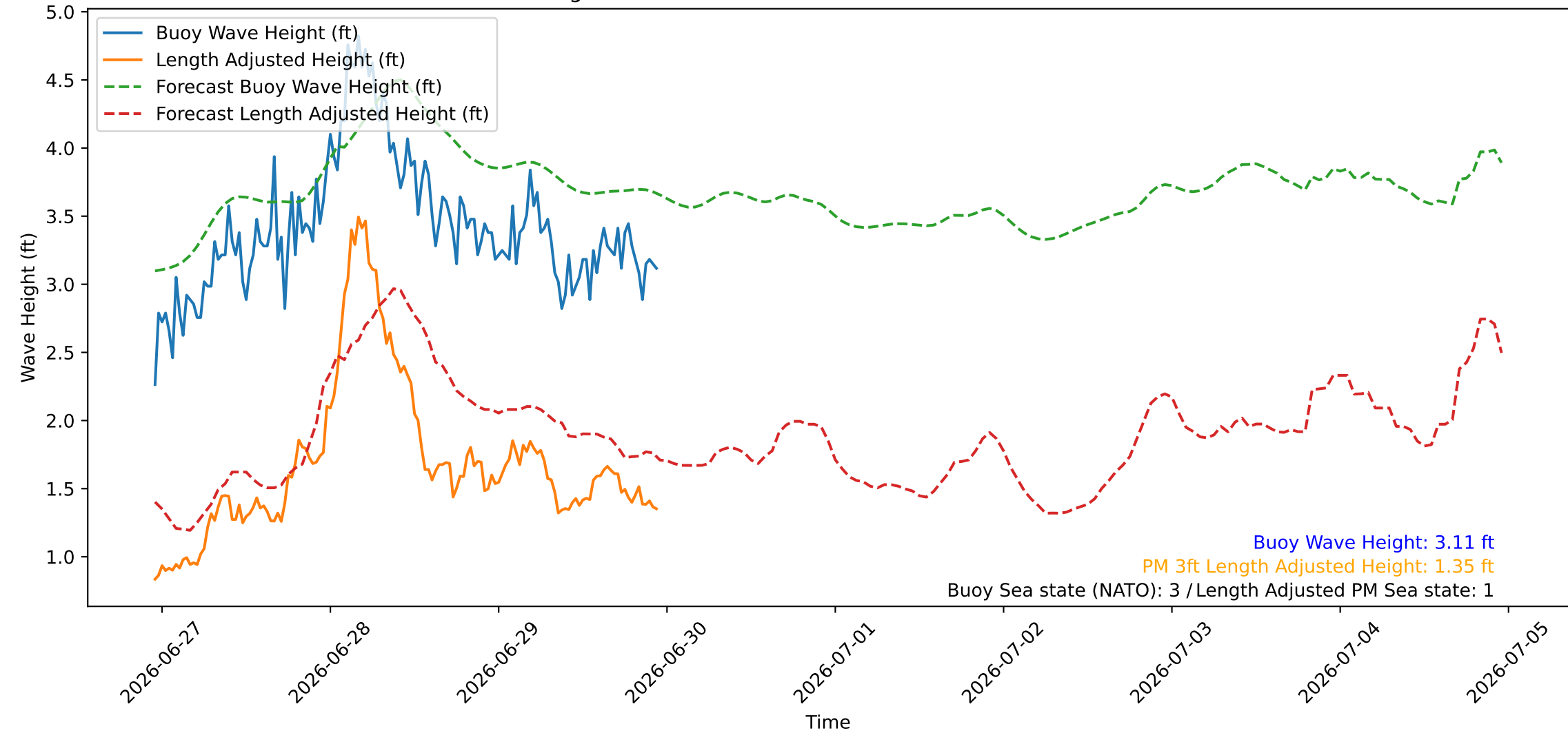
Wave Heights over Time for Green Beach at 2026-06-29 23:11:08
